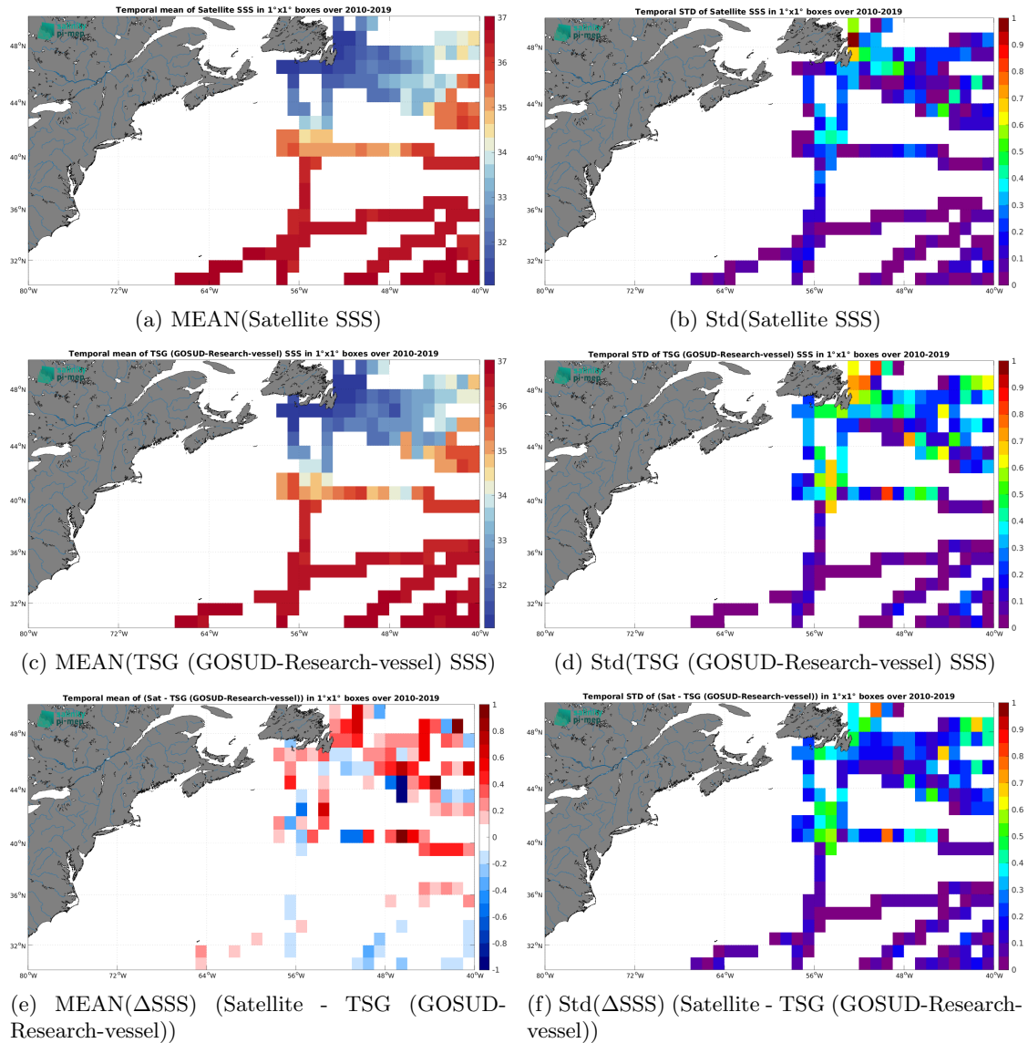
Figure 6: Temporal mean (left) and Std (right) of SSS from SMOS SSS L3 v9 - 18 Days (CATDS-CEC-LOCEAN) (top), TSG (GOSUD-Research-vessel) (middle), and of \Delta SSS (Satellite - TSG (GOSUD-Research-vessel)). Only match-up pairs are used to generate these maps.
