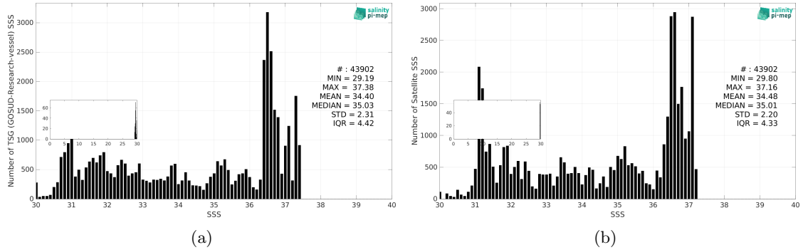
Figure 2: Histograms of SSS from TSG (GOSUD-Research-vessel) (a) and SMOS SSS L3 v9 - 18 Days (CATDS-CEC-LOCEAN) (b) considering all match-up pairs per bins of 0.1 over the Gulf Stream Pi-MEP region and for the full satellite product period.
