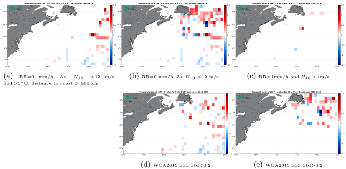
Figure 12: Temporal mean gridded over spatial boxes of size 1^{\circ}\times 1^{\circ} of \Delta SSS (SMOS SSS L3 v9 - 18 Days (CATDS-CEC-LOCEAN) - TSG (GOSUD-Research-vessel)) for 5 different subdatasets corresponding to:RR=0 mm/h, 3 < U_{10} < 12 m/s, SST >5^{\circ}\text{C} , distance to coast > 800 km (a), RR=0 mm/h, 3 < U_{10} < 12 m/s (b), RR >1 mm/h and U_{10} < 4 m/s (c), WOA2013 SSS Std <0.2 (d), WOA2013 SSS Std >0.2 (e).
