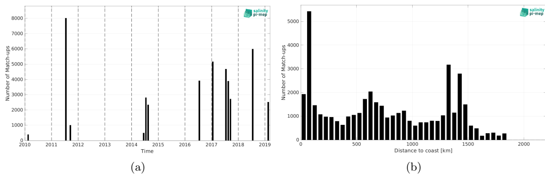
Figure 1: Number of match-ups between TSG (GOSUD-Research-vessel) and SMOS SSS L3 v9 - 18 Days (CATDS-CEC-LOCEAN) SSS as a function of time (a) and as function of the distance to coast (b) over the Gulf Stream Pi-MEP region and for the full satellite product period.
