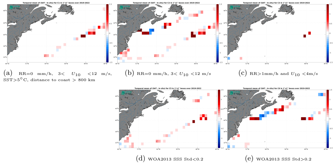
Figure 12: Temporal mean gridded over spatial boxes of size 1^\circ \times 1^\circ of \Delta SSS (SMOS SSS L3 v9 - 18 Days (CATDS-CEC-LOCEAN) - Saildrone) for 5 different subdatasets corresponding to: RR=0 mm/h, 3 < U_{10} < 12 m/s, SST > 5^\circ C , distance to coast > 800 km (a), RR=0 mm/h, 3 < U_{10} < 12 m/s (b), RR > 1 mm/h and U_{10} < 4 m/s (c), WOA2013 SSS Std < 0.2 (d), WOA2013 SSS Std > 0.2 (e).
