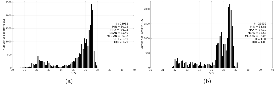
Figure 2: Histograms of SSS from Saildrone (a) and SMOS SSS L3 v9 - 18 Days (CATDS-CEC-LOCEAN) (b) considering all match-up pairs per bins of 0.1 over the Gulf Stream Pi-MEP region and for the full satellite product period.
