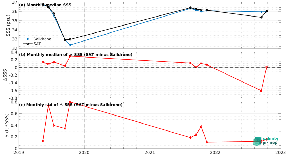
Figure 7: Time series of the monthly median SSS (top), median of \Delta\text{SSS} (Satellite - Saildrone) and Std of \Delta\text{SSS} (Satellite - Saildrone) over the Gulf Stream Pi-MEP region considering all match-ups collected by the Pi-MEP.
