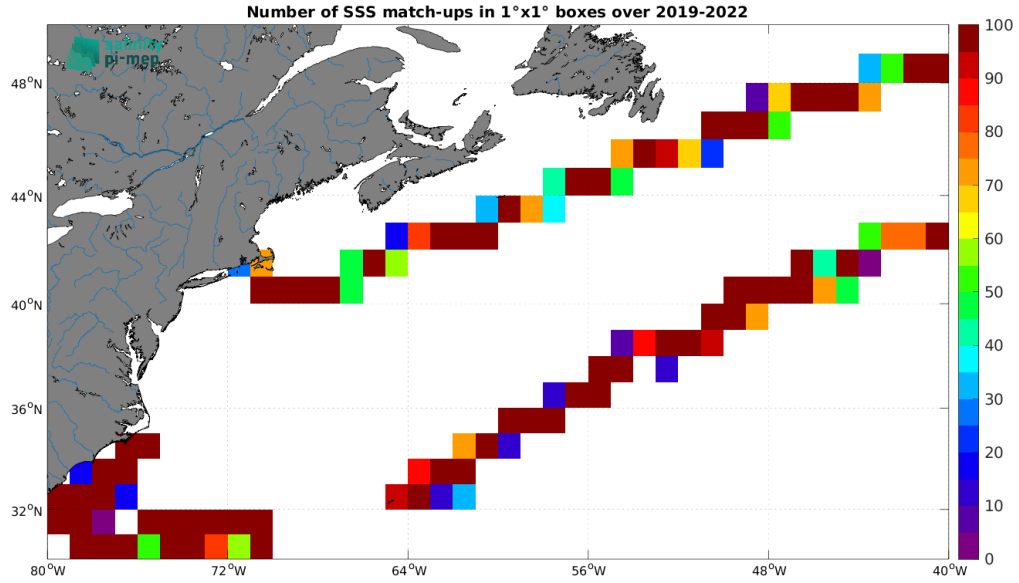
Figure 4: Number of SSS match-ups between Saildrone SSS and the SMOS SSS L3 v9 - 18 Days (CATDS-CEC-LOCEAN) SSS product for the Gulf Stream Pi-MEP region over 1^\circ \times 1^\circ boxes and for the full satellite product period.
