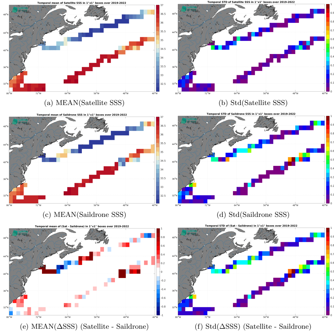
Figure 6: Temporal mean (left) and Std (right) of SSS from SMOS SSS L3 v9 - 18 Days (CATDS-CEC-LOCEAN) (top), Saildrone (middle), and of \Delta SSS (Satellite - Saildrone). Only match-up pairs are used to generate these maps.
