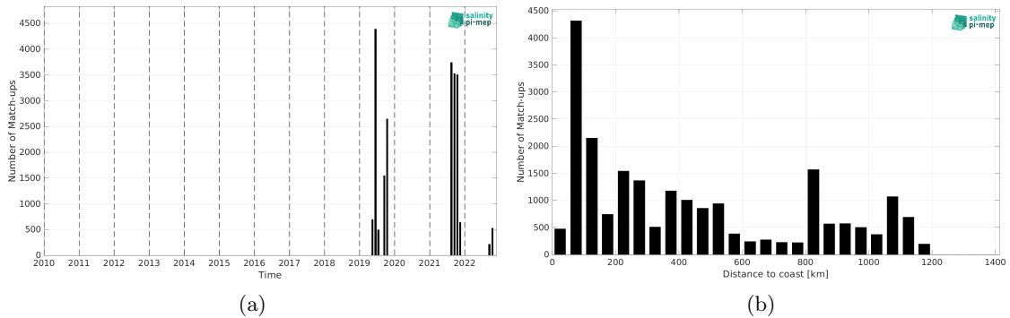
Figure 1: Number of match-ups between Saildrone and SMOS SSS L3 v9 - 18 Days (CATDS-CEC-LOCEAN) SSS as a function of time (a) and as function of the distance to coast (b) over the Gulf Stream Pi-MEP region and for the full satellite product period.
