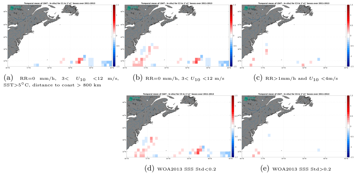
Figure 11: Temporal mean gridded over spatial boxes of size 1^{\circ}\times 1^{\circ} of \Delta\text{SSS} (SMOS SSS L3 v9 - 18 Days (CATDS-CEC-LOCEAN) - Surface drifters) for 5 different subdatasets corresponding to:RR=0 mm/h, 3 < U_{10} < 12 m/s, SST >5^{\circ}\text{C} , distance to coast > 800 km (a), RR=0 mm/h, 3 < U_{10} < 12 m/s (b), RR >1 mm/h and U_{10} < 4 m/s (c), WOA2013 SSS Std <0.2 (d), WOA2013 SSS Std >0.2 (e).
