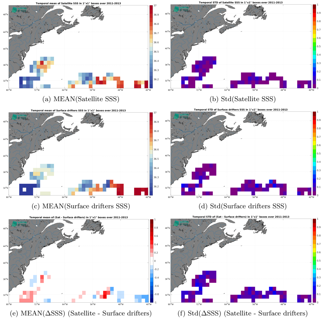
Figure 5: Temporal mean (left) and Std (right) of SSS from SMOS SSS L3 v9 - 18 Days (CATDS-CEC-LOCEAN) (top), Surface drifters (middle), and of \Delta SSS (Satellite - Surface drifters). Only match-up pairs are used to generate these maps.
