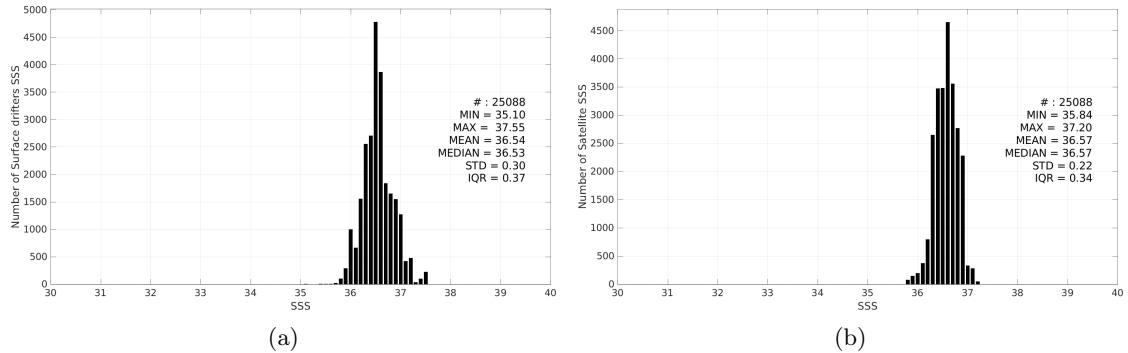
Figure 2: Histograms of SSS from Surface drifters (a) and SMOS SSS L3 v9 - 18 Days (CATDS-CEC-LOCEAN) (b) considering all match-up pairs per bins of 0.1 over the Gulf Stream Pi-MEP region and for the full satellite product period.
