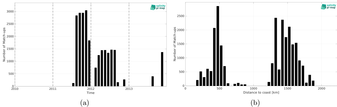
Figure 1: Number of match-ups between Surface drifters and SMOS SSS L3 v9 - 18 Days (CATDS-CEC-LOCEAN) SSS as a function of time (a) and as function of the distance to coast (b) over the Gulf Stream Pi-MEP region and for the full satellite product period.
