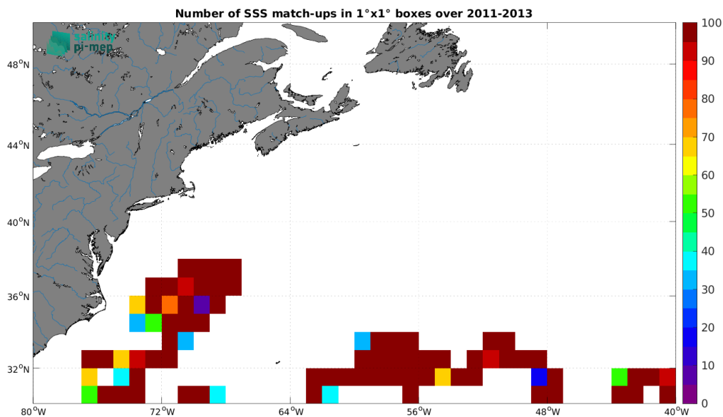
Figure 3: Number of SSS match-ups between Surface drifters SSS and the SMOS SSS L3 v9 - 18 Days (CATDS-CEC-LOCEAN) SSS product for the Gulf Stream Pi-MEP region over 1^\circ \times 1^\circ boxes and for the full satellite product period.
