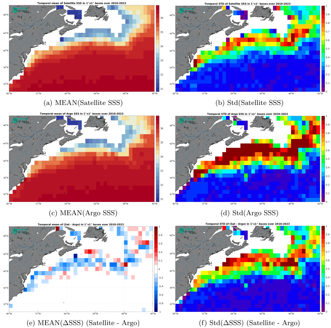
Figure 6: Temporal mean (left) and Std (right) of SSS from SMOS SSS L3 v9 - 18 Days (CATDS-CEC-LOCEAN) (top), Argo (middle), and of \Delta SSS (Satellite - Argo). Only match-up pairs are used to generate these maps.
