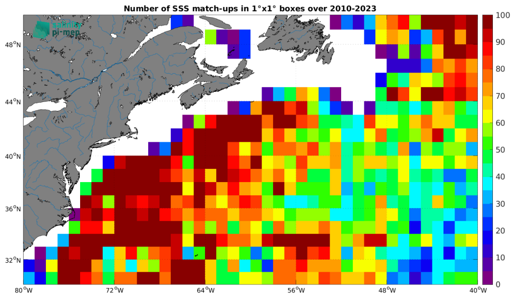
Figure 4: Number of SSS match-ups between Argo SSS and the SMOS SSS L3 v9 - 18 Days (CATDS-CEC-LOCEAN) SSS product for the Gulf Stream Pi-MEP region over 1^\circ \times 1^\circ boxes and for the full satellite product period.
