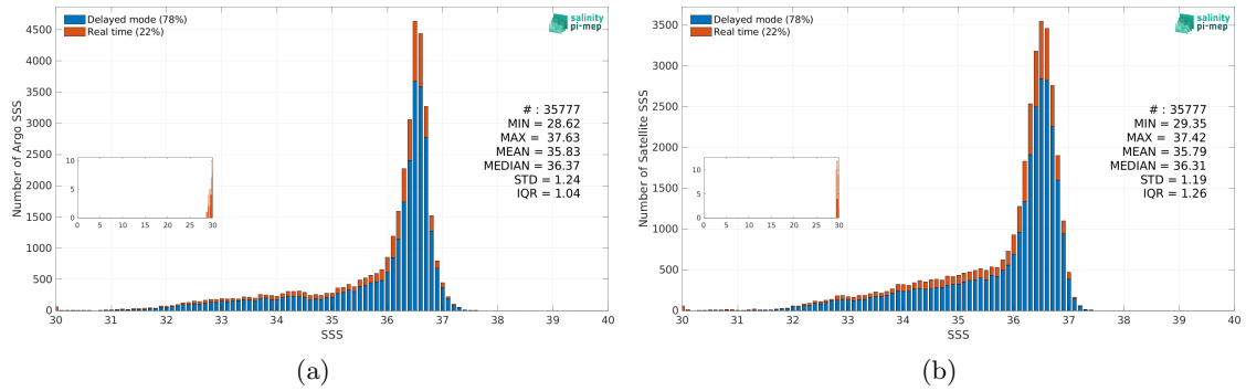
Figure 2: Histograms of SSS from Argo (a) and SMOS SSS L3 v9 - 18 Days (CATDS-CEC-LOCEAN) (b) considering all match-up pairs per bins of 0.1 over the Gulf Stream Pi-MEP region and for the full satellite product period.
