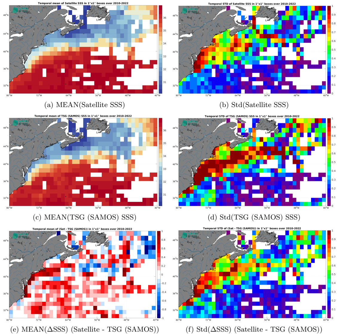
Figure 6: Temporal mean (left) and Std (right) of SSS from SMOS SSS L3 v8 - 9 Days (CATDS-CEC-LOCEAN) (top), TSG (SAMOS) (middle), and of \Delta SSS (Satellite - TSG (SAMOS)). Only match-up pairs are used to generate these maps.
