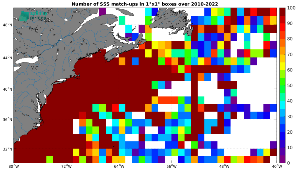
Figure 4: Number of SSS match-ups between TSG (SAMOS) SSS and the SMOS SSS L3 v8 - 9 Days (CATDS-CEC-LOCEAN) SSS product for the Gulf Stream Pi-MEP region over 1^\circ \times 1^\circ boxes and for the full satellite product period.
