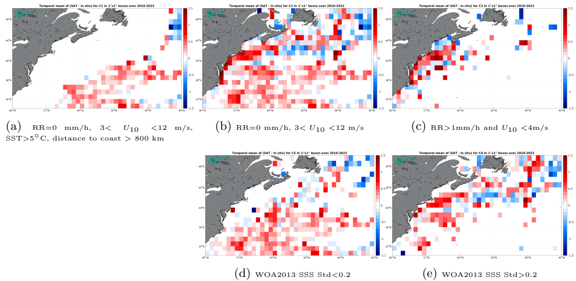
Figure 12: Temporal mean gridded over spatial boxes of size 1^\circ \times 1^\circ of \Delta SSS (SMOS SSS L3 v8 - 9 Days (CATDS-CEC-LOCEAN) - TSG (SAMOS)) for 5 different subdatasets corresponding to:RR=0 mm/h, 3 < U_{10} < 12 m/s, SST >5^\circ\text{C} , distance to coast > 800 km (a), RR=0 mm/h, 3 < U_{10} < 12 m/s (b), RR >1 mm/h and U_{10} < 4 m/s (c), WOA2013 SSS Std <0.2 (d), WOA2013 SSS Std >0.2 (e).
