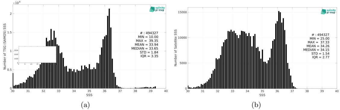
Figure 2: Histograms of SSS from TSG (SAMOS) (a) and SMOS SSS L3 v8 - 9 Days (CATDS-CEC-LOCEAN) (b) considering all match-up pairs per bins of 0.1 over the Gulf Stream Pi-MEP region and for the full satellite product period.
