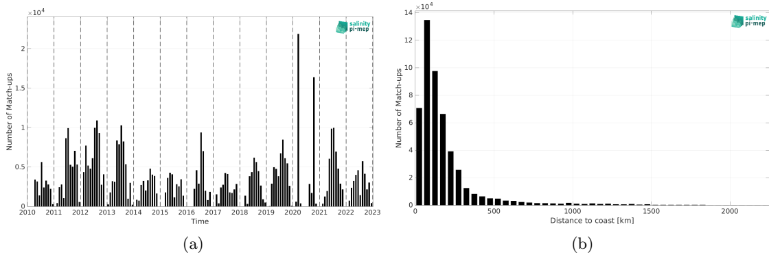
Figure 1: Number of match-ups between TSG (SAMOS) and SMOS SSS L3 v8 - 9 Days (CATDS-CEC-LOCEAN) SSS as a function of time (a) and as function of the distance to coast (b) over the Gulf Stream Pi-MEP region and for the full satellite product period.
