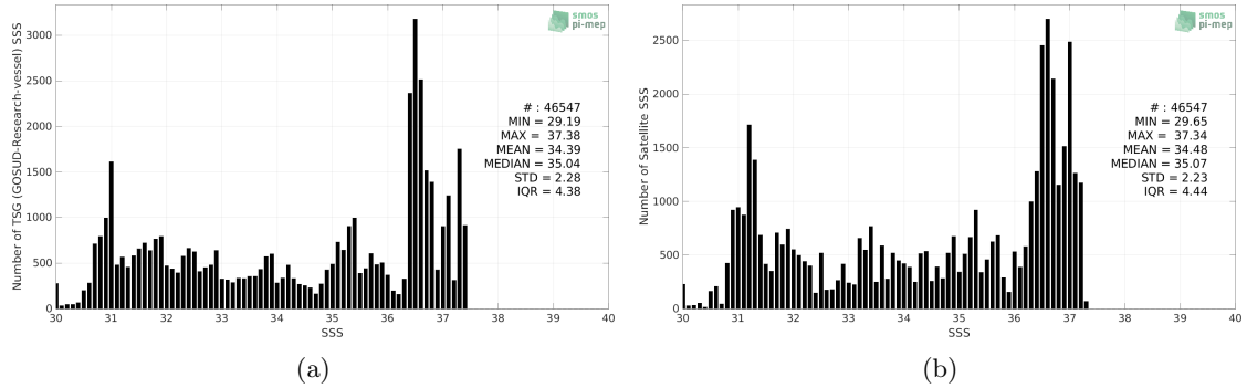
Figure 2: Histograms of SSS from TSG (GOSUD-Research-vessel) (a) and SMOS SSS L3 v8 - 9 Days (CATDS-CECOS-LOCEAN) (b) considering all match-up pairs per bins of 0.1 over the Gulf Stream Pi-MEP region and for the full satellite product period.
