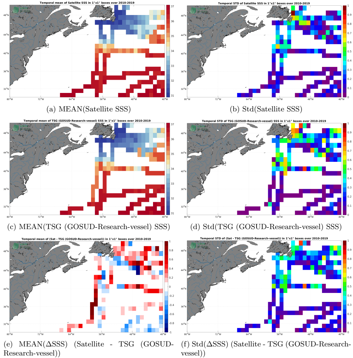
Figure 6: Temporal mean (left) and Std (right) of SSS from SMOS SSS L3 v8 - 9 Days (CATDS-CECOS-LOCEAN) (top), TSG (GOSUD-Research-vessel) (middle), and of \Delta SSS (Satellite - TSG (GOSUD-Research-vessel)). Only match-up pairs are used to generate these maps.
