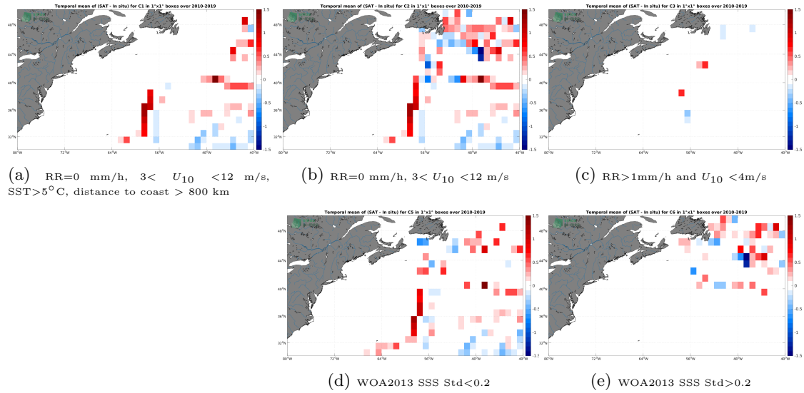
Figure 12: Temporal mean gridded over spatial boxes of size 1^\circ \times 1^\circ of \Delta SSS (SMOS SSS L3 v8 - 9 Days (CATDS-CECOS-LOCEAN) - TSG (GOSUD-Research-vessel)) for 5 different subdatasets corresponding to: RR=0 mm/h, 3 < U_{10} < 12 m/s, SST > 5^\circ\text{C} , distance to coast > 800 km (a), RR=0 mm/h, 3 < U_{10} < 12 m/s (b), RR > 1 mm/h and U_{10} < 4 m/s (c), WOA2013 SSS Std < 0.2 (d), WOA2013 SSS Std > 0.2 (e).
