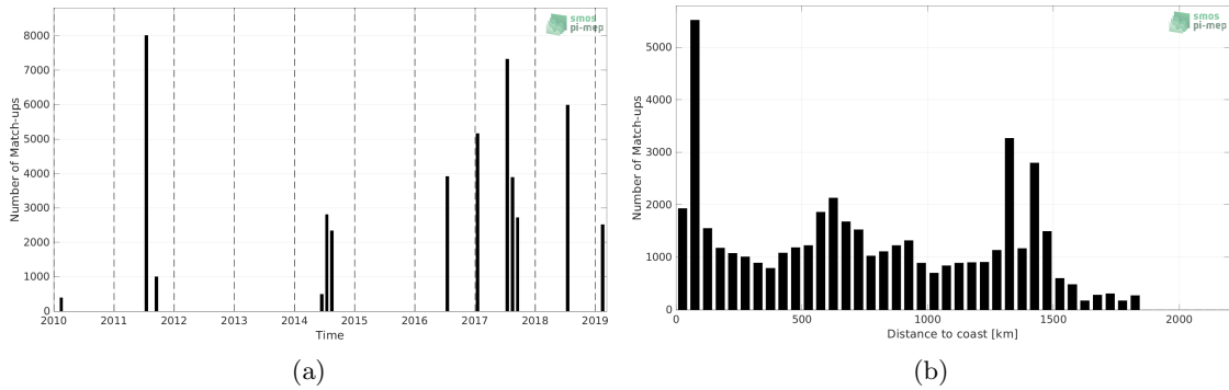
Figure 1: Number of match-ups between TSG (GOSUD-Research-vessel) and SMOS SSS L3 v8 - 9 Days (CATDS-CECOS-LOCEAN) SSS as a function of time (a) and as function of the distance to coast (b) over the Gulf Stream Pi-MEP region and for the full satellite product period.
