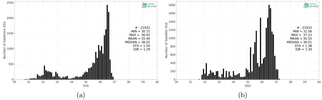
Figure 2: Histograms of SSS from Saildrone (a) and SMOS SSS L3 v8 - 9 Days (CATDS-CECOS-LOCEAN) (b) considering all match-up pairs per bins of 0.1 over the Gulf Stream Pi-MEP region and for the full satellite product period.
