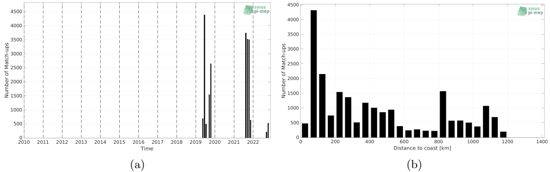
Figure 1: Number of match-ups between Saildrone and SMOS SSS L3 v8 - 9 Days (CATDS-CECOS-LOCEAN) SSS as a function of time (a) and as function of the distance to coast (b) over the Gulf Stream Pi-MEP region and for the full satellite product period.
