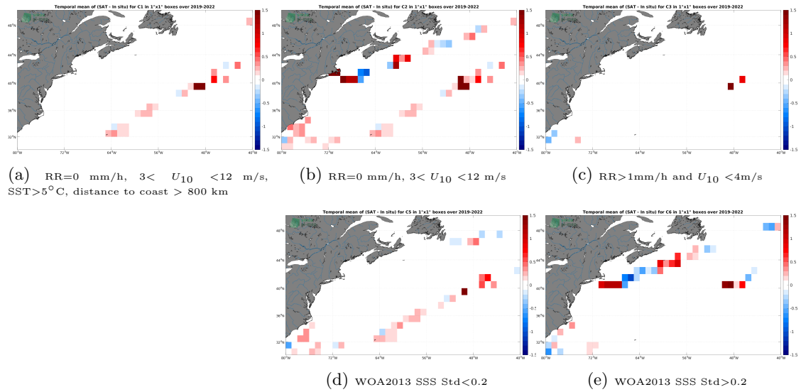
Figure 12: Temporal mean gridded over spatial boxes of size 1^\circ \times 1^\circ of \Delta SSS (SMOS SSS L3 v8 - 9 Days (CATDS-CECOS-LOCEAN) - Saildrone) for 5 different subdatasets corresponding to:RR=0 mm/h, 3 < U_{10} < 12 m/s, SST >5^\circ C, distance to coast > 800 km (a), RR=0 mm/h, 3 < U_{10} < 12 m/s (b), RR >1 mm/h and U_{10} < 4 m/s (c), WOA2013 SSS Std <0.2 (d), WOA2013 SSS Std >0.2 (e).
