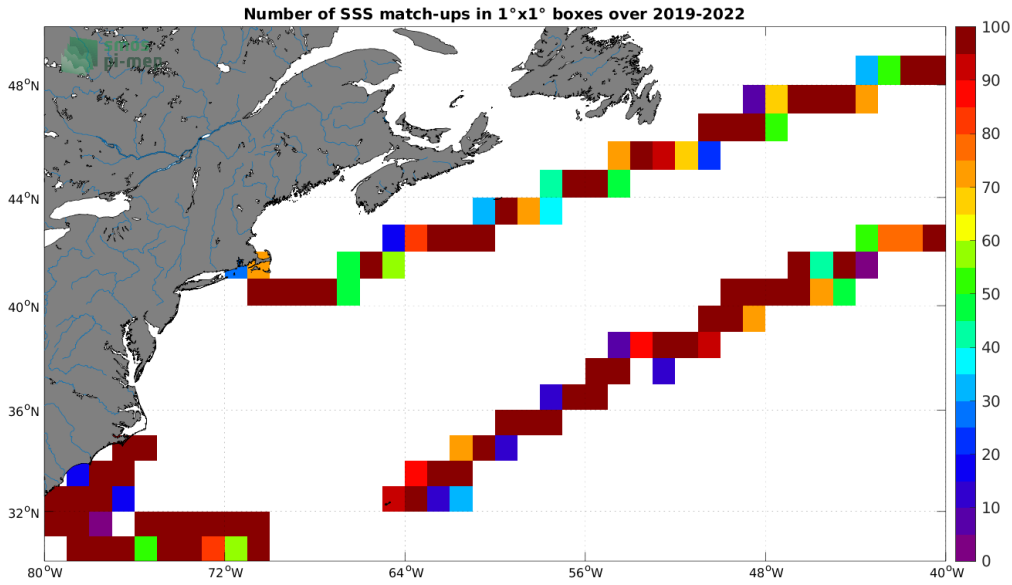
Figure 4: Number of SSS match-ups between Saildrone SSS and the SMOS SSS L3 v8 - 9 Days (CATDS-CECOS-LOCEAN) SSS product for the Gulf Stream Pi-MEP region over 1^\circ \times 1^\circ boxes and for the full satellite product period.
