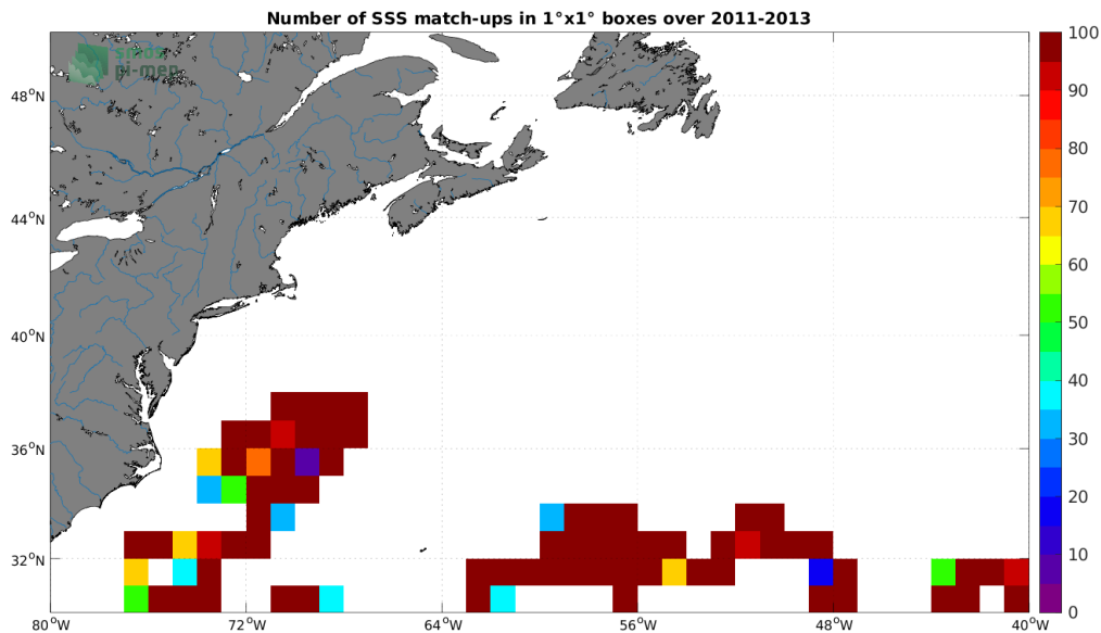
Figure 3: Number of SSS match-ups between Surface drifters SSS and the SMOS SSS L3 v8 - 9 Days (CATDS-CECOS-LOCEAN) SSS product for the Gulf Stream Pi-MEP region over 1^\circ \times 1^\circ boxes and for the full satellite product period.
