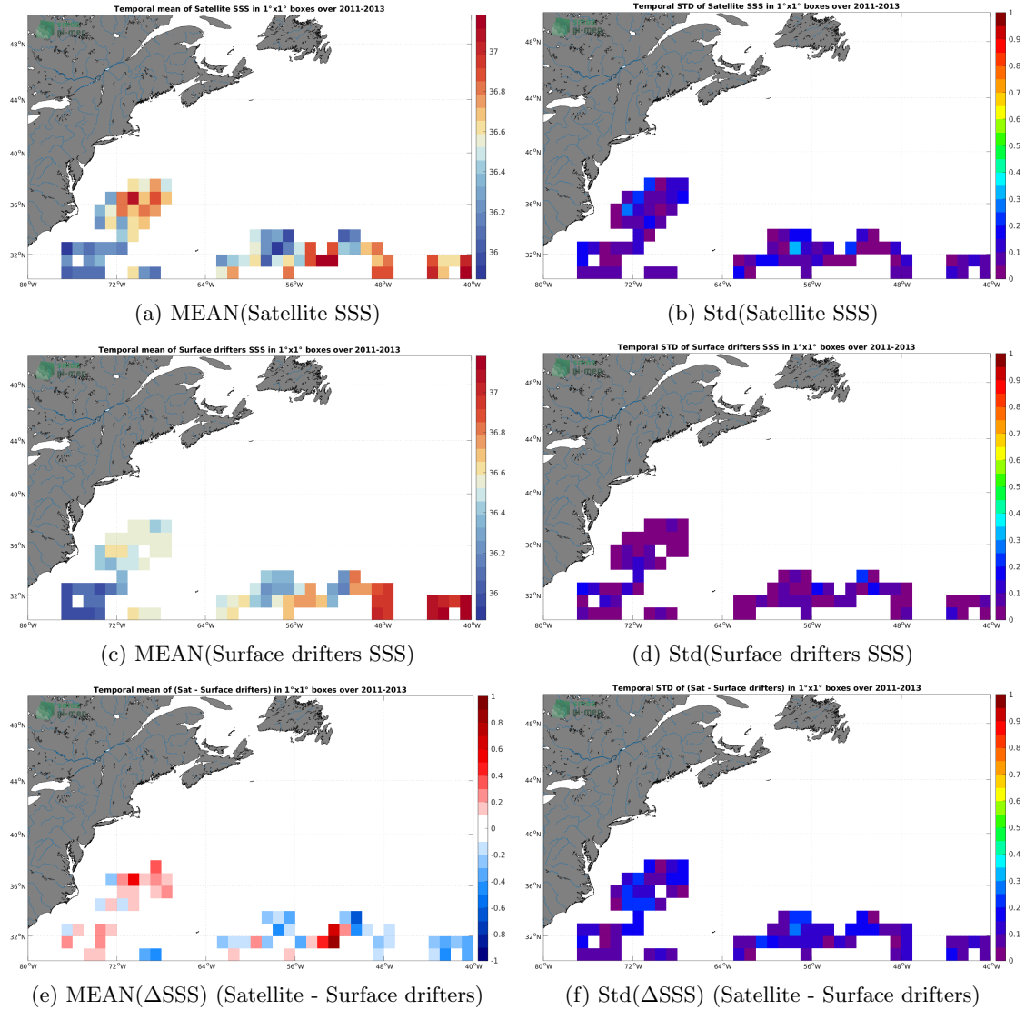
Figure 5: Temporal mean (left) and Std (right) of SSS from SMOS SSS L3 v8 - 9 Days (CATDS-CECOS-LOCEAN) (top), Surface drifters (middle), and of \Delta SSS (Satellite - Surface drifters). Only match-up pairs are used to generate these maps.
