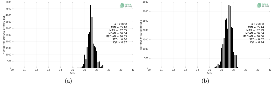
Figure 2: Histograms of SSS from Surface drifters (a) and SMOS SSS L3 v8 - 9 Days (CATDS-CECOS-LOCEAN) (b) considering all match-up pairs per bins of 0.1 over the Gulf Stream Pi-MEP region and for the full satellite product period.
