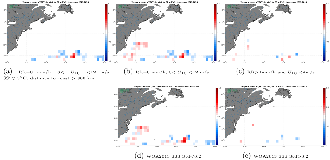
Figure 11: Temporal mean gridded over spatial boxes of size 1^{\circ}\times 1^{\circ} of \Delta\text{SSS} (SMOS SSS L3 v8 - 9 Days (CATDS-CECOS-LOCEAN) - Surface drifters) for 5 different subdatasets corresponding to:RR=0 mm/h, 3 < U_{10} < 12 m/s, SST >5^{\circ}\text{C} , distance to coast > 800 km (a), RR=0 mm/h, 3 < U_{10} < 12 m/s (b), RR >1 mm/h and U_{10} < 4 m/s (c), WOA2013 SSS Std <0.2 (d), WOA2013 SSS Std >0.2 (e).
