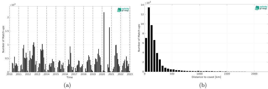
Figure 1: Number of match-ups between TSG (SAMOS) and SMOS SSS L3 v8 - 18 Days (CATDS-CEC-LOCEAN) SSS as a function of time (a) and as function of the distance to coast (b) over the Gulf Stream Pi-MEP region and for the full satellite product period.
