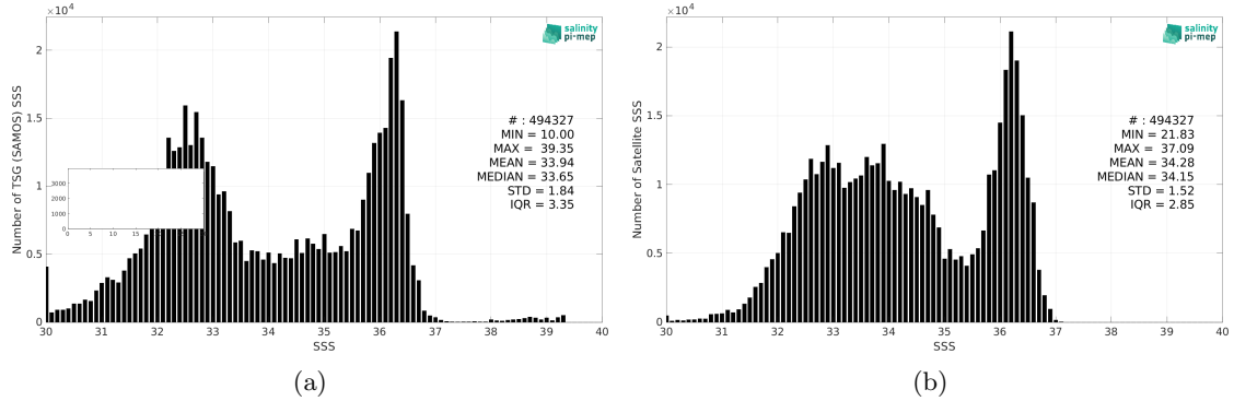
Figure 2: Histograms of SSS from TSG (SAMOS) (a) and SMOS SSS L3 v8 - 18 Days (CATDS-CEC-LOCEAN) (b) considering all match-up pairs per bins of 0.1 over the Gulf Stream Pi-MEP region and for the full satellite product period.
