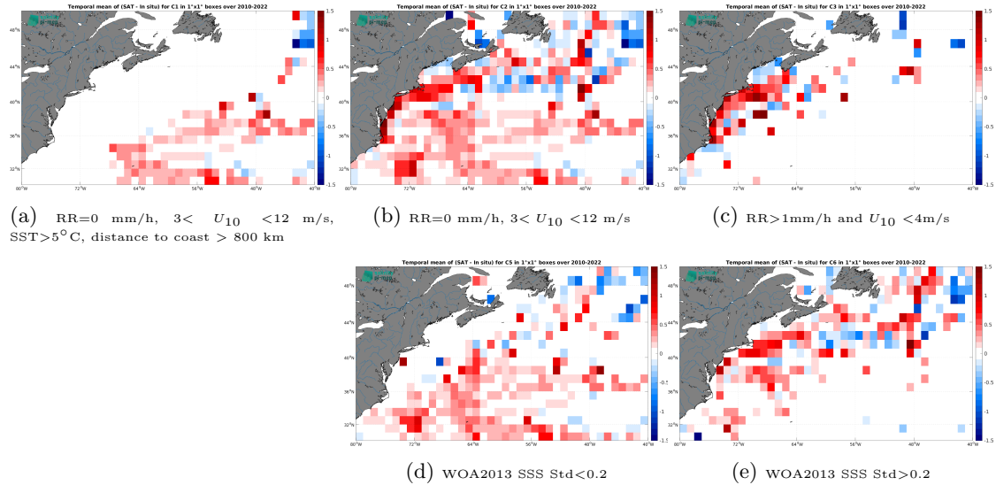
Figure 12: Temporal mean gridded over spatial boxes of size 1^{\circ}\times 1^{\circ} of \Delta\text{SSS} (SMOS SSS L3 v8 - 18 Days (CATDS-CEC-LOCEAN) - TSG (SAMOS)) for 5 different subdatasets corresponding to:RR=0 mm/h, 3 < U_{10} < 12 m/s, SST >5^{\circ}\text{C} , distance to coast > 800 km (a), RR=0 mm/h, 3 < U_{10} < 12 m/s (b), RR >1 mm/h and U_{10} < 4 m/s (c), WOA2013 SSS Std <0.2 (d), WOA2013 SSS Std >0.2 (e).
