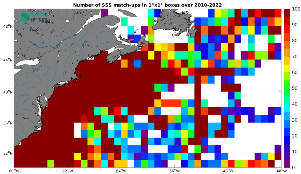
Figure 4: Number of SSS match-ups between TSG (SAMOS) SSS and the SMOS SSS L3 v8 - 18 Days (CATDS-CEC-LOCEAN) SSS product for the Gulf Stream Pi-MEP region over 1^\circ \times 1^\circ boxes and for the full satellite product period.
