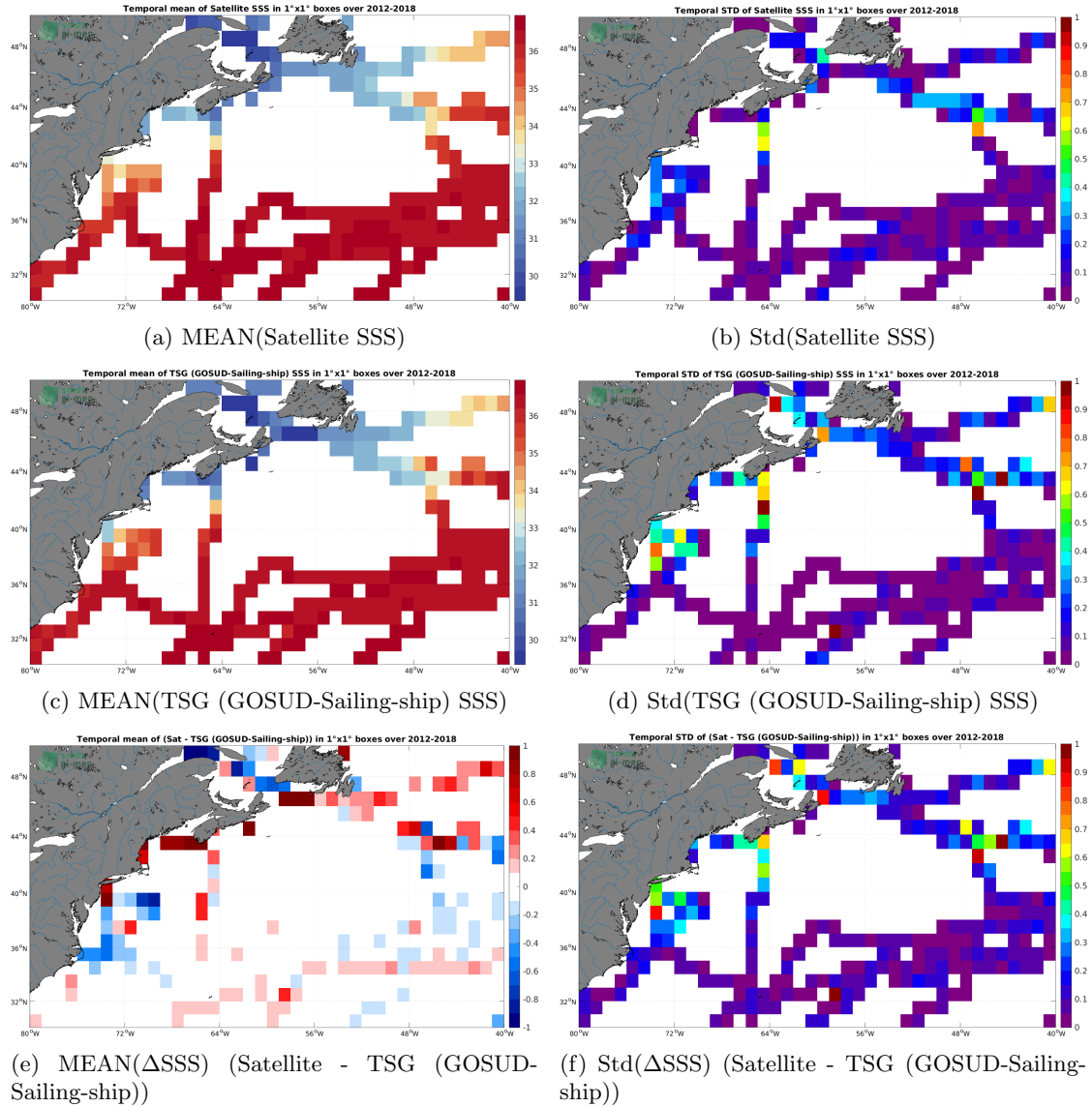
Figure 6: Temporal mean (left) and Std (right) of SSS from SMOS SSS L3 v8 - 18 Days (CATDS-CECOS-LOCEAN) (top), TSG (GOSUD-Sailing-ship) (middle), and of \Delta SSS (Satellite - TSG (GOSUD-Sailing-ship)). Only match-up pairs are used to generate these maps.
