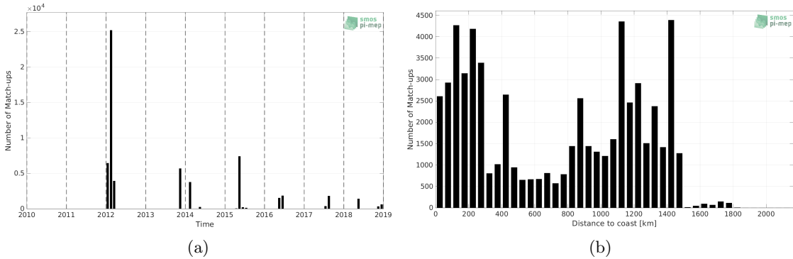
Figure 1: Number of match-ups between TSG (GOSUD-Sailing-ship) and SMOS SSS L3 v8 - 18 Days (CATDS-CECOS-LOCEAN) SSS as a function of time (a) and as function of the distance to coast (b) over the Gulf Stream Pi-MEP region and for the full satellite product period.
