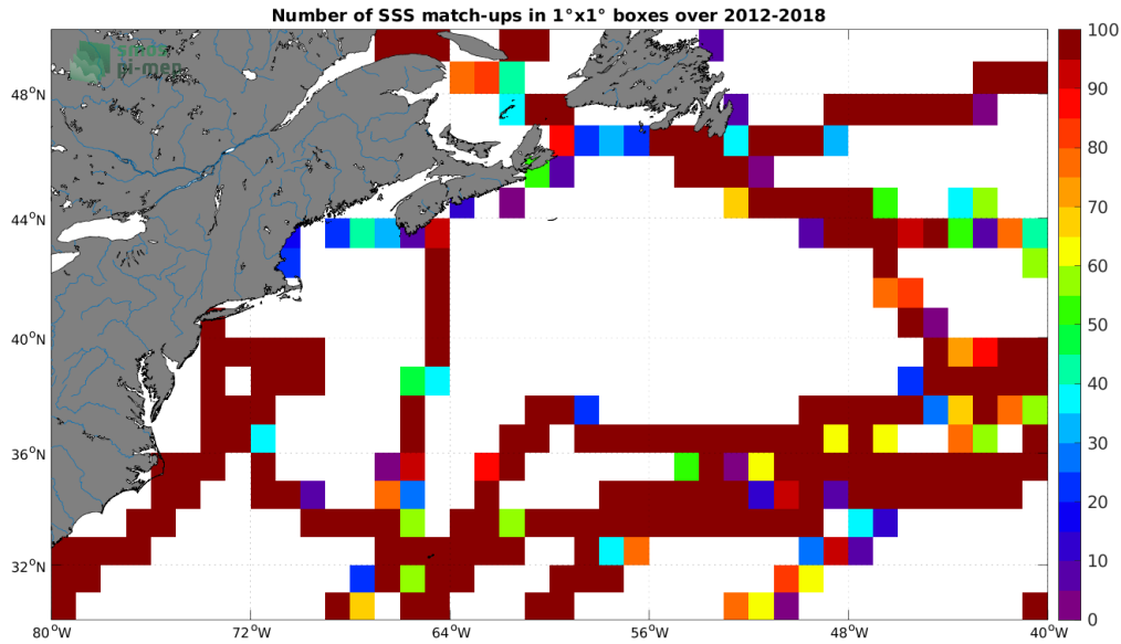
Figure 4: Number of SSS match-ups between TSG (GOSUD-Sailing-ship) SSS and the SMOS SSS L3 v8 - 18 Days (CATDS-CECOS-LOCEAN) SSS product for the Gulf Stream Pi-MEP region over 1^\circ \times 1^\circ boxes and for the full satellite product period.
