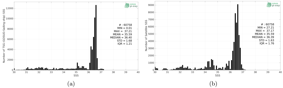
Figure 2: Histograms of SSS from TSG (GOSUD-Sailing-ship) (a) and SMOS SSS L3 v8 - 18 Days (CATDS-CECOS-LOCEAN) (b) considering all match-up pairs per bins of 0.1 over the Gulf Stream Pi-MEP region and for the full satellite product period.
