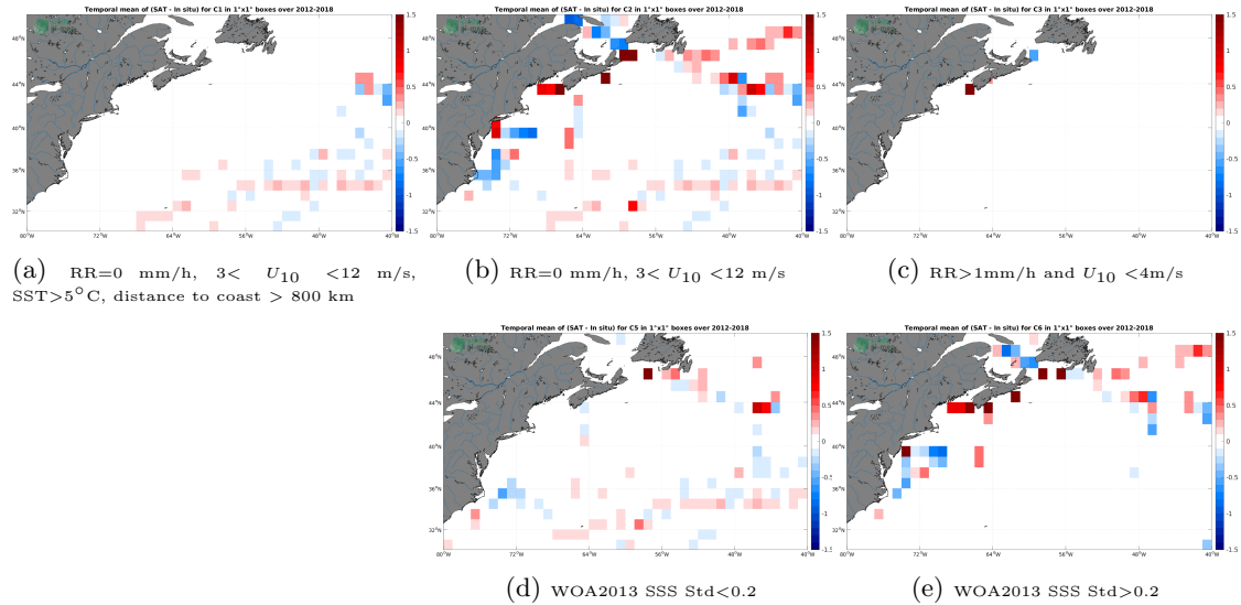
Figure 12: Temporal mean gridded over spatial boxes of size 1^{\circ}\times 1^{\circ} of \Delta SSS (SMOS SSS L3 v8 - 18 Days (CATDS-CECOS-LOCEAN) - TSG (GOSUD-Sailing-ship)) for 5 different subdatasets corresponding to:RR=0 mm/h, 3 < U_{10} < 12 m/s, SST > 5^{\circ}\text{C} , distance to coast > 800 km (a), RR=0 mm/h, 3 < U_{10} < 12 m/s (b), RR > 1 mm/h and U_{10} < 4 m/s (c), WOA2013 SSS Std < 0.2 (d), WOA2013 SSS Std > 0.2 (e).
