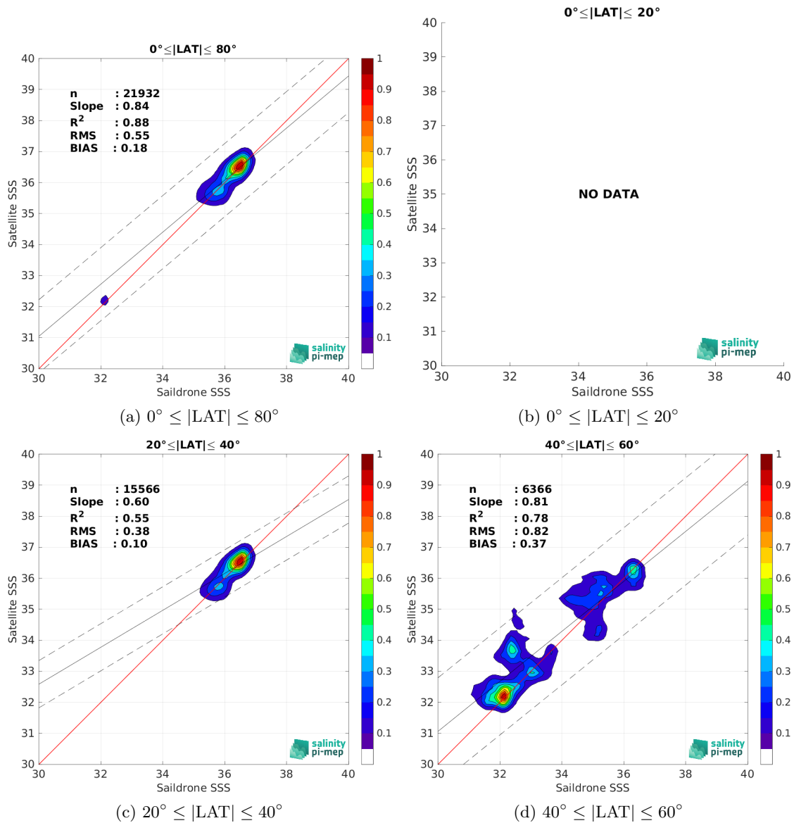
Figure 9: Contour maps of the concentration of SMOS SSS L3 v8 - 18 Days (CATDS-CEC-LOCEAN) SSS (y-axis) versus Sailldrone SSS (x-axis) at match-up pairs for different latitude bands. For each plot, the red line shows x=y . The black thin and dashed lines indicate a linear fit through the data cloud and the \pm 95\% confidence levels, respectively. The number match-up pairs n , the slope and R^2 coefficient of the linear fit, the root mean square (RMS) and the mean bias between satellite and in situ data are indicated for each latitude band in each plots.
