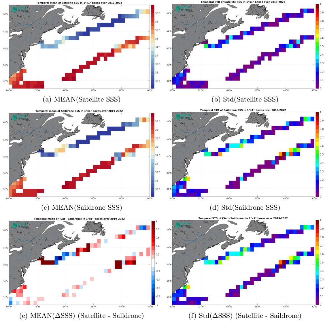
Figure 6: Temporal mean (left) and Std (right) of SSS from SMOS SSS L3 v8 - 18 Days (CATDS-CEC-LOCEAN) (top), Saildrone (middle), and of \Delta SSS (Satellite - Saildrone). Only match-up pairs are used to generate these maps.
