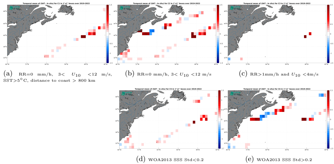
Figure 12: Temporal mean gridded over spatial boxes of size 1^\circ \times 1^\circ of \Delta SSS (SMOS SSS L3 v8 - 18 Days (CATDS-CEC-LOCEAN) - Saildrone) for 5 different subdatasets corresponding to:RR=0 mm/h, 3 < U_{10} < 12 m/s, SST >5^\circ C, distance to coast > 800 km (a), RR=0 mm/h, 3 < U_{10} < 12 m/s (b), RR >1 mm/h and U_{10} < 4 m/s (c), WOA2013 SSS Std <0.2 (d), WOA2013 SSS Std >0.2 (e).
