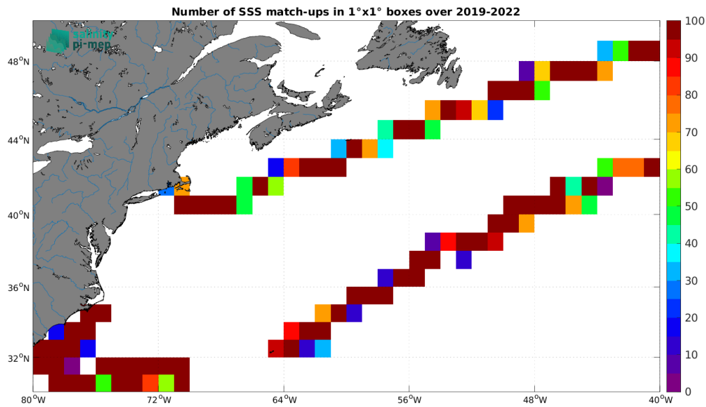
Figure 4: Number of SSS match-ups between Saildrone SSS and the SMOS SSS L3 v8 - 18 Days (CATDS-CEC-LOCEAN) SSS product for the Gulf Stream Pi-MEP region over 1^\circ \times 1^\circ boxes and for the full satellite product period.
