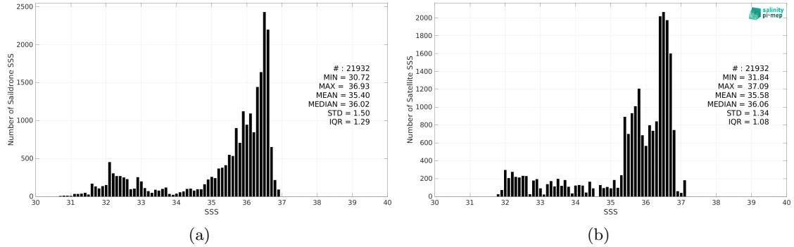
Figure 2: Histograms of SSS from Saildrone (a) and SMOS SSS L3 v8 - 18 Days (CATDS-CEC-LOCEAN) (b) considering all match-up pairs per bins of 0.1 over the Gulf Stream Pi-MEP region and for the full satellite product period.
