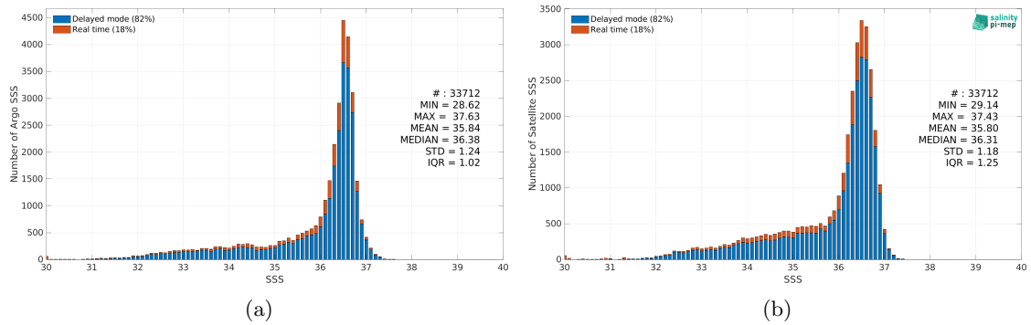
Figure 2: Histograms of SSS from Argo (a) and SMOS SSS L3 v8 - 18 Days (CATDS-CEC-LOCEAN) (b) considering all match-up pairs per bins of 0.1 over the Gulf Stream Pi-MEP region and for the full satellite product period.
