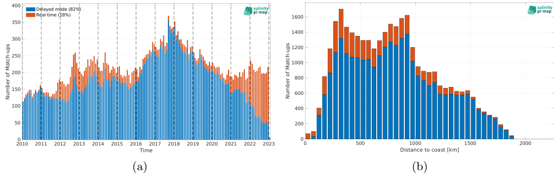
Figure 1: Number of match-ups between Argo and SMOS SSS L3 v8 - 18 Days (CATDS-CEC-LOCEAN) SSS as a function of time (a) and as function of the distance to coast (b) over the Gulf Stream Pi-MEP region and for the full satellite product period.
