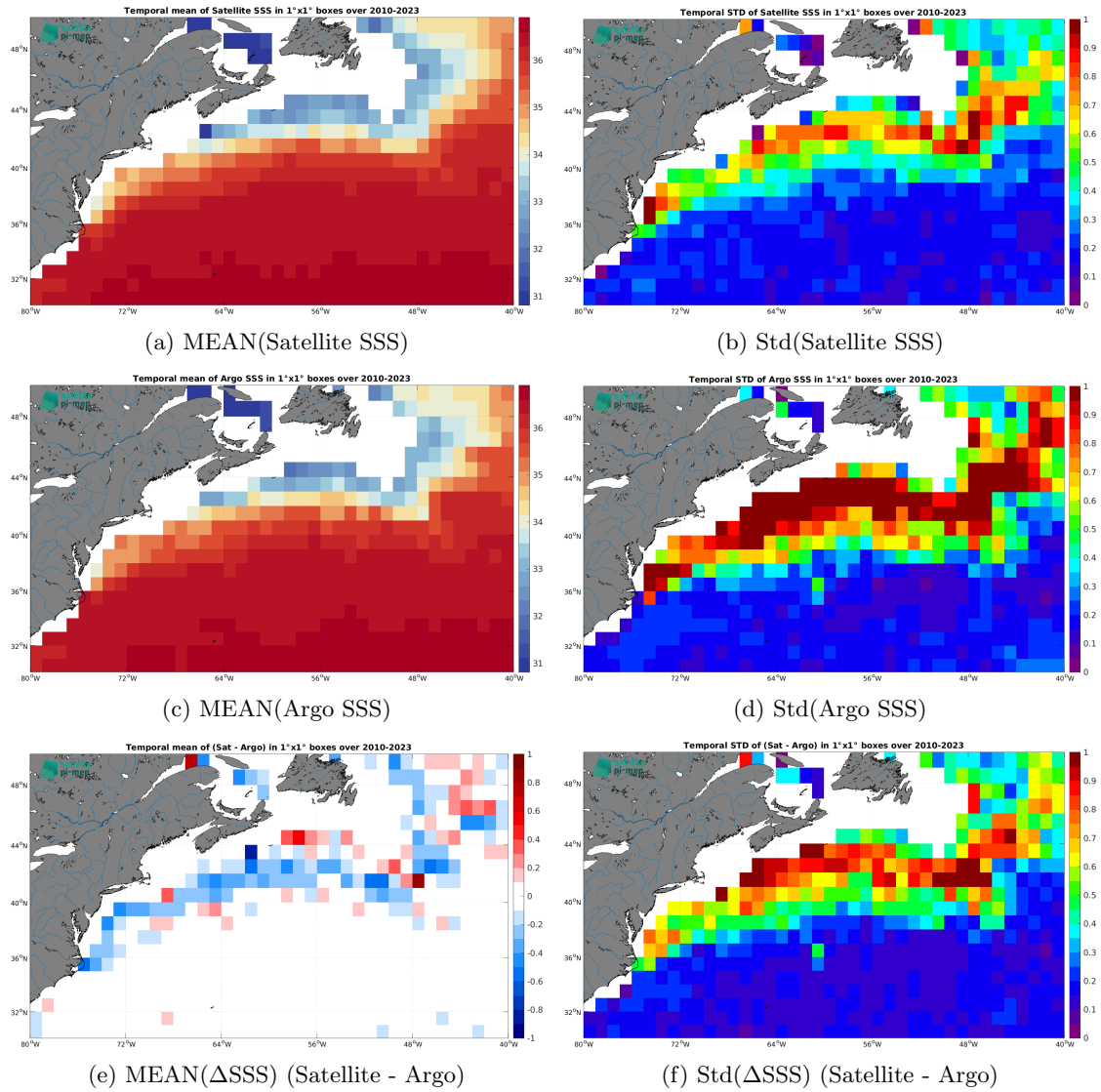
Figure 6: Temporal mean (left) and Std (right) of SSS from SMOS SSS L3 v8 - 18 Days (CATDS-CEC-LOCEAN) (top), Argo (middle), and of \Delta SSS (Satellite - Argo). Only match-up pairs are used to generate these maps.
