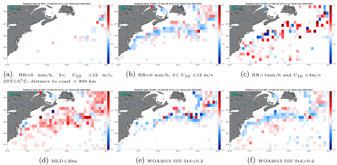
Figure 12: Temporal mean gridded over spatial boxes of size 1^\circ \times 1^\circ of \Delta SSS (SMOS SSS L3 v8 - 18 Days (CATDS-CEC-LOCEAN) - Argo) for 6 different subdatasets corresponding to:RR=0 mm/h, 3 < U_{10} < 12 m/s, SST >5^\circ C, distance to coast > 800 km (a), RR=0 mm/h, 3 < U_{10} < 12 m/s (b), RR >1 mm/h and U_{10} < 4 m/s (c),MLD <20 m (d),WOA2013 SSS Std <0.2 (e),WOA2013 SSS Std >0.2 (f).
