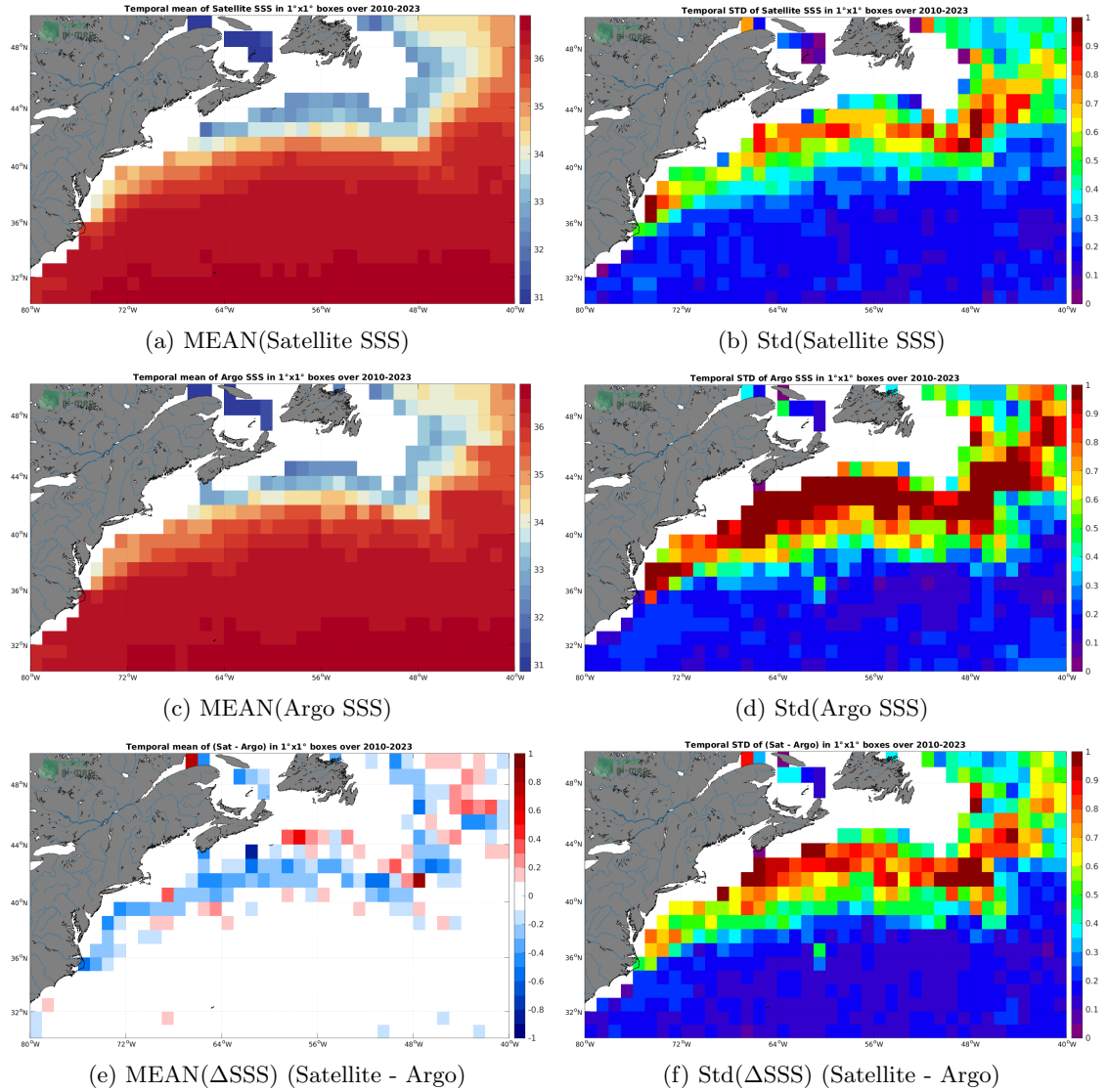
Figure 6: Temporal mean (left) and Std (right) of SSS from SMOS SSS L3 v8 - 18 Days (CATDS-CECOS-LOCEAN) (top), Argo (middle), and of \Delta SSS (Satellite - Argo). Only match-up pairs are used to generate these maps.
