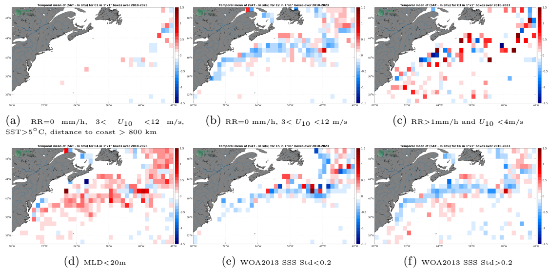
Figure 12: Temporal mean gridded over spatial boxes of size 1^\circ \times 1^\circ of \Delta SSS (SMOS SSS L3 v8 - 18 Days (CATDS-CECOS-LOCEAN) - Argo) for 6 different subdatasets corresponding to:RR=0 mm/h, 3 < U_{10} < 12 m/s, SST > 5^\circ\text{C} , distance to coast > 800 km (a), RR=0 mm/h, 3 < U_{10} < 12 m/s (b), RR > 1 mm/h and U_{10} < 4 m/s (c),MLD < 20 m (d),WOA2013 SSS Std < 0.2 (e),WOA2013 SSS Std > 0.2 (f).
