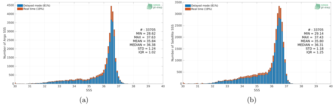
Figure 2: Histograms of SSS from Argo (a) and SMOS SSS L3 v8 - 18 Days (CATDS-CECOS-LOCEAN) (b) considering all match-up pairs per bins of 0.1 over the Gulf Stream Pi-MEP region and for the full satellite product period.
