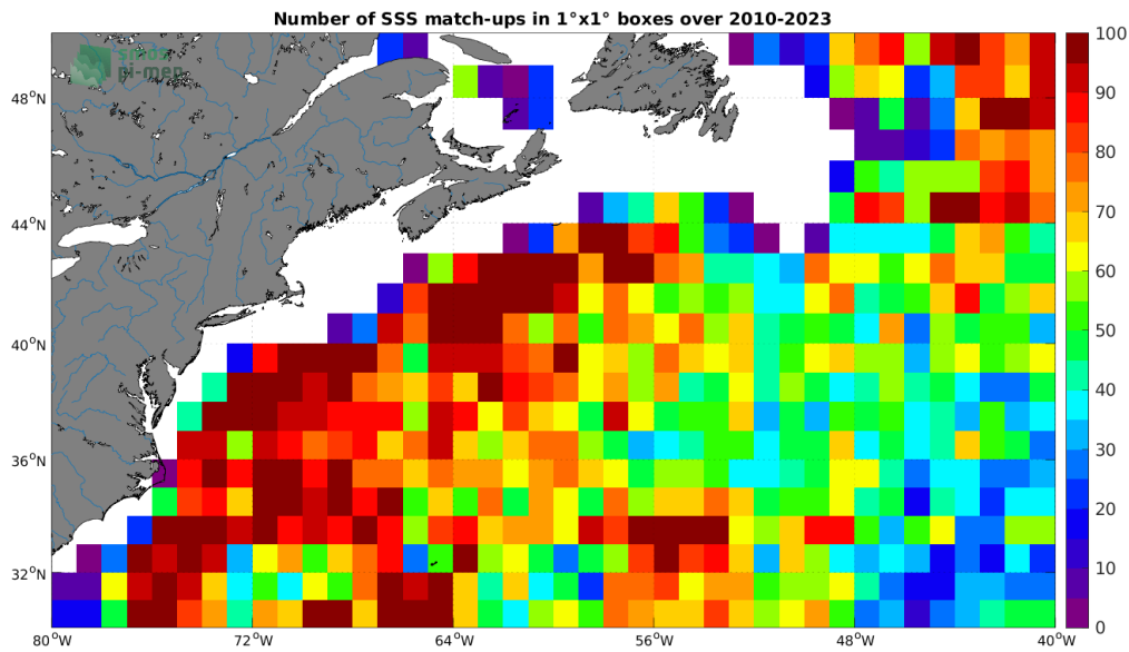
Figure 4: Number of SSS match-ups between Argo SSS and the SMOS SSS L3 v8 - 18 Days (CATDS-CECOS-LOCEAN) SSS product for the Gulf Stream Pi-MEP region over 1^\circ \times 1^\circ boxes and for the full satellite product period.
