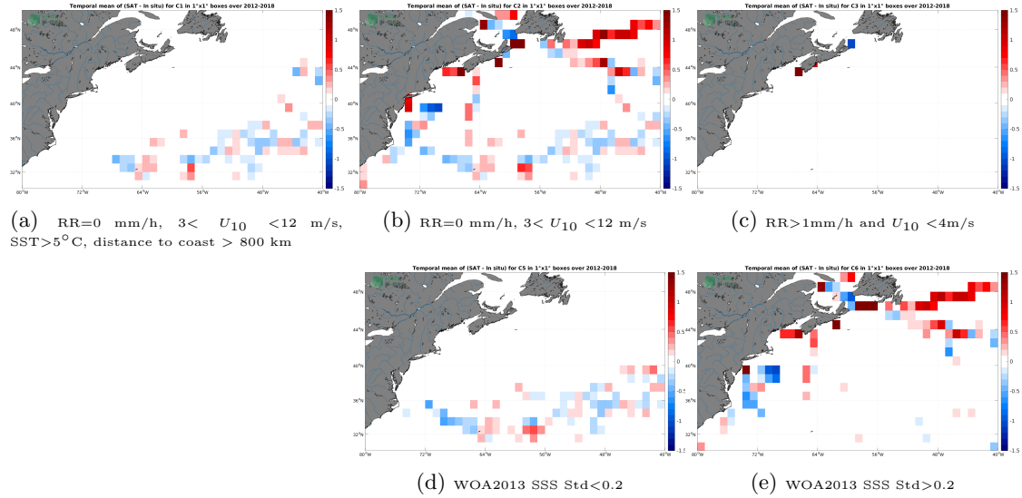
Figure 12: Temporal mean gridded over spatial boxes of size 1^{\circ}\times 1^{\circ} of \Delta SSS (SMOS SSS L3 v7 - 9 Days (CATDS-CECOS-LOCEAN) - TSG (GOSUD-Sailing-ship)) for 5 different subdatasets corresponding to:RR=0 mm/h, 3 < U_{10} < 12 m/s, SST > 5^{\circ}\text{C} , distance to coast > 800 km (a), RR=0 mm/h, 3 < U_{10} < 12 m/s (b), RR > 1 mm/h and U_{10} < 4 m/s (c), WOA2013 SSS Std < 0.2 (d), WOA2013 SSS Std > 0.2 (e).
