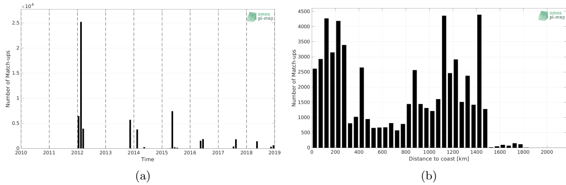
Figure 1: Number of match-ups between TSG (GOSUD-Sailing-ship) and SMOS SSS L3 v7 - 9 Days (CATDS-CECOS-LOCEAN) SSS as a function of time (a) and as function of the distance to coast (b) over the Gulf Stream Pi-MEP region and for the full satellite product period.
