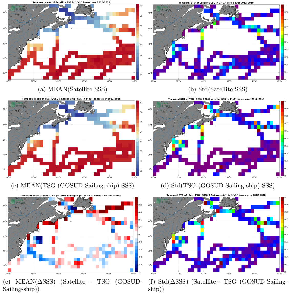
Figure 6: Temporal mean (left) and Std (right) of SSS from SMOS SSS L3 v7 - 9 Days (CATDS-CECOS-LOCEAN) (top), TSG (GOSUD-Sailing-ship) (middle), and of \Delta SSS (Satellite - TSG (GOSUD-Sailing-ship)). Only match-up pairs are used to generate these maps.
