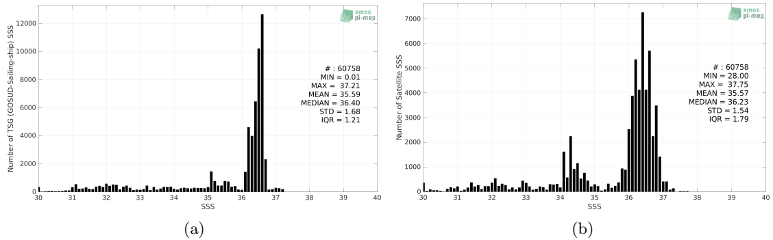
Figure 2: Histograms of SSS from TSG (GOSUD-Sailing-ship) (a) and SMOS SSS L3 v7 - 9 Days (CATDS-CECOS-LOCEAN) (b) considering all match-up pairs per bins of 0.1 over the Gulf Stream Pi-MEP region and for the full satellite product period.
