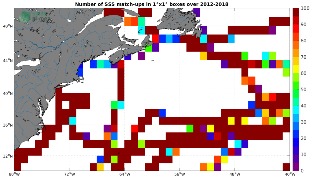
Figure 4: Number of SSS match-ups between TSG (GOSUD-Sailing-ship) SSS and the SMOS SSS L3 v7 - 9 Days (CATDS-CECOS-LOCEAN) SSS product for the Gulf Stream Pi-MEP region over 1^\circ \times 1^\circ boxes and for the full satellite product period.
