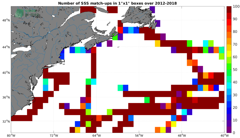
Figure 4: Number of SSS match-ups between TSG (GOSUD-Sailing-ship) SSS and the SMOS SSS L3 v7 - 18 Days (CATDS-CECOS-LOCEAN) SSS product for the Gulf Stream Pi-MEP region over 1^\circ \times 1^\circ boxes and for the full satellite product period.
