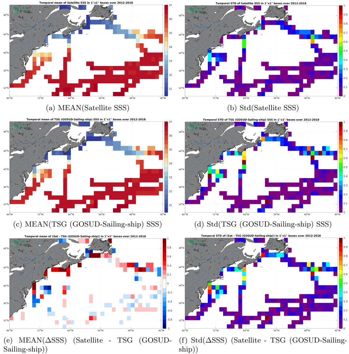
Figure 6: Temporal mean (left) and Std (right) of SSS from SMOS SSS L3 v7 - 18 Days (CATDS-CECOS-LOCEAN) (top), TSG (GOSUD-Sailing-ship) (middle), and of \Delta SSS (Satellite - TSG (GOSUD-Sailing-ship)). Only match-up pairs are used to generate these maps.
