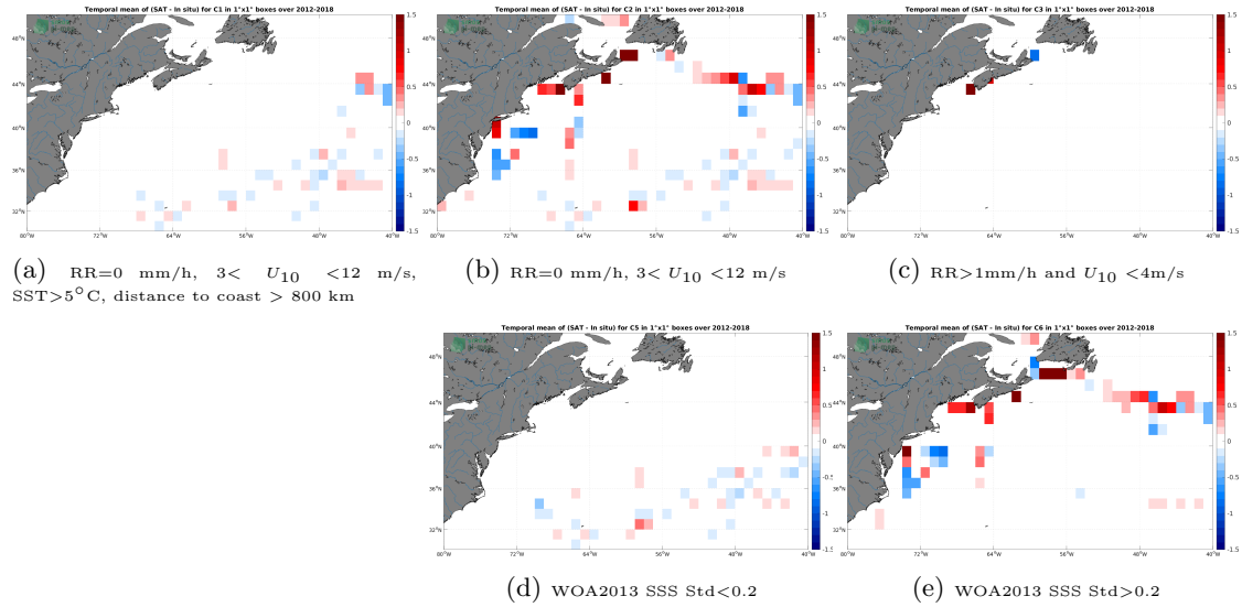
Figure 12: Temporal mean gridded over spatial boxes of size 1^{\circ}\times 1^{\circ} of \Delta SSS (SMOS SSS L3 v7 - 18 Days (CATDS-CECOS-LOCEAN) - TSG (GOSUD-Sailing-ship)) for 5 different subdatasets corresponding to:RR=0 mm/h, 3 < U_{10} < 12 m/s, SST >5^{\circ}\text{C} , distance to coast > 800 km (a), RR=0 mm/h, 3 < U_{10} < 12 m/s (b), RR >1 mm/h and U_{10} < 4 m/s (c), WOA2013 SSS Std <0.2 (d), WOA2013 SSS Std >0.2 (e).
