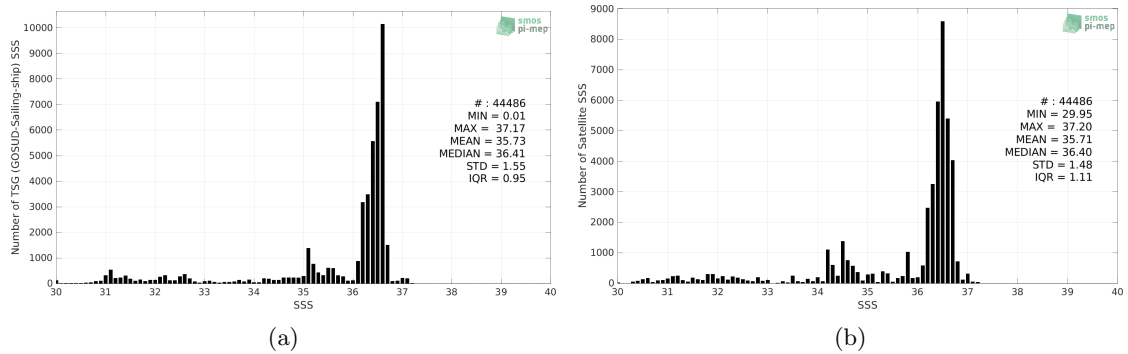
Figure 2: Histograms of SSS from TSG (GOSUD-Sailing-ship) (a) and SMOS SSS L3 v7 - 18 Days (CATDS-CECOS-LOCEAN) (b) considering all match-up pairs per bins of 0.1 over the Gulf Stream Pi-MEP region and for the full satellite product period.
