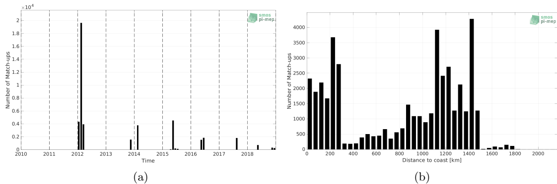
Figure 1: Number of match-ups between TSG (GOSUD-Sailing-ship) and SMOS SSS L3 v7 - 18 Days (CATDS-CECOS-LOCEAN) SSS as a function of time (a) and as function of the distance to coast (b) over the Gulf Stream Pi-MEP region and for the full satellite product period.
