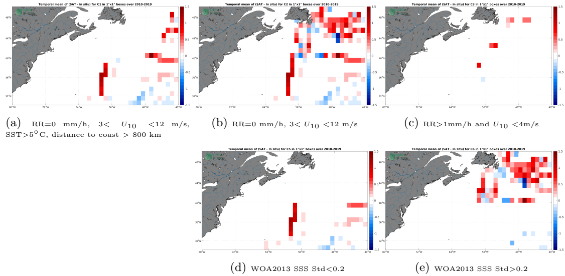
Figure 12: Temporal mean gridded over spatial boxes of size 1^{\circ}\times 1^{\circ} of \Delta SSS (SMOS SSS L3 v7 - 18 Days (CATDS-CECOS-LOCEAN) - TSG (GOSUD-Research-vessel)) for 5 different sub-datasets corresponding to:RR=0 mm/h, 3 < U_{10} < 12 m/s, SST > 5^{\circ}\text{C} , distance to coast > 800 km (a), RR=0 mm/h, 3 < U_{10} < 12 m/s (b), RR > 1 mm/h and U_{10} < 4 m/s (c), WOA2013 SSS Std < 0.2 (d), WOA2013 SSS Std > 0.2 (e).
