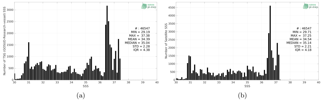
Figure 2: Histograms of SSS from TSG (GOSUD-Research-vessel) (a) and SMOS SSS L3 v7 - 18 Days (CATDS-CECOS-LOCEAN) (b) considering all match-up pairs per bins of 0.1 over the Gulf Stream Pi-MEP region and for the full satellite product period.
