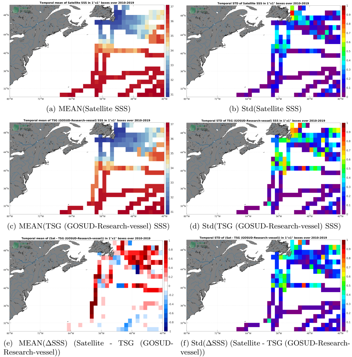
Figure 6: Temporal mean (left) and Std (right) of SSS from SMOS SSS L3 v7 - 18 Days (CATDS-CECOS-LOCEAN) (top), TSG (GOSUD-Research-vessel) (middle), and of \Delta SSS (Satellite - TSG (GOSUD-Research-vessel)). Only match-up pairs are used to generate these maps.
