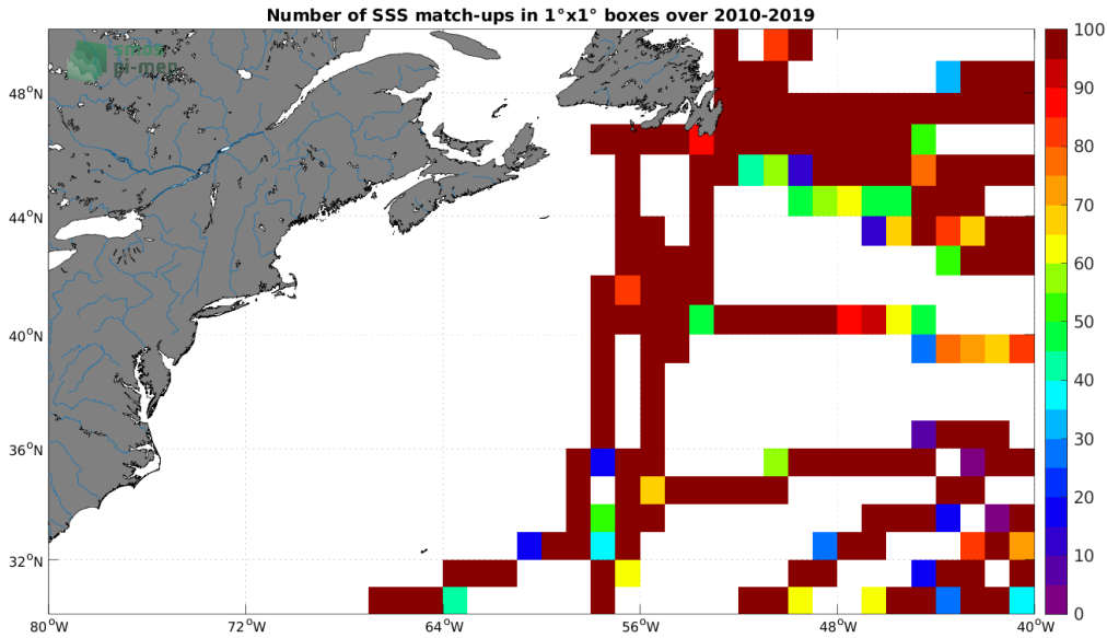
Figure 4: Number of SSS match-ups between TSG (GOSUD-Research-vessel) SSS and the SMOS SSS L3 v7 - 18 Days (CATDS-CECOS-LOCEAN) SSS product for the Gulf Stream Pi-MEP region over 1^\circ \times 1^\circ boxes and for the full satellite product period.
