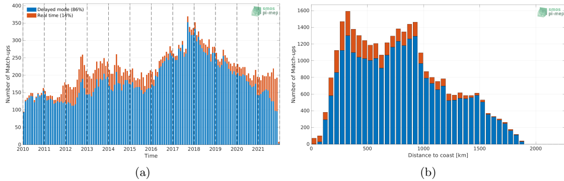
Figure 1: Number of match-ups between Argo and SMOS SSS L3 v7 - 18 Days (CATDS-CECOS-LOCEAN) SSS as a function of time (a) and as function of the distance to coast (b) over the Gulf Stream Pi-MEP region and for the full satellite product period.
