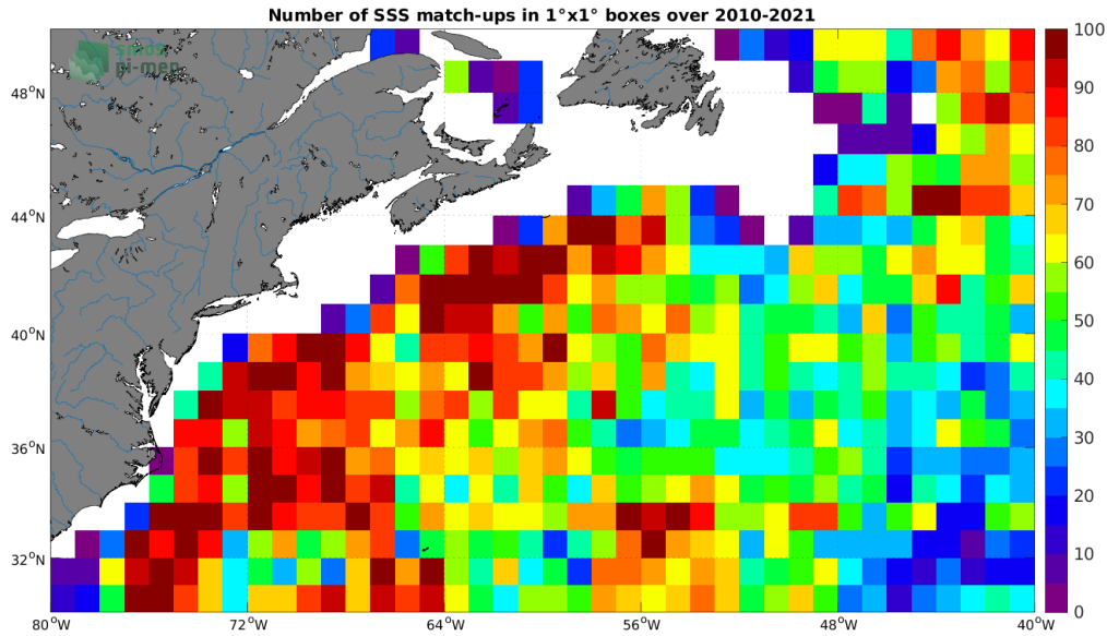
Figure 4: Number of SSS match-ups between Argo SSS and the SMOS SSS L3 v7 - 18 Days (CATDS-CECOS-LOCEAN) SSS product for the Gulf Stream Pi-MEP region over 1^\circ \times 1^\circ boxes and for the full satellite product period.
