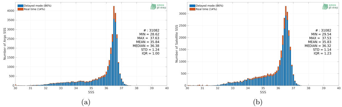
Figure 2: Histograms of SSS from Argo (a) and SMOS SSS L3 v7 - 18 Days (CATDS-CECOS-LOCEAN) (b) considering all match-up pairs per bins of 0.1 over the Gulf Stream Pi-MEP region and for the full satellite product period.
