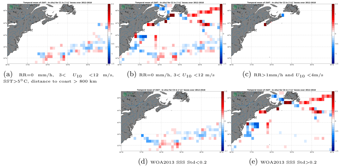
Figure 12: Temporal mean gridded over spatial boxes of size 1^\circ \times 1^\circ of \Delta SSS (SMOS SSS L3 v5 - 9 Days (CATDS-CECOS-LOCEAN) - TSG (GOSUD-Sailing-ship)) for 5 different subdatasets corresponding to:RR=0 mm/h, 3 < U_{10} < 12 m/s, SST >5^\circ\text{C} , distance to coast > 800 km (a), RR=0 mm/h, 3 < U_{10} < 12 m/s (b), RR >1 mm/h and U_{10} < 4 m/s (c), WOA2013 SSS Std <0.2 (d), WOA2013 SSS Std >0.2 (e).
