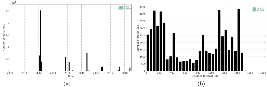
Figure 1: Number of match-ups between TSG (GOSUD-Sailing-ship) and SMOS SSS L3 v5 - 9 Days (CATDS-CECOS-LOCEAN) SSS as a function of time (a) and as function of the distance to coast (b) over the Gulf Stream Pi-MEP region and for the full satellite product period.
