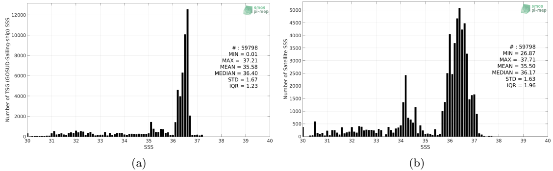
Figure 2: Histograms of SSS from TSG (GOSUD-Sailing-ship) (a) and SMOS SSS L3 v5 - 9 Days (CATDS-CECOS-LOCEAN) (b) considering all match-up pairs per bins of 0.1 over the Gulf Stream Pi-MEP region and for the full satellite product period.
