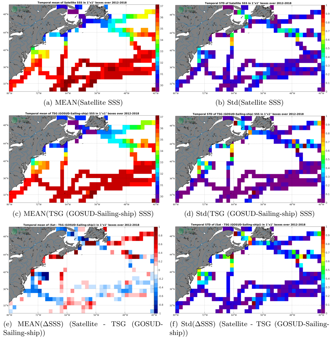
Figure 6: Temporal mean (left) and Std (right) of SSS from SMOS SSS L3 v5 - 9 Days (CATDS-CECOS-LOCEAN) (top), TSG (GOSUD-Sailing-ship) (middle), and of \Delta SSS (Satellite - TSG (GOSUD-Sailing-ship)). Only match-up pairs are used to generate these maps.
