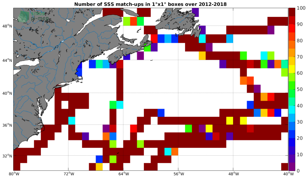
Figure 4: Number of SSS match-ups between TSG (GOSUD-Sailing-ship) SSS and the SMOS SSS L3 v5 - 9 Days (CATDS-CECOS-LOCEAN) SSS product for the Gulf Stream Pi-MEP region over 1^\circ \times 1^\circ boxes and for the full satellite product period.
