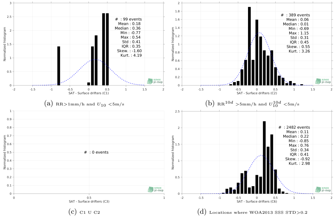
Figure 12: Normalized histogram of \Delta\text{SSS} (SMOS-L3-CATDS-CECOS-LOCEAN-V3-9DAYS-25KM - Surface drifters) for 6 different subdatasets corresponding to: RR > 1mm/h and U_{10} < 5\text{m/s} (a), RR^{10d} > 5\text{mm/h} and U_{10}^{10d} < 5\text{m/s} (b), C1 U C2 (c), Locations where WOA2013 SSS STD > 0.2 (d).
