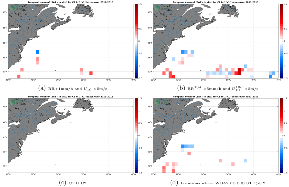
Figure 11: Temporal mean gridded over spatial boxes of size 1^\circ \times 1^\circ of \Delta SSS (SMOS-L3-CATDS-CECOS-LOCEAN-V3-9DAYS-25KM - Surface drifters) for 4 different subdatasets corresponding to: RR > 1 mm/h and U_{10} < 5 m/s (a), RR 10d > 5 mm/h and U_{10}^{10d} < 5 m/s (b), C1 U C2 (c), Locations where WOA2013 SSS STD > 0.2 (d).
