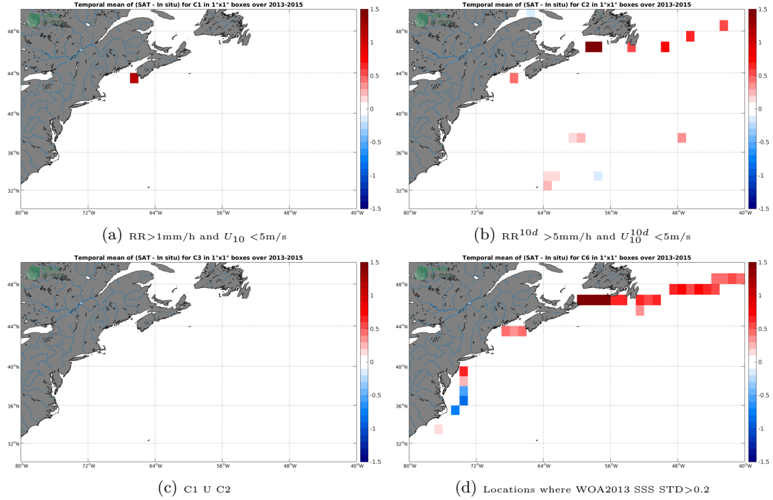
Figure 12: Temporal mean gridded over spatial boxes of size 1^\circ \times 1^\circ of \Delta SSS (SMOS-L3-CATDS-CECOS-LOCEAN-V3-18DAYS-25KM - TSG-GOSUD-Sailing-ship) for 4 different subdatasets corresponding to: RR > 1\text{mm/h} and U_{10} < 5\text{m/s} (a), RR^{10d} > 5\text{mm/h} and U_{10}^{10d} < 5\text{m/s} (b), C1 U C2 (c), Locations where WOA2013 SSS STD > 0.2 (d).
