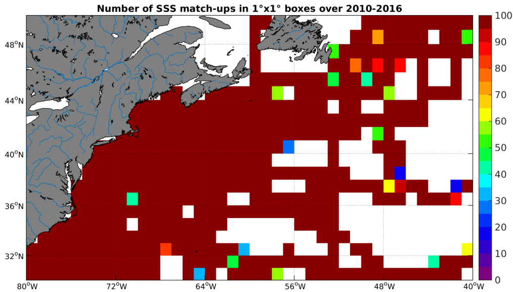
Figure 4: Number of SSS match-ups between TSG-SAMOS SSS and the SMOS-L3-CATDS-CECOS-LOCEAN-V2.1-9DAYS-25KM SSS product for the Gulf Stream Pi-MEP region over 1^\circ \times 1^\circ boxes and for the full satellite product period.
