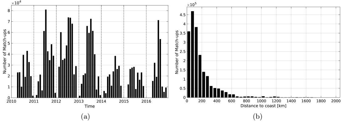
Figure 1: Number of match-ups between TSG-SAMOS and SMOS-L3-CATDS-CECOS-LOCEAN-V2.1-9DAYS-25KM SSS as a function of time (a) and as function of the distance to coast (b) over the Gulf Stream Pi-MEP region and for the full satellite product period.
