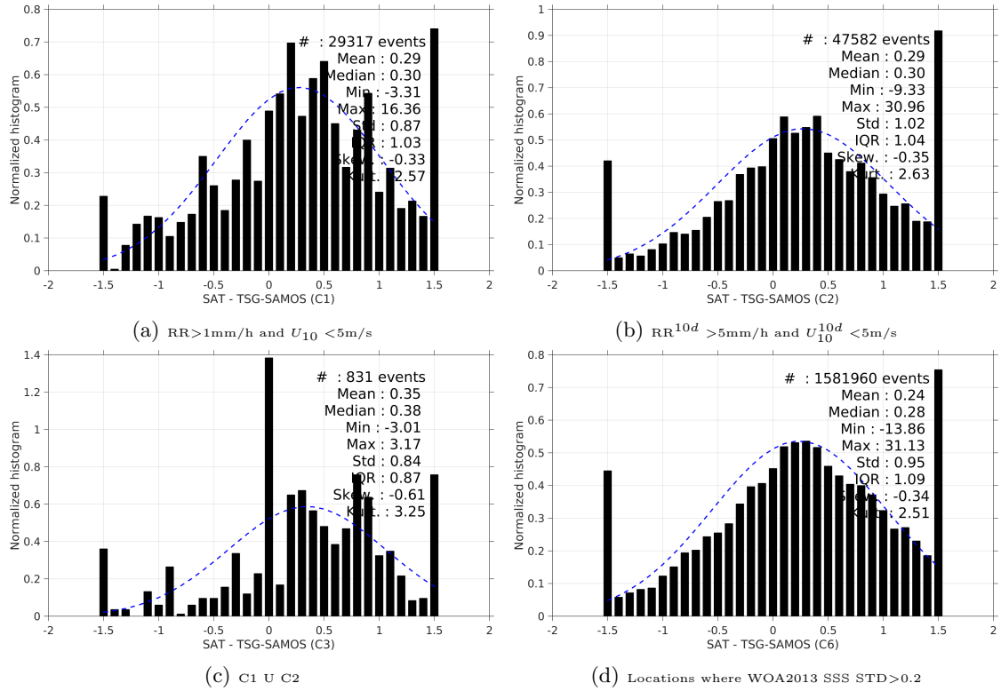
Figure 13: Normalized histogram of \Delta\text{SSS} (SMOS-L3-CATDS-CECOS-LOCEAN-V2.1-9DAYS-25KM - TSG-SAMOS) for 6 different subdatasets corresponding to: \text{RR} > 1\text{mm/h} and U_{10} < 5\text{m/s} (a), \text{RR}^{10d} > 5\text{mm/h} and U_{10}^{10d} < 5\text{m/s} (b), C1 U C2 (c), Locations where WOA2013 SSS STD > 0.2 (d).
