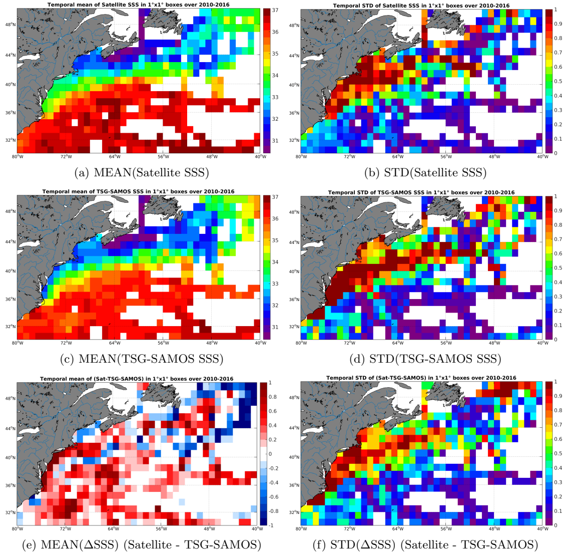
Figure 6: Temporal mean (left) and STD (right) of SSS from SMOS-L3-CATDS-CECOS-LOCEAN-V2.1-9DAYS-25KM (top), TSG-SAMOS (middle), and of \Delta SSS (Satellite - TSG-SAMOS). Only match-up pairs are used to generate these maps.
