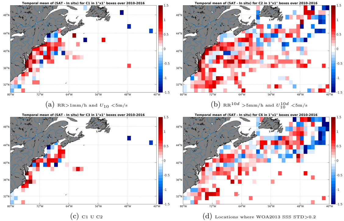
Figure 12: Temporal mean gridded over spatial boxes of size 1^\circ \times 1^\circ of \Delta SSS (SMOS-L3-CATDS-CECOS-LOCEAN-V2.1-9DAYS-25KM - TSG-SAMOS) for 4 different subdatasets corresponding to: RR > 1\text{mm/h} and U_{10} < 5\text{m/s} (a), RR^{10d} > 5\text{mm/h} and U_{10}^{10d} < 5\text{m/s} (b), C1 U C2 (c), Locations where WOA2013 SSS STD > 0.2 (d).
