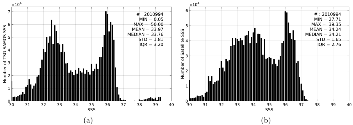
Figure 2: Histograms of SSS from TSG-SAMOS (a) and SMOS-L3-CATDS-CECOS-LOCEAN-V2.1-9DAYS-25KM (b) considering all match-up pairs per bins of 0.1 over the Gulf Stream Pi-MEP region and for the full satellite product period.
