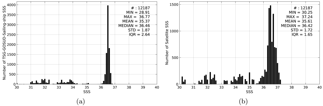
Figure 2: Histograms of SSS from TSG-GOSUD-Sailing-ship (a) and SMOS-L3-CATDS-CECOS-LOCEAN-V2.1-9DAYS-25KM (b) considering all match-up pairs per bins of 0.1 over the Gulf Stream Pi-MEP region and for the full satellite product period.
