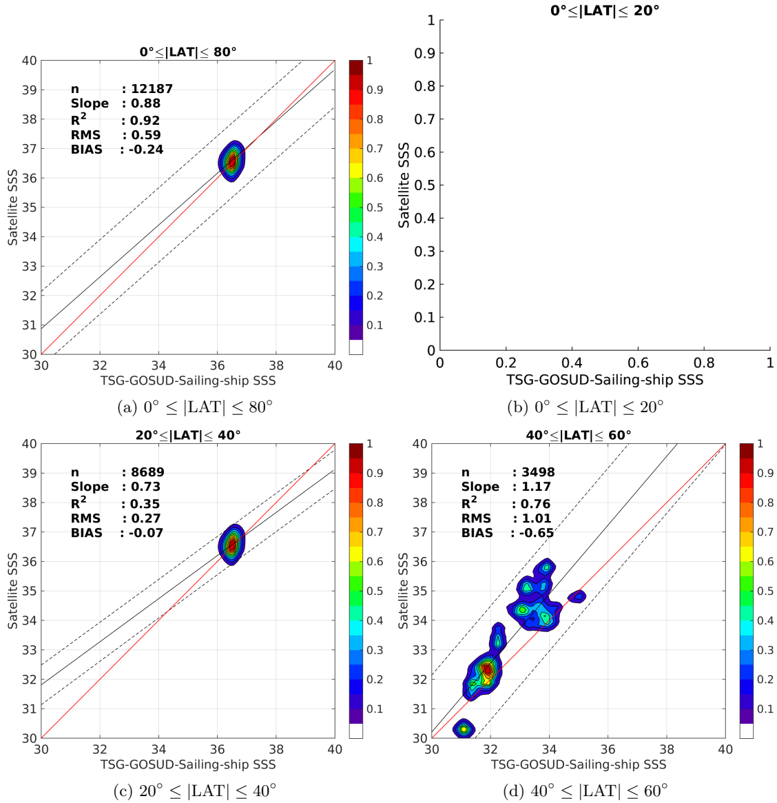
Figure 9: Contour maps of the concentration of SMOS-L3-CATDS-CECOS-LOCEAN-V2.1-9DAYS-25KM SSS (y-axis) versus TSG-GOSUD-Sailing-ship SSS (x-axis) at match-up pairs for different latitude bands. For each plot, the red line shows x=y . The black thin and dashed lines indicate a linear fit through the data cloud and the \pm 95\% confidence levels, respectively. The number match-up pairs n , the slope and R^2 coefficient of the linear fit, the root mean square (RMS) and the mean bias between satellite and in situ data are indicated for each latitude band in each plots.
