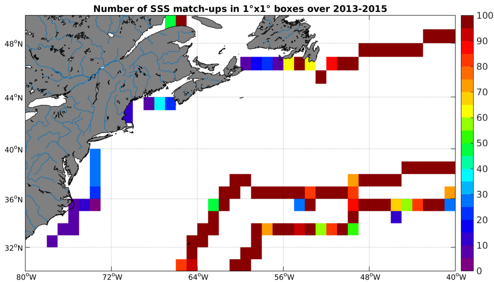
Figure 4: Number of SSS match-ups between TSG-GOSUD-Sailing-ship SSS and the SMOS-L3-CATDS-CECOS-LOCEAN-V2.1-9DAYS-25KM SSS product for the Gulf Stream Pi-MEP region over 1^\circ \times 1^\circ boxes and for the full satellite product period.
