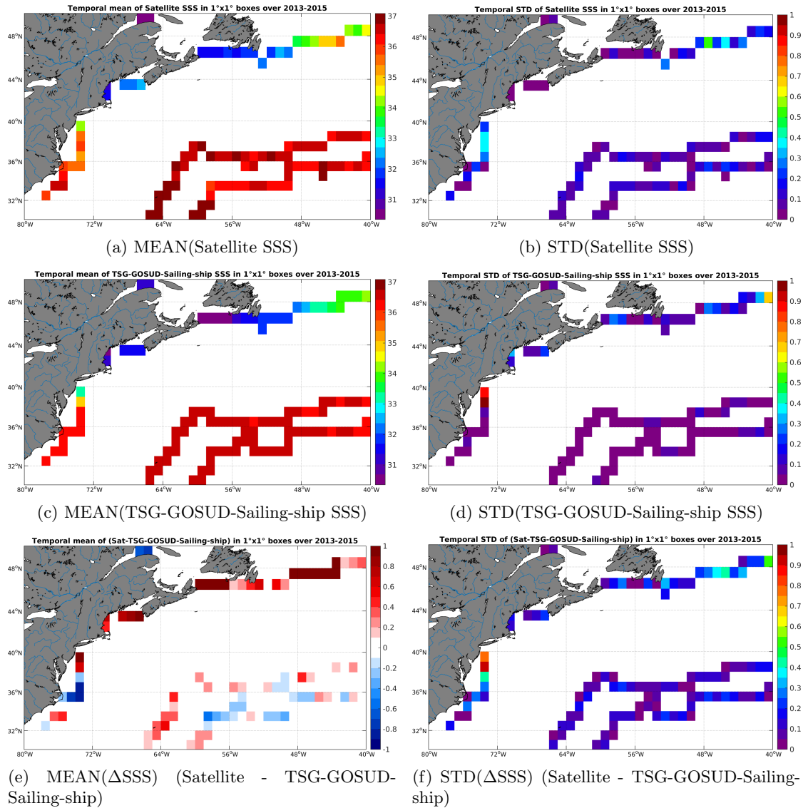
Figure 6: Temporal mean (left) and STD (right) of SSS from SMOS-L3-CATDS-CECOS-LOCEAN-V2.1-9DAYS-25KM (top), TSG-GOSUD-Sailing-ship (middle), and of \Delta SSS (Satellite - TSG-GOSUD-Sailing-ship). Only match-up pairs are used to generate these maps.
