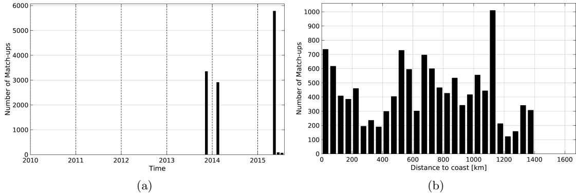
Figure 1: Number of match-ups between TSG-GOSUD-Sailing-ship and SMOS-L3-CATDS-CECOS-LOCEAN-V2.1-9DAYS-25KM SSS as a function of time (a) and as function of the distance to coast (b) over the Gulf Stream Pi-MEP region and for the full satellite product period.
