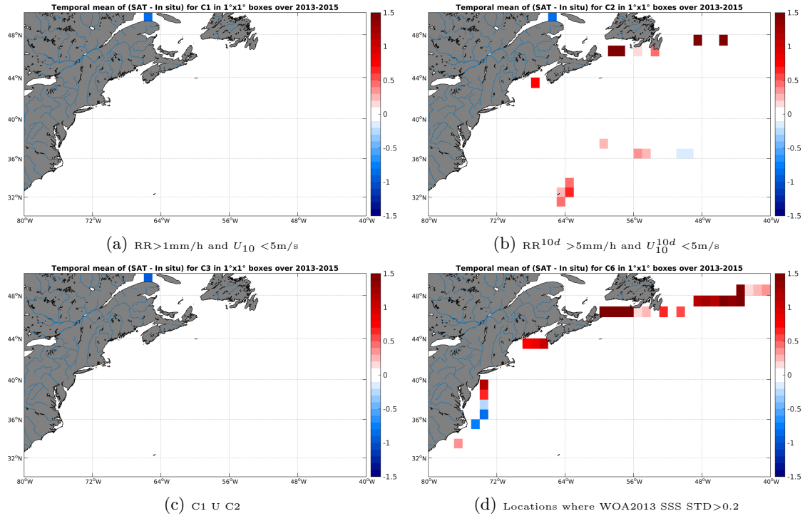
Figure 12: Temporal mean gridded over spatial boxes of size 1^\circ \times 1^\circ of \Delta SSS (SMOS-L3-CATDS-CECOS-LOCEAN-V2.1-9DAYS-25KM - TSG-GOSUD-Sailing-ship) for 4 different subdatasets corresponding to:RR>1mm/h and U_{10} < 5\text{m/s} (a), RR^{10d} > 5\text{mm/h} and U_{10}^{10d} < 5\text{m/s} (b), C1 U C2 (c),Locations where WOA2013 SSS STD>0.2 (d).
