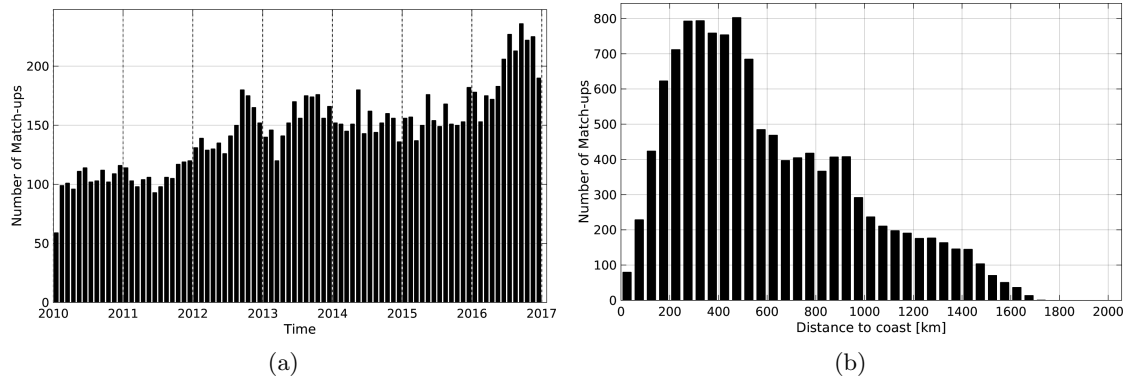
Figure 1: Number of match-ups between Argo and SMOS-L3-CATDS-CECOS-LOCEAN-V2-18DAYS-25KM SSS as a function of time (a) and as function of the distance to coast (b) over the Gulf Stream Pi-MEP region and for the full satellite product period.
