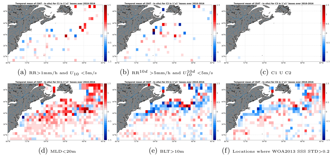
Figure 12: Temporal mean gridded over spatial boxes of size 1^\circ \times 1^\circ of \Delta SSS (SMOS-L3-CATDS-CECOS-LOCEAN-V2-18DAYS-25KM - Argo) for 6 different subdatasets corresponding to:RR>1mm/h and U_{10} < 5\text{m/s} (a), RR^{10d} > 5\text{mm/h} and U_{10}^{10d} < 5\text{m/s} (b), C1 U C2 (c),MLD<20m (d),BLT>10m (e),Locations where WOA2013 SSS STD>0.2 (f).
