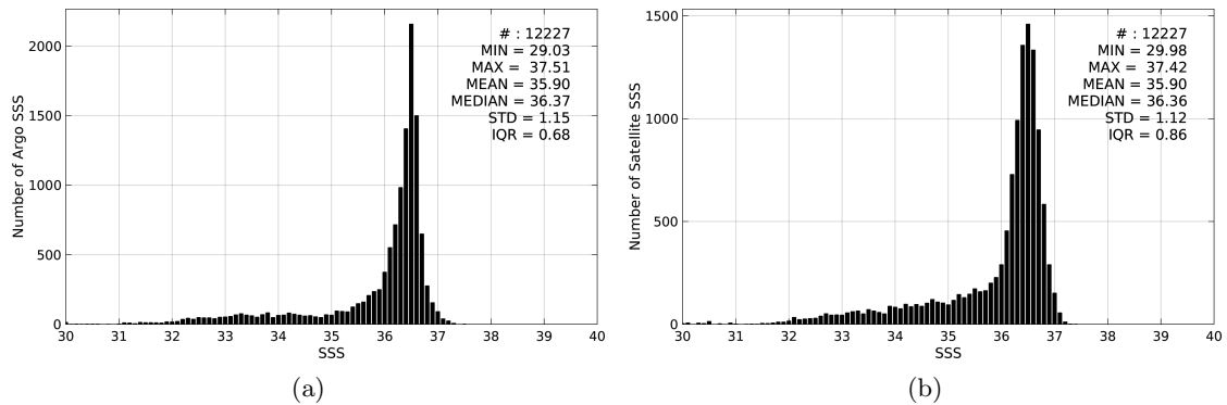
Figure 2: Histograms of SSS from Argo (a) and SMOS-L3-CATDS-CECOS-LOCEAN-V2-18DAYS-25KM (b) considering all match-up pairs per bins of 0.1 over the Gulf Stream Pi-MEP region and for the full satellite product period.
