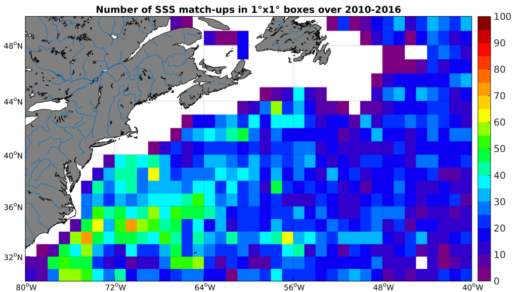
Figure 4: Number of SSS match-ups between Argo SSS and the SMOS-L3-CATDS-CECOS-LOCEAN-V2-18DAYS-25KM SSS product for the Gulf Stream Pi-MEP region over 1°x1° boxes and for the full satellite product period.
