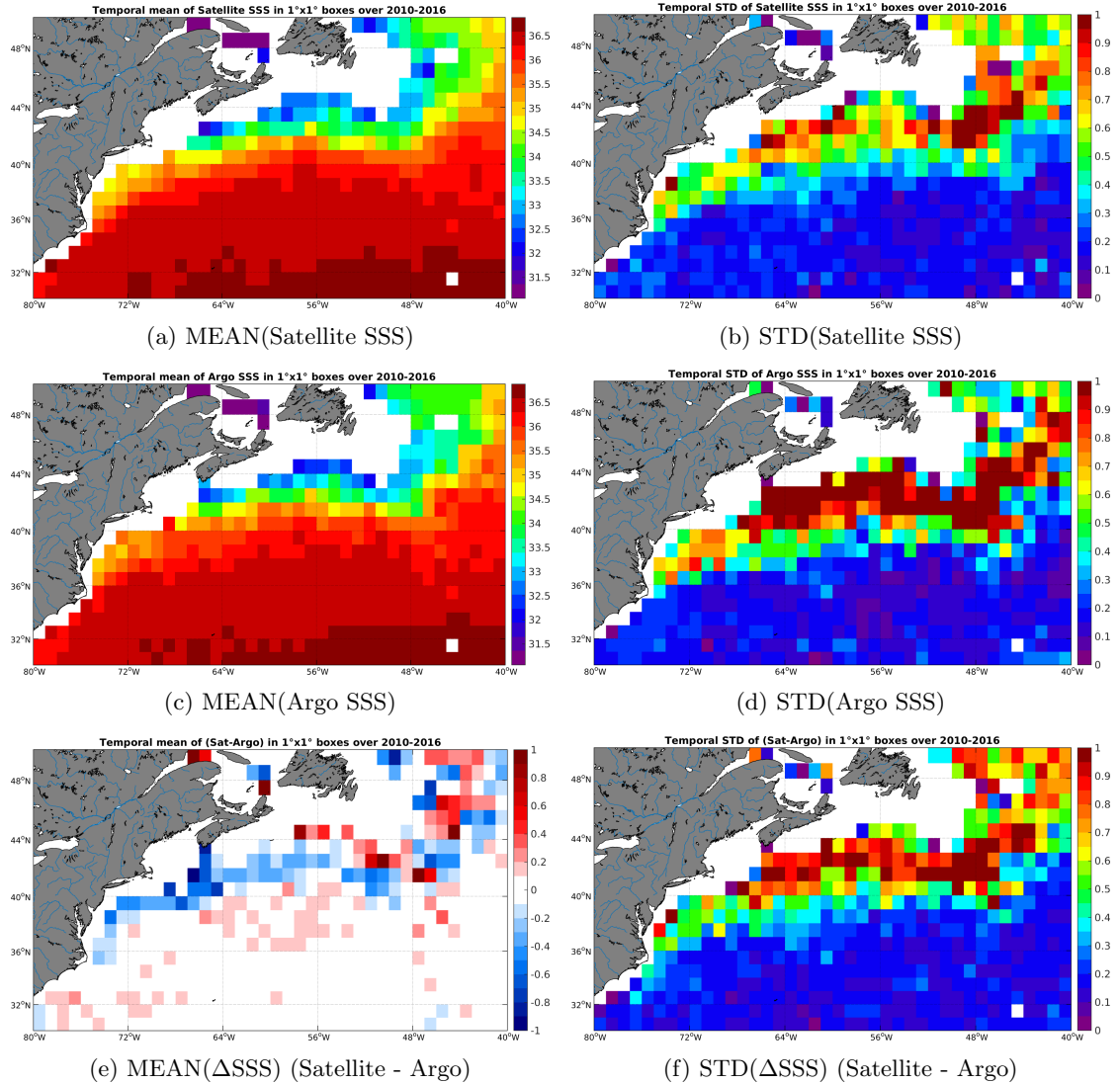
Figure 6: Temporal mean (left) and STD (right) of SSS from SMOS-L3-CATDS-CECOS-LOCEAN-V2-18DAYS-25KM (top), Argo (middle), and of \Delta SSS (Satellite - Argo). Only match-up pairs are used to generate these maps.
