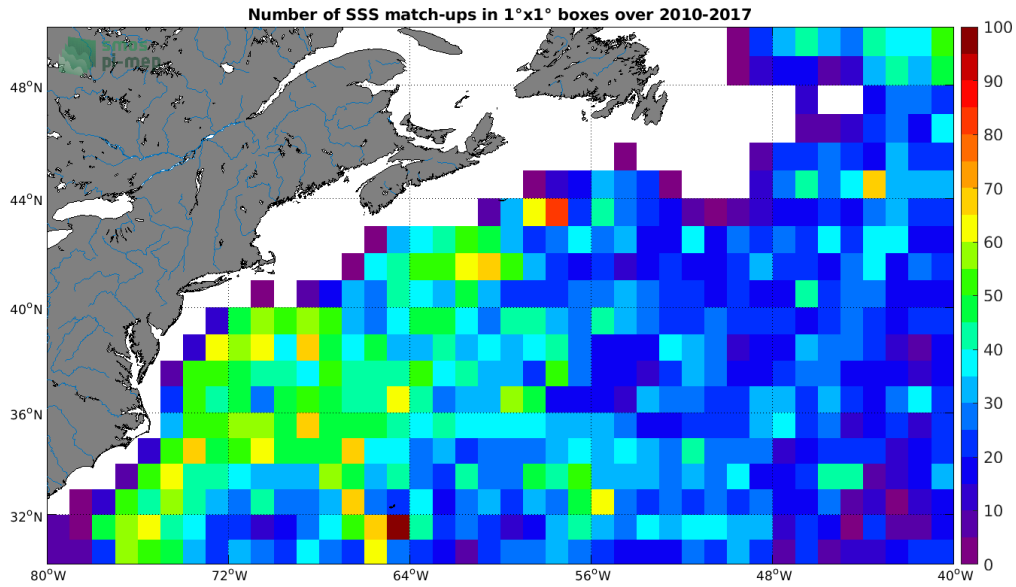
Figure 4: Number of SSS match-ups between Argo SSS and the SMOS SSS L3 v2 - Monthly - 0.25 Deg (CATDS-CECOS-IFREMER) SSS product for the Gulf Stream Pi-MEP region over 1^\circ \times 1^\circ boxes and for the full satellite product period.
