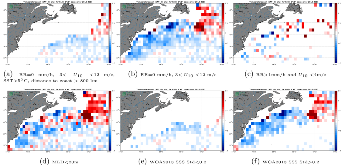
Figure 12: Temporal mean gridded over spatial boxes of size 1^\circ \times 1^\circ of \Delta SSS (SMOS SSS L3 v2 - Monthly - 0.25 Deg (CATDS-CECOS-IFREMER) - Argo) for 6 different subdatasets corresponding to: RR=0 mm/h, 3 < U_{10} < 12 m/s, SST >5^\circ C, distance to coast > 800 km (a), RR=0 mm/h, 3 < U_{10} < 12 m/s (b), RR>1 mm/h and U_{10} < 4 m/s (c), MLD <20 m (d), WOA2013 SSS Std <0.2 (e), WOA2013 SSS Std >0.2 (f).
