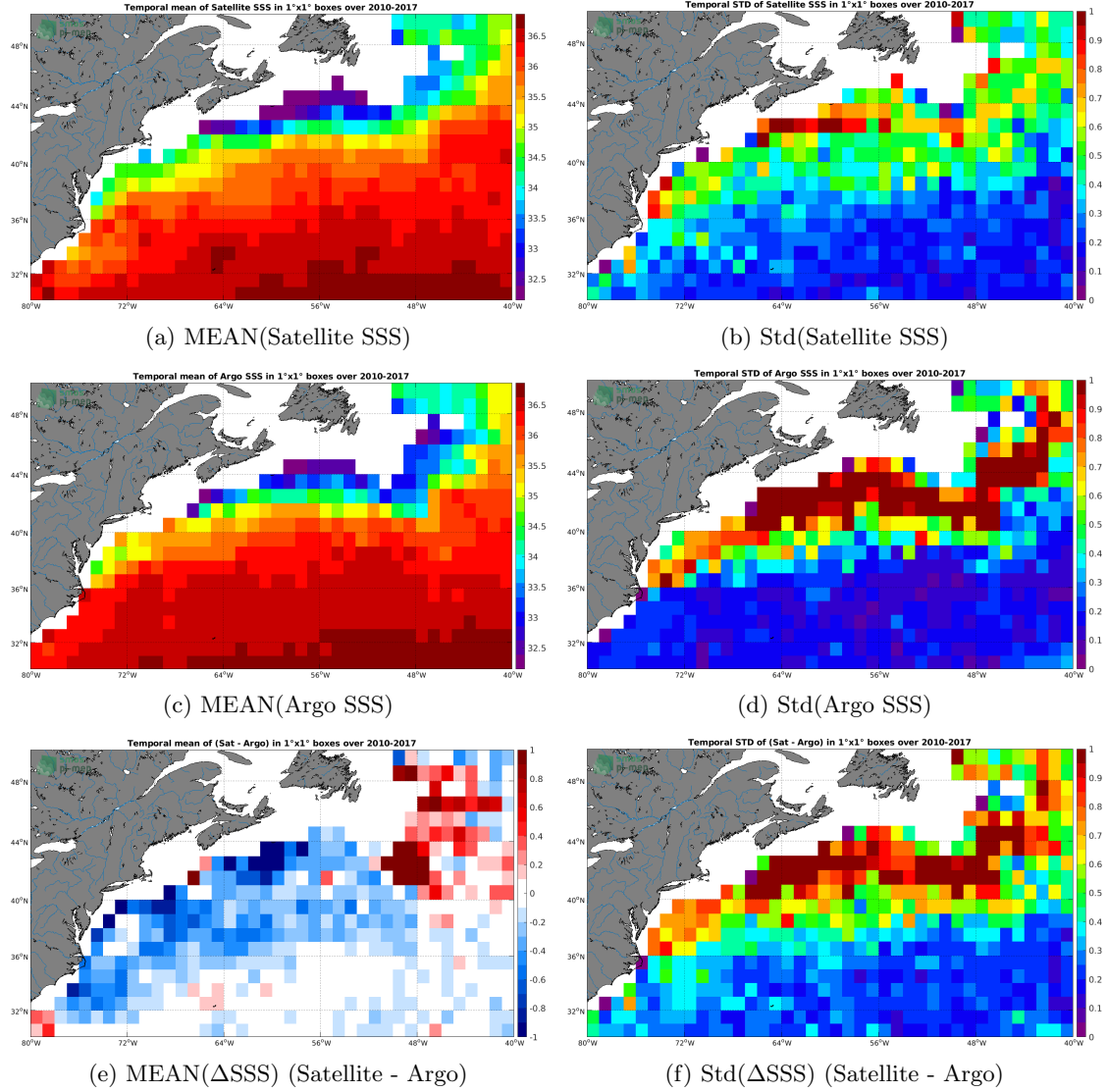
Figure 6: Temporal mean (left) and Std (right) of SSS from SMOS SSS L3 v2 - Monthly - 0.25 Deg (CATDS-CECOS-IFREMER) (top), Argo (middle), and of \Delta SSS (Satellite - Argo). Only match-up pairs are used to generate these maps.
