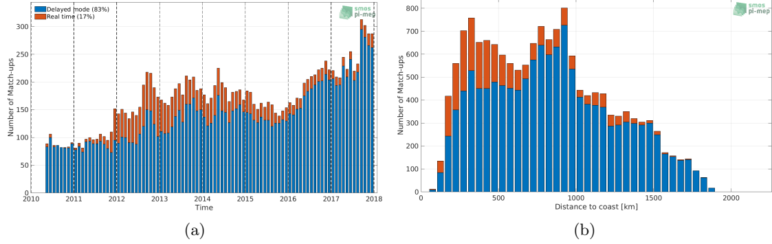
Figure 1: Number of match-ups between Argo and SMOS SSS L3 v2 - Monthly - 0.25 Deg (CATDS-CECOS-IFREMER) SSS as a function of time (a) and as function of the distance to coast (b) over the Gulf Stream Pi-MEP region and for the full satellite product period.
