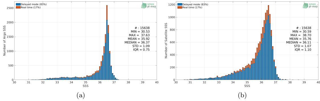
Figure 2: Histograms of SSS from Argo (a) and SMOS SSS L3 v2 - Monthly - 0.25 Deg (CATDS-CECOS-IFREMER) (b) considering all match-up pairs per bins of 0.1 over the Gulf Stream Pi-MEP region and for the full satellite product period.
