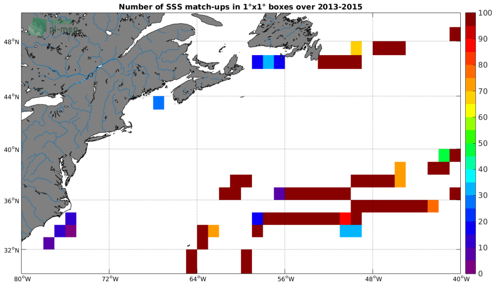
Figure 4: Number of SSS match-ups between TSG-GOSUD-Sailing-ship SSS and the SMOS-L3-CATDS-CECOS-IFREMER-V2-1DAY-0.5DEG SSS product for the Gulf Stream Pi-MEP region over 1°x1° boxes and for the full satellite product period.
