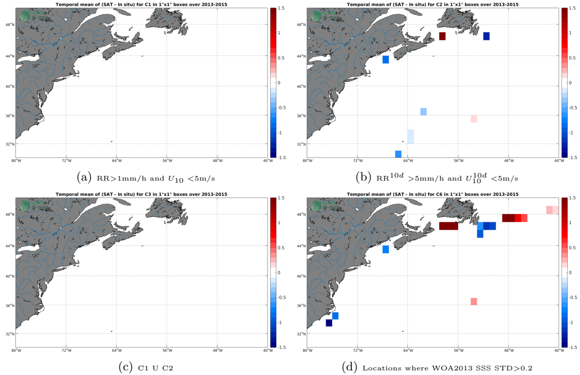
Figure 12: Temporal mean gridded over spatial boxes of size 1^\circ \times 1^\circ of \Delta SSS (SMOS-L3-CATDS-CECOS-IFREMER-V2-1DAY-0.5DEG - TSG-GOSUD-Sailing-ship) for 4 different subdatasets corresponding to: RR > 1\text{mm/h} and U_{10} < 5\text{m/s} (a), RR^{10d} > 5\text{mm/h} and U_{10}^{10d} < 5\text{m/s} (b), C1 U C2 (c), Locations where WOA2013 SSS STD > 0.2 (d).
