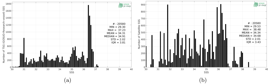
Figure 2: Histograms of SSS from TSG (GOSUD-Research-vessel) (a) and SMOS SSS L3 v2 - Daily - 0.5 Deg (CATDS-CECOS-IFREMER) (b) considering all match-up pairs per bins of 0.1 over the Gulf Stream Pi-MEP region and for the full satellite product period.
