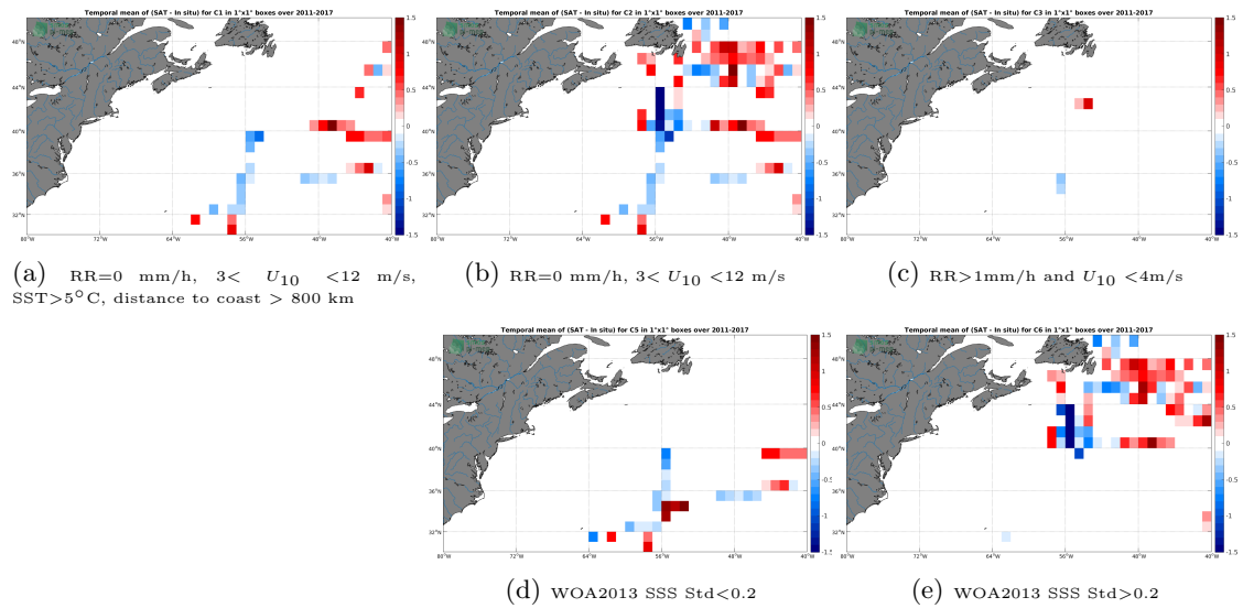
Figure 12: Temporal mean gridded over spatial boxes of size 1^\circ \times 1^\circ of \Delta SSS (SMOS SSS L3 v2 - Daily - 0.5 Deg (CATDS-CECOS-IFREMER) - TSG (GOSUD-Research-vessel)) for 5 different subdatasets corresponding to:RR=0 mm/h, 3 < U_{10} < 12 m/s, SST > 5^\circ\text{C} , distance to coast > 800 km (a), RR=0 mm/h, 3 < U_{10} < 12 m/s (b), RR > 1 mm/h and U_{10} < 4 m/s (c), WOA2013 SSS Std < 0.2 (d), WOA2013 SSS Std > 0.2 (e).
