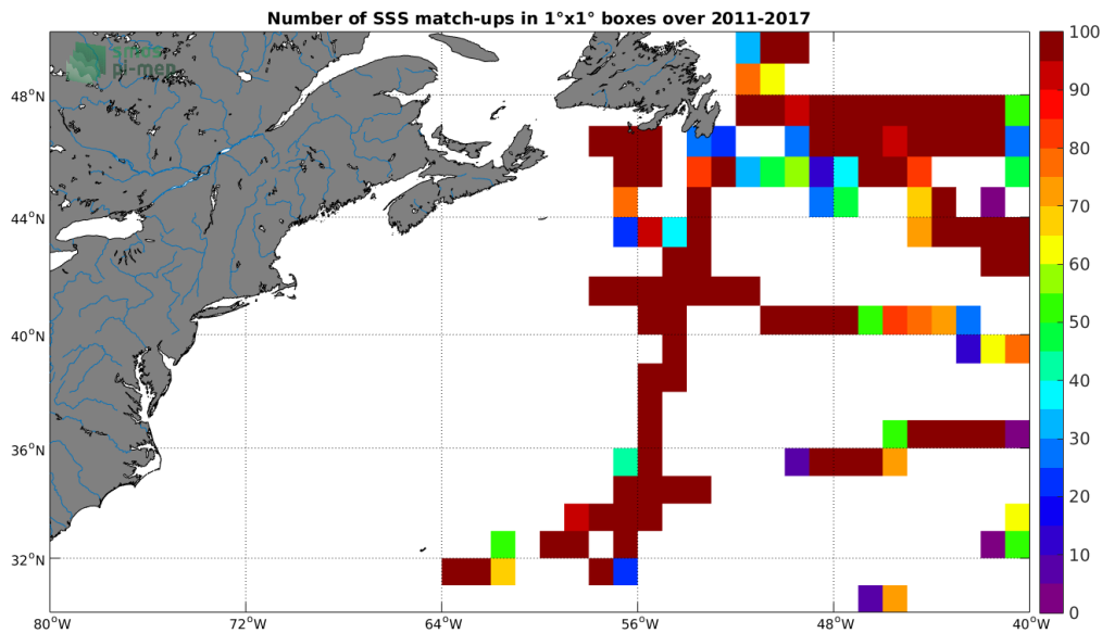
Figure 4: Number of SSS match-ups between TSG (GOSUD-Research-vessel) SSS and the SMOS SSS L3 v2 - Daily - 0.5 Deg (CATDS-CECOS-IFREMER) SSS product for the Gulf Stream Pi-MEP region over 1^\circ \times 1^\circ boxes and for the full satellite product period.
