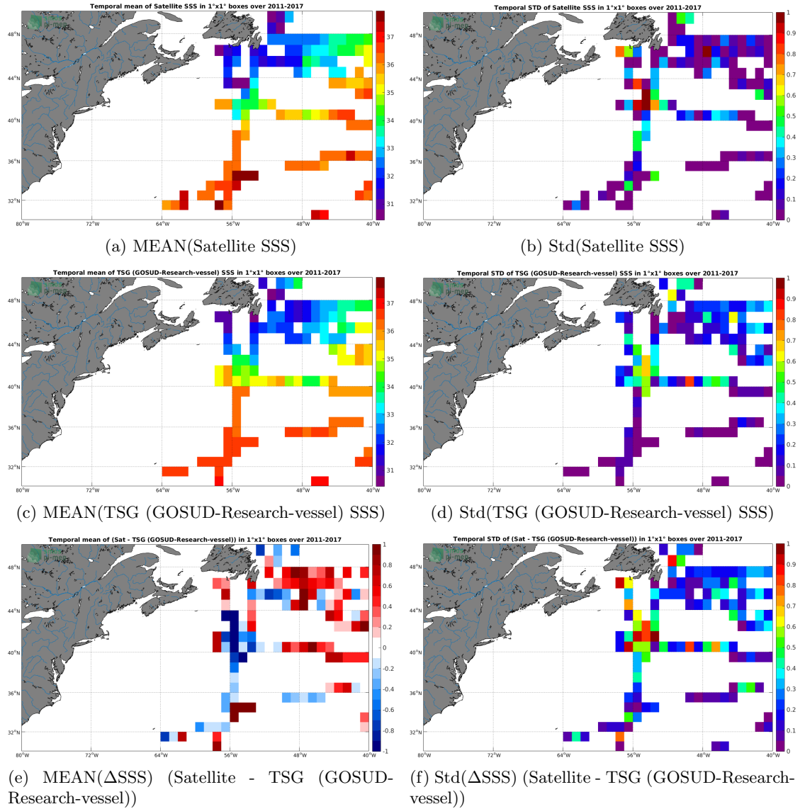
Figure 6: Temporal mean (left) and Std (right) of SSS from SMOS SSS L3 v2 - Daily - 0.5 Deg (CATDS-CECOS-IFREMER) (top), TSG (GOSUD-Research-vessel) (middle), and of \Delta SSS (Satellite - TSG (GOSUD-Research-vessel)). Only match-up pairs are used to generate these maps.
