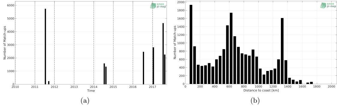
Figure 1: Number of match-ups between TSG-GOSUD-Research-vessel and SMOS-L3-CATDS-CECOS-IFREMER-V2-1DAY-0.5DEG SSS as a function of time (a) and as function of the distance to coast (b) over the Gulf Stream Pi-MEP region and for the full satellite product period.
