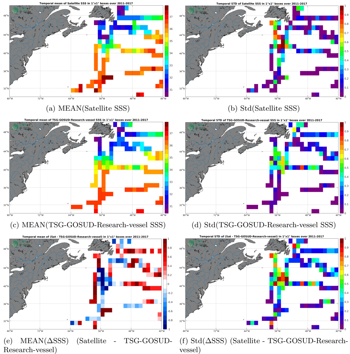
Figure 6: Temporal mean (left) and Std (right) of SSS from SMOS-L3-CATDS-CECOS-IFREMER-V2-1DAY-0.5DEG (top), TSG-GOSUD-Research-vessel (middle), and of \Delta SSS (Satellite - TSG-GOSUD-Research-vessel). Only match-up pairs are used to generate these maps.
