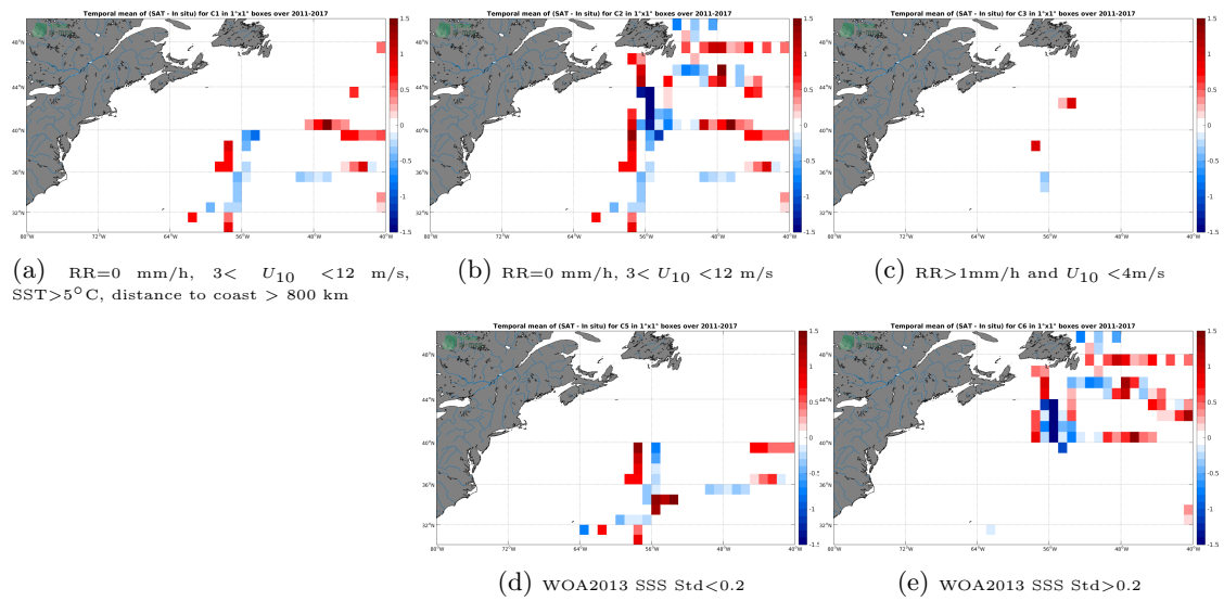
Figure 12: Temporal mean gridded over spatial boxes of size 1^\circ \times 1^\circ of \Delta SSS (SMOS-L3-CATDS-CECOS-IFREMER-V2-1DAY-0.5DEG - TSG-GOSUD-Research-vessel) for 5 different subdatasets corresponding to:RR=0 mm/h, 3 < U_{10} < 12 m/s, SST>5°C, distance to coast > 800 km (a), RR=0 mm/h, 3 < U_{10} < 12 m/s (b), RR>1mm/h and U_{10} < 4 m/s (c), WOA2013 SSS Std<0.2 (d), WOA2013 SSS Std>0.2 (e).
