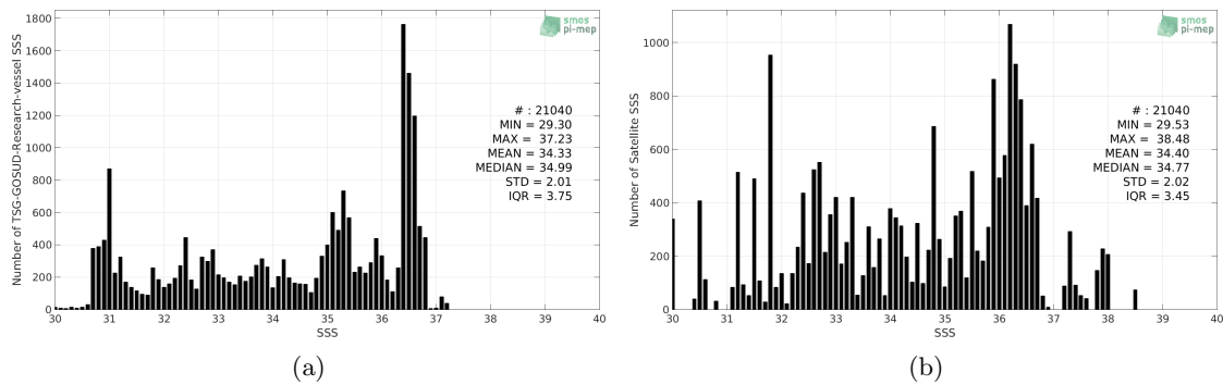
Figure 2: Histograms of SSS from TSG-GOSUD-Research-vessel (a) and SMOS-L3-CATDS-CECOS-IFREMER-V2-1DAY-0.5DEG (b) considering all match-up pairs per bins of 0.1 over the Gulf Stream Pi-MEP region and for the full satellite product period.
