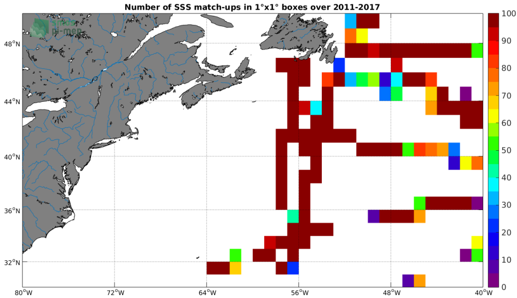
Figure 4: Number of SSS match-ups between TSG-GOSUD-Research-vessel SSS and the SMOS-L3-CATDS-CECOS-IFREMER-V2-1DAY-0.5DEG SSS product for the Gulf Stream Pi-MEP region over 1^\circ \times 1^\circ boxes and for the full satellite product period.
