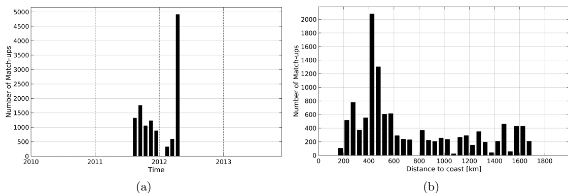
Figure 1: Number of match-ups between Surface drifters and SMOS-L3-CATDS-CECOS-IFREMER-V2-1DAY-0.5deg SSS as a function of time (a) and as function of the distance to coast (b) over the Gulf Stream Pi-MEP region and for the full satellite product period.
