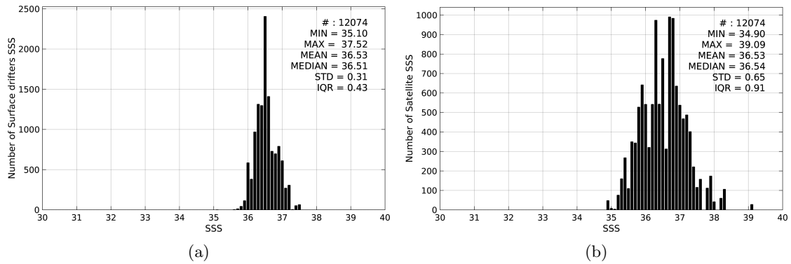
Figure 2: Histograms of SSS from Surface drifters (a) and SMOS-L3-CATDS-CECOS-IFREMER-V2-1DAY-0.5deg (b) considering all match-up pairs per bins of 0.1 over the Gulf Stream Pi-MEP region and for the full satellite product period.
