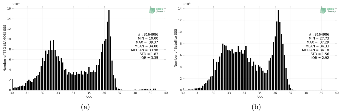
Figure 2: Histograms of SSS from TSG (SAMOS) (a) and SMOS SSS L3 v335 - Monthly - 25 km (CATDS-CPDC) (b) considering all match-up pairs per bins of 0.1 over the Gulf Stream Pi-MEP region and for the full satellite product period.
