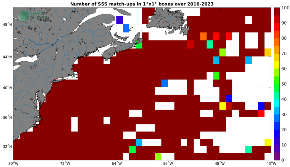
Figure 4: Number of SSS match-ups between TSG (SAMOS) SSS and the SMOS SSS L3 v335 - Monthly - 25 km (CATDS-CPDC) SSS product for the Gulf Stream Pi-MEP region over 1^\circ \times 1^\circ boxes and for the full satellite product period.
