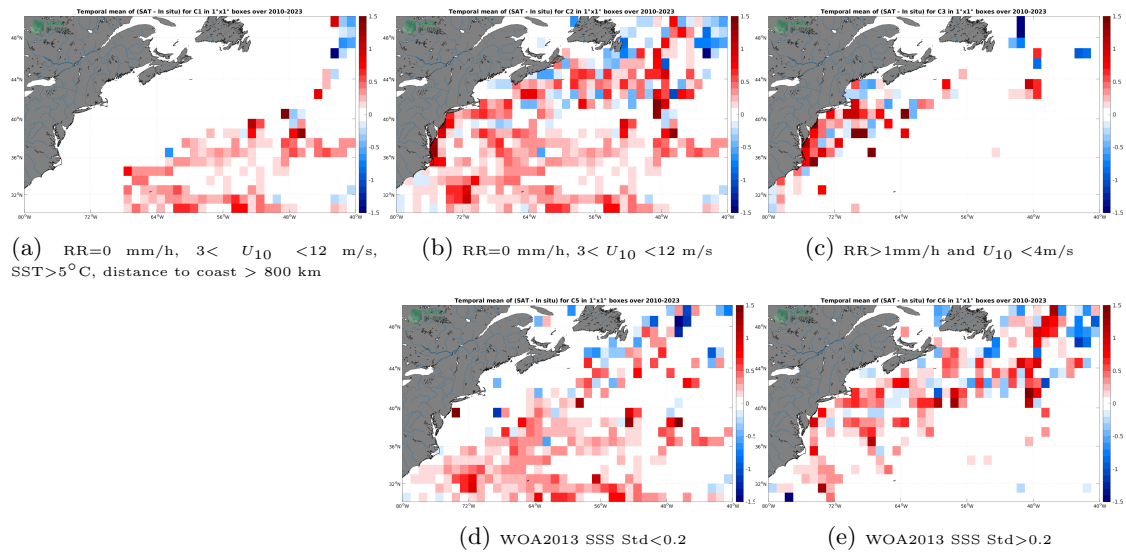
Figure 12: Temporal mean gridded over spatial boxes of size 1^\circ \times 1^\circ of \Delta SSS (SMOS SSS L3 v335 - Monthly - 25 km (CATDS-CPDC) - TSG (SAMOS)) for 5 different subdatasets corresponding to:RR=0 mm/h, 3 < U_{10} < 12 m/s, SST >5^\circ C, distance to coast > 800 km (a), RR=0 mm/h, 3 < U_{10} < 12 m/s (b), RR >1 mm/h and U_{10} < 4 m/s (c), WOA2013 SSS Std <0.2 (d), WOA2013 SSS Std >0.2 (e).
