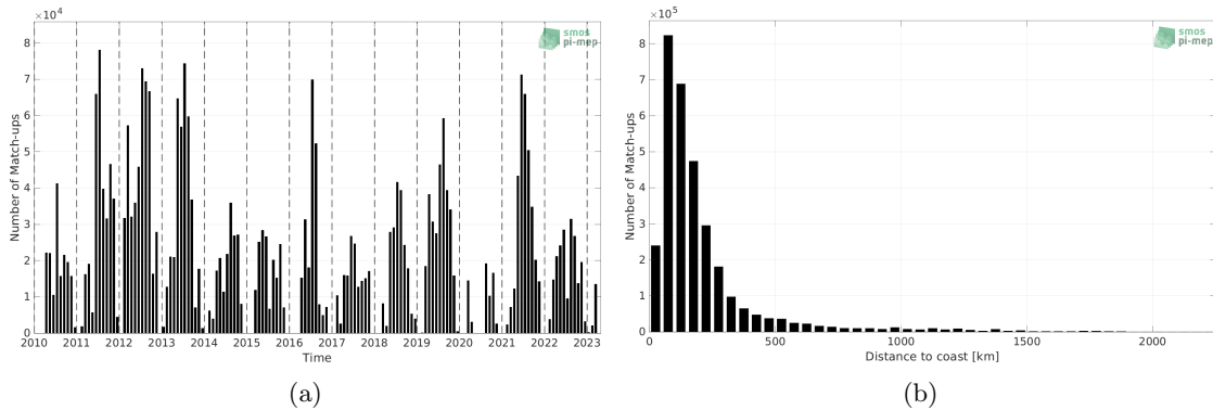
Figure 1: Number of match-ups between TSG (SAMOS) and SMOS SSS L3 v335 - Monthly - 25 km (CATDS-CPDC) SSS as a function of time (a) and as function of the distance to coast (b) over the Gulf Stream Pi-MEP region and for the full satellite product period.
