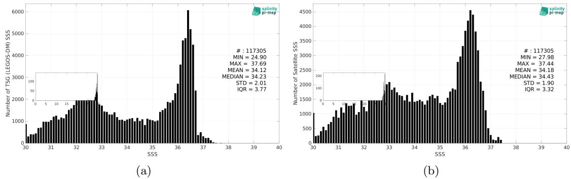
Figure 3: Histograms of SSS from TSG (LEGOS-DM) (a) and SMOS SSS L3 v335 - Monthly - 25 km (CATDS-CPDC) (b) considering all match-up pairs per bins of 0.1 over the Gulf Stream Pi-MEP region and for the full satellite product period.
