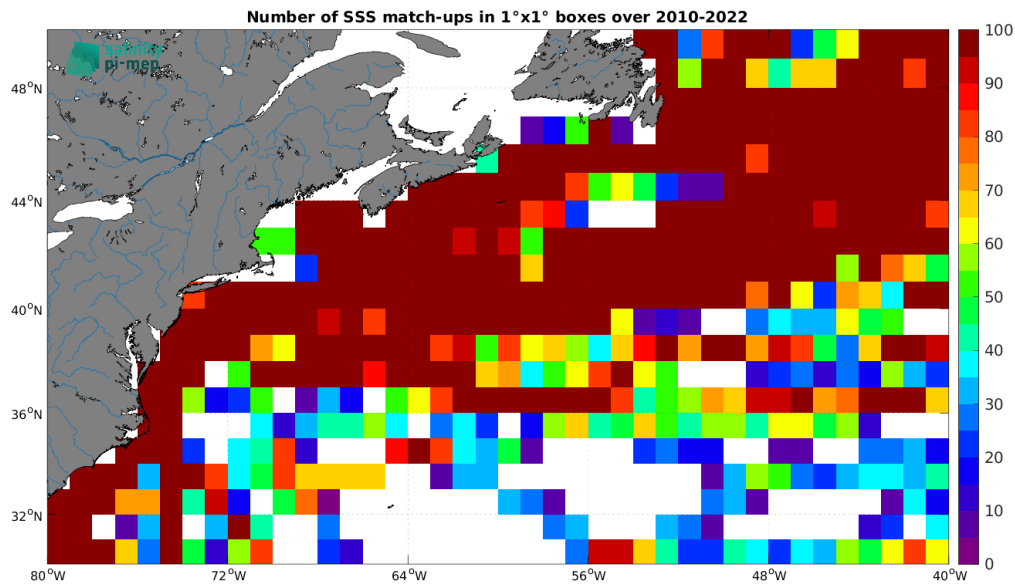
Figure 5: Number of SSS match-ups between TSG (LEGOS-DM) SSS and the SMOS SSS L3 v335 - Monthly - 25 km (CATDS-CPDC) SSS product for the Gulf Stream Pi-MEP region over 1^\circ \times 1^\circ boxes and for the full satellite product period.
