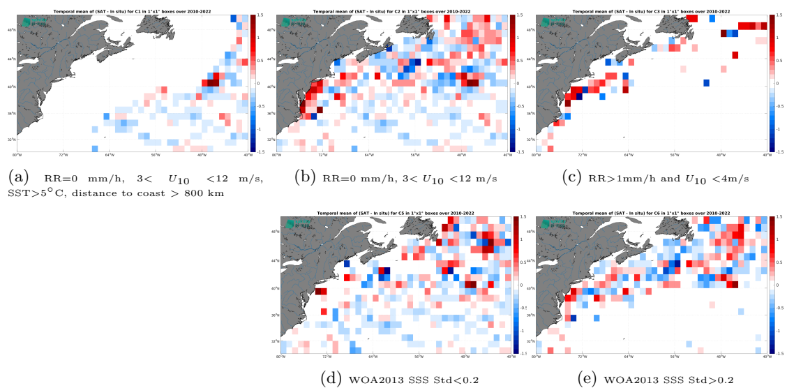
Figure 14: Temporal mean gridded over spatial boxes of size 1^\circ \times 1^\circ of \Delta SSS (SMOS SSS L3 v335 - Monthly - 25 km (CATDS-CPDC) - TSG (LEGOS-DM)) for 5 different subdatasets corresponding to:RR=0 mm/h, 3 < U_{10} < 12 m/s, SST >5^\circ C, distance to coast > 800 km (a), RR=0 mm/h, 3 < U_{10} < 12 m/s (b), RR >1 mm/h and U_{10} < 4 m/s (c), WOA2013 SSS Std <0.2 (d), WOA2013 SSS Std >0.2 (e).
