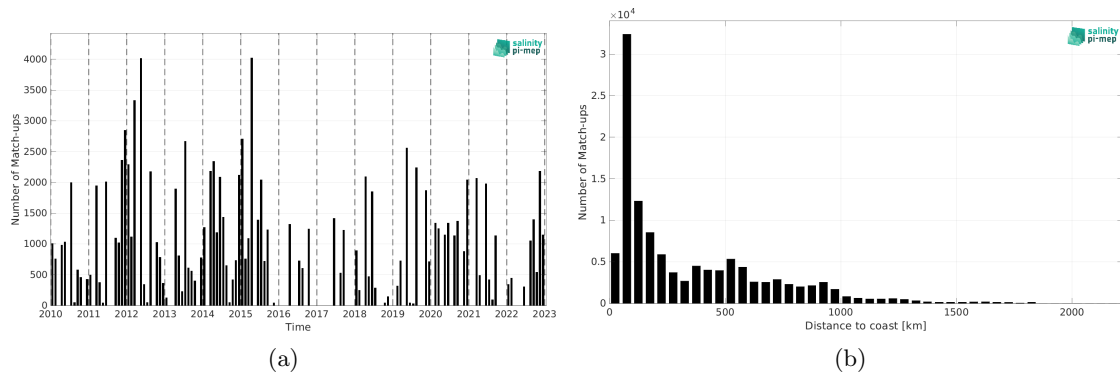
Figure 2: Number of match-ups between TSG (LEGOS-DM) and SMOS SSS L3 v335 - Monthly - 25 km (CATDS-CPDC) SSS as a function of time (a) and as function of the distance to coast (b) over the Gulf Stream Pi-MEP region and for the full satellite product period.
