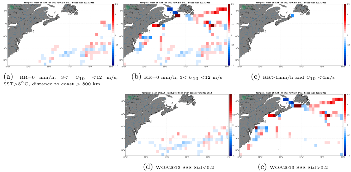
Figure 12: Temporal mean gridded over spatial boxes of size 1^{\circ}\times 1^{\circ} of \Delta SSS (SMOS SSS L3 v335 - Monthly - 25 km (CATDS-CPDC) - TSG (GOSUD-Sailing-ship)) for 5 different subdatasets corresponding to:RR=0 mm/h, 3 < U_{10} < 12 m/s, SST > 5^{\circ}\text{C} , distance to coast > 800 km (a), RR=0 mm/h, 3 < U_{10} < 12 m/s (b), RR > 1 mm/h and U_{10} < 4 m/s (c), WOA2013 SSS Std < 0.2 (d), WOA2013 SSS Std > 0.2 (e).
