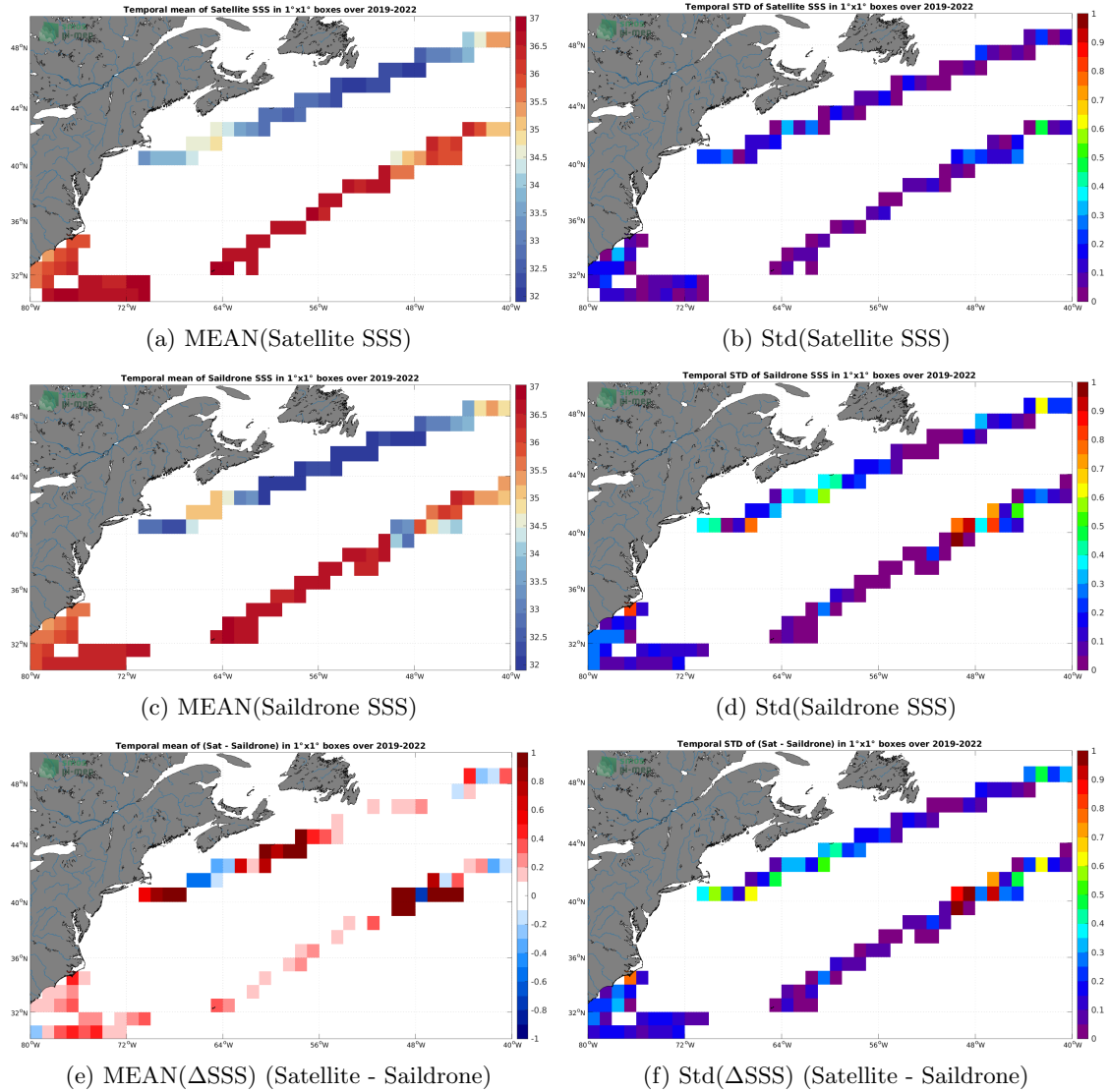
Figure 6: Temporal mean (left) and Std (right) of SSS from SMOS SSS L3 v335 - Monthly - 25 km (CATDS-CPDC) (top), Saildrone (middle), and of \Delta SSS (Satellite - Saildrone). Only match-up pairs are used to generate these maps.
