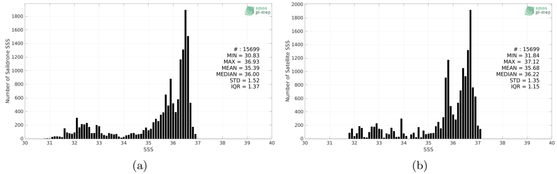
Figure 2: Histograms of SSS from Sairdrone (a) and SMOS SSS L3 v335 - Monthly - 25 km (CATDS-CPDC) (b) considering all match-up pairs per bins of 0.1 over the Gulf Stream Pi-MEP region and for the full satellite product period.
