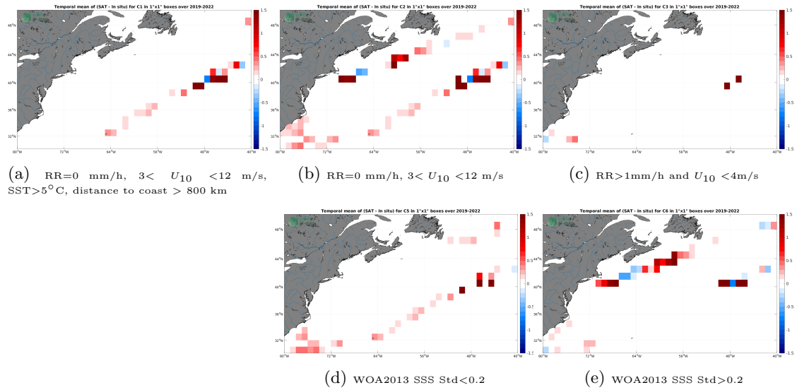
Figure 12: Temporal mean gridded over spatial boxes of size 1^\circ \times 1^\circ of \Delta SSS (SMOS SSS L3 v335 - Monthly - 25 km (CATDS-CPDC) - Saildrone) for 5 different subdatasets corresponding to:RR=0 mm/h, 3 < U_{10} < 12 m/s, SST >5^\circ C, distance to coast > 800 km (a), RR=0 mm/h, 3 < U_{10} < 12 m/s (b), RR >1 mm/h and U_{10} < 4 m/s (c), WOA2013 SSS Std <0.2 (d), WOA2013 SSS Std >0.2 (e).
