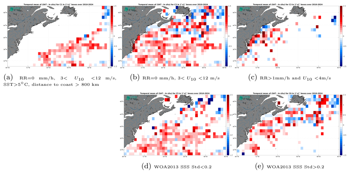
Figure 14: Temporal mean gridded over spatial boxes of size 1^\circ \times 1^\circ of \Delta SSS (SMOS SSS L3 v335 - 10 Days - 25 km (CATDS-CPDC) - TSG (SAMOS)) for 5 different subdatasets corresponding to: RR=0 mm/h, 3 < U_{10} < 12 m/s, SST > 5°C, distance to coast > 800 km (a), RR=0 mm/h, 3 < U_{10} < 12 m/s (b), RR > 1mm/h and U_{10} < 4 m/s (c), WOA2013 SSS Std < 0.2 (d), WOA2013 SSS Std > 0.2 (e).
