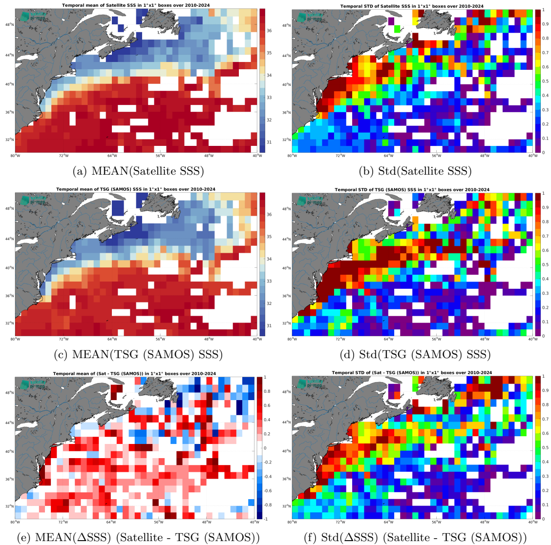
Figure 7: Temporal mean (left) and Std (right) of SSS from SMOS SSS L3 v335 - 10 Days - 25 km (CATDS-CPDC) (top), TSG (SAMOS) (middle), and of \Delta SSS (Satellite - TSG (SAMOS)). Only match-up pairs are used to generate these maps.
