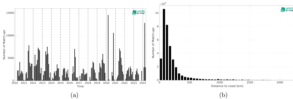
Figure 2: Number of match-ups between TSG (SAMOS) and SMOS SSS L3 v335 - 10 Days - 25 km (CATDS-CPDC) SSS as a function of time (a) and as function of the distance to coast (b) over the Gulf Stream Pi-MEP region and for the full satellite product period.
