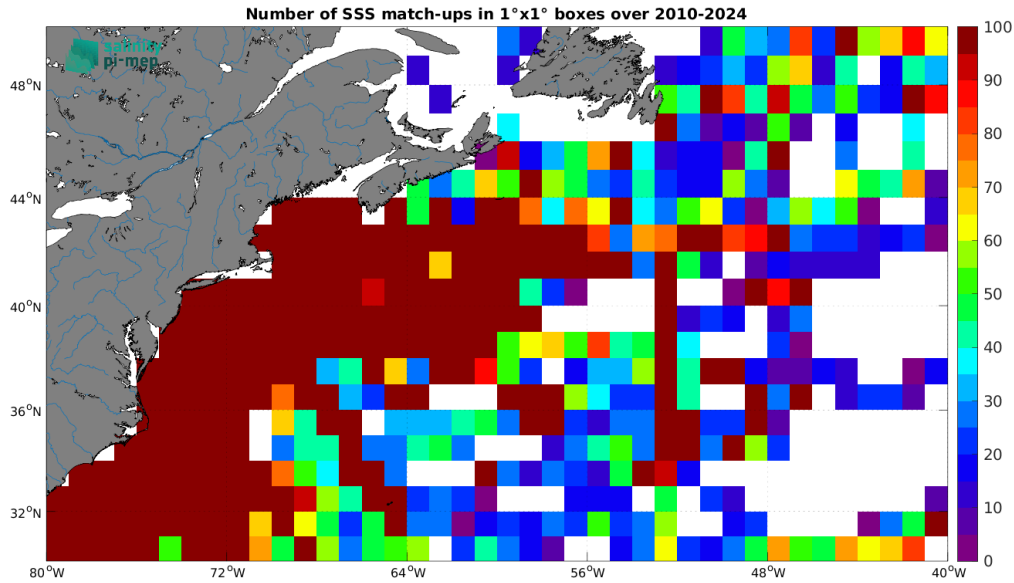
Figure 5: Number of SSS match-ups between TSG (SAMOS) SSS and the SMOS SSS L3 v335 - 10 Days - 25 km (CATDS-CPDC) SSS product for the Gulf Stream Pi-MEP region over 1^{\circ} \times 1^{\circ} boxes and for the full satellite product period.
