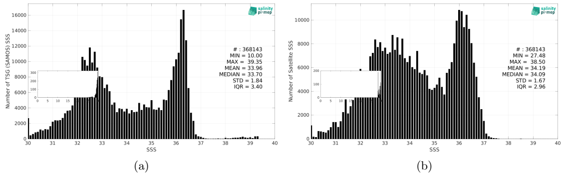
Figure 3: Histograms of SSS from TSG (SAMOS) (a) and SMOS SSS L3 v335 - 10 Days - 25 km (CATDS-CPDC) (b) considering all match-up pairs per bins of 0.1 over the Gulf Stream Pi-MEP region and for the full satellite product period.
