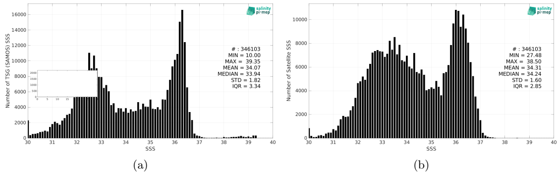
Figure 2: Histograms of SSS from TSG (SAMOS) (a) and SMOS SSS L3 v335 - 10 Days - 25 km (CATDS-CPDC) (b) considering all match-up pairs per bins of 0.1 over the Gulf Stream Pi-MEP region and for the full satellite product period.
