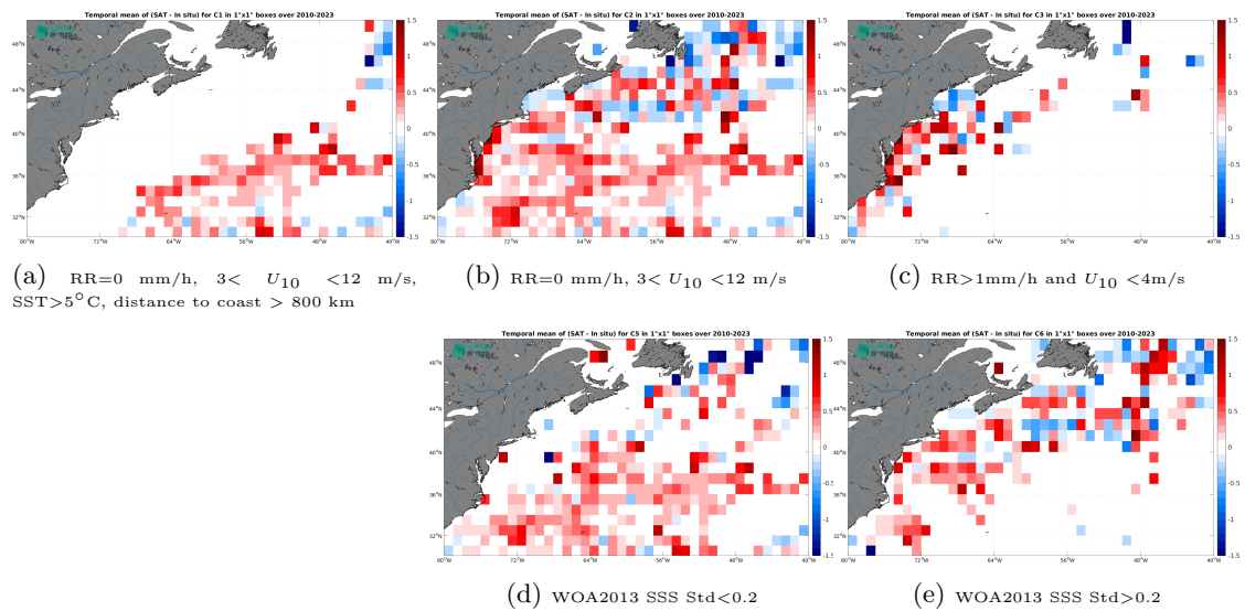
Figure 12: Temporal mean gridded over spatial boxes of size 1^\circ \times 1^\circ of \Delta\text{SSS} (SMOS SSS L3 v335 - 10 Days - 25 km (CATDS-CPDC) - TSG (SAMOS)) for 5 different subdatasets corresponding to:RR=0 mm/h, 3 < U_{10} < 12 m/s, SST >5^\circ\text{C} , distance to coast > 800 km (a), RR=0 mm/h, 3 < U_{10} < 12 m/s (b), RR >1 mm/h and U_{10} < 4 m/s (c), WOA2013 SSS Std <0.2 (d), WOA2013 SSS Std >0.2 (e).
