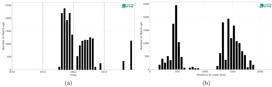
Figure 2: Number of match-ups between Surface drifters and SMOS SSS L3 v335 - 10 Days - 25 km (CATDS-CPDC) SSS as a function of time (a) and as function of the distance to coast (b) over the Gulf Stream Pi-MEP region and for the full satellite product period.
