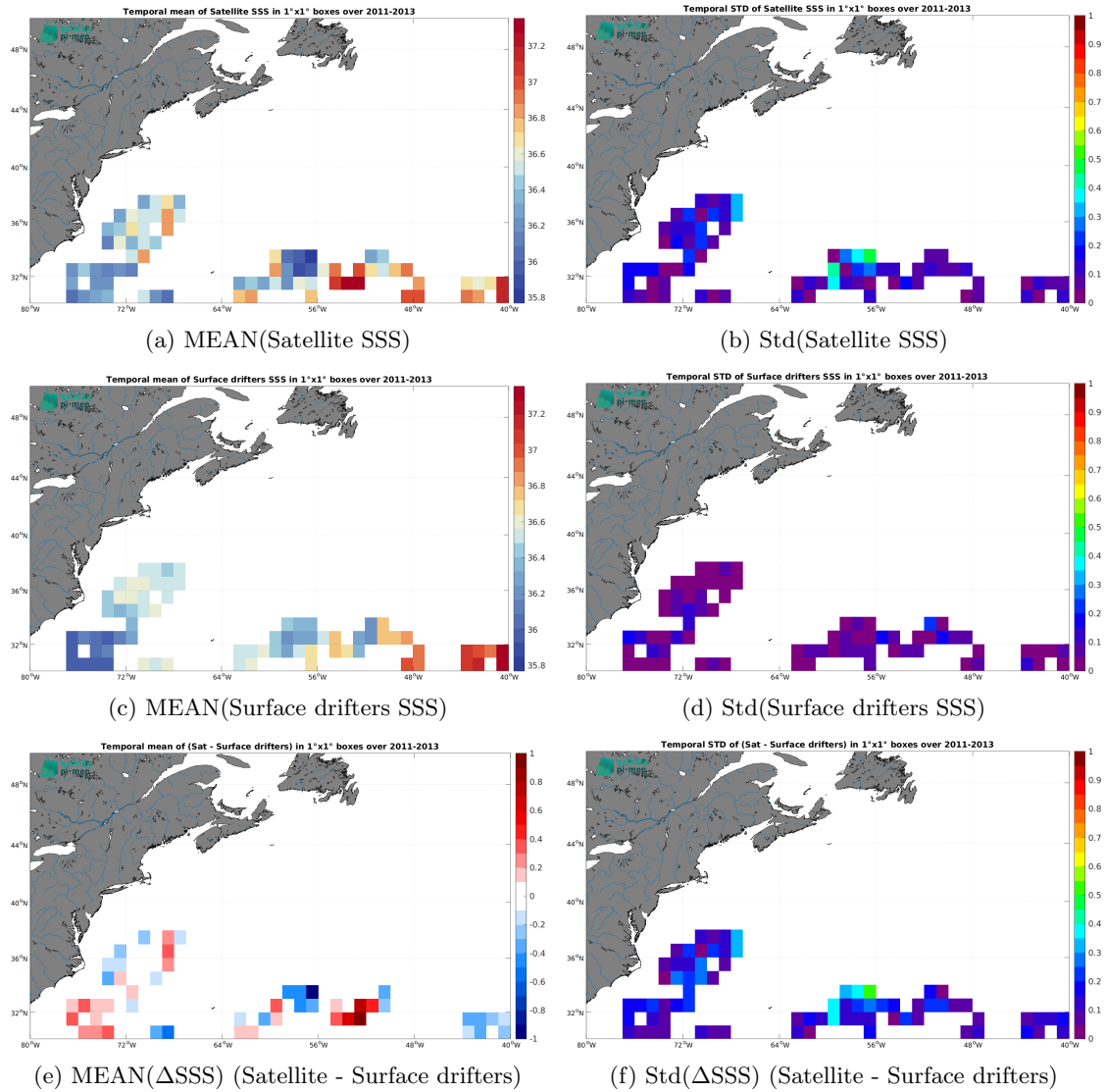
Figure 6: Temporal mean (left) and Std (right) of SSS from SMOS SSS L3 v335 - 10 Days - 25 km (CATDS-CPDC) (top), Surface drifters (middle), and of \Delta SSS (Satellite - Surface drifters). Only match-up pairs are used to generate these maps.
