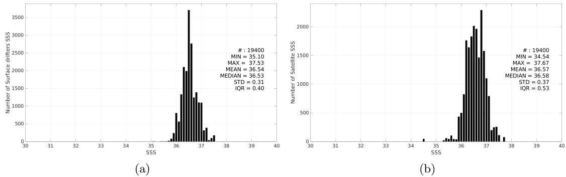
Figure 3: Histograms of SSS from Surface drifters (a) and SMOS SSS L3 v335 - 10 Days - 25 km (CATDS-CPDC) (b) considering all match-up pairs per bins of 0.1 over the Gulf Stream Pi-MEP region and for the full satellite product period.
