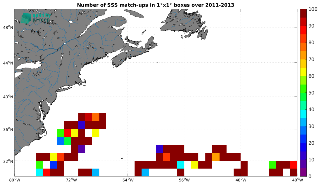
Figure 4: Number of SSS match-ups between Surface drifters SSS and the SMOS SSS L3 v335 - 10 Days - 25 km (CATDS-CPDC) SSS product for the Gulf Stream Pi-MEP region over 1^\circ \times 1^\circ boxes and for the full satellite product period.
