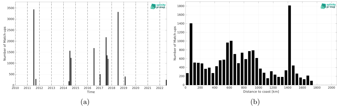
Figure 2: Number of match-ups between TSG (GOSUD-Research-vessel) and SMOS SSS L2Q v333 - 0.25 Deg (CATDS-CPDC) SSS as a function of time (a) and as function of the distance to coast (b) over the Gulf Stream Pi-MEP region and for the full satellite product period.
