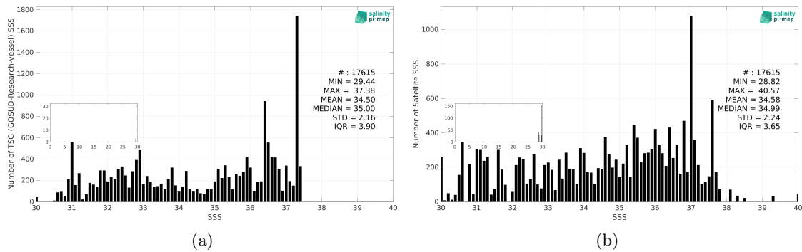
Figure 3: Histograms of SSS from TSG (GOSUD-Research-vessel) (a) and SMOS SSS L2Q v333 - 0.25 Deg (CATDS-CPDC) (b) considering all match-up pairs per bins of 0.1 over the Gulf Stream Pi-MEP region and for the full satellite product period.
