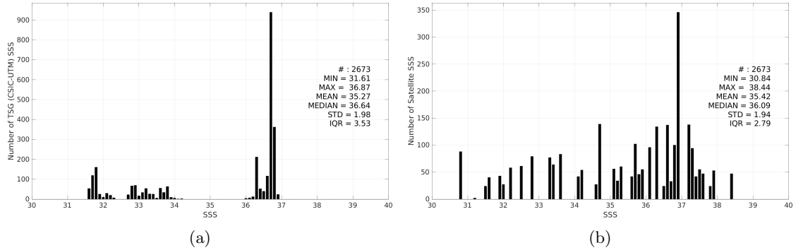
Figure 3: Histograms of SSS from TSG (CSIC-UTM) (a) and SMOS SSS L2Q v333 - 0.25 Deg (CATDS-CPDC) (b) considering all match-up pairs per bins of 0.1 over the Gulf Stream Pi-MEP region and for the full satellite product period.
