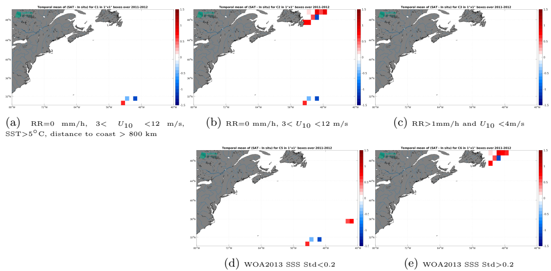
Figure 14: Temporal mean gridded over spatial boxes of size 1^\circ \times 1^\circ of \Delta SSS (SMOS SSS L2Q v333 - 0.25 Deg (CATDS-CPDC) - TSG (CSIC-UTM)) for 5 different subdatasets corresponding to: RR=0 mm/h, 3 < U_{10} < 12 m/s, SST > 5°C, distance to coast > 800 km (a), RR=0 mm/h, 3 < U_{10} < 12 m/s (b), RR > 1mm/h and U_{10} < 4 m/s (c), WOA2013 SSS Std < 0.2 (d), WOA2013 SSS Std > 0.2 (e).
