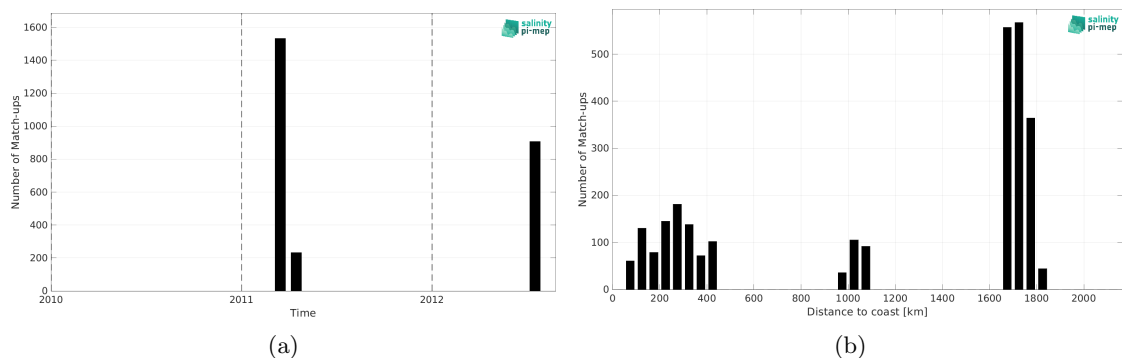
Figure 2: Number of match-ups between TSG (CSIC-UTM) and SMOS SSS L2Q v333 - 0.25 Deg (CATDS-CPDC) SSS as a function of time (a) and as function of the distance to coast (b) over the Gulf Stream Pi-MEP region and for the full satellite product period.
