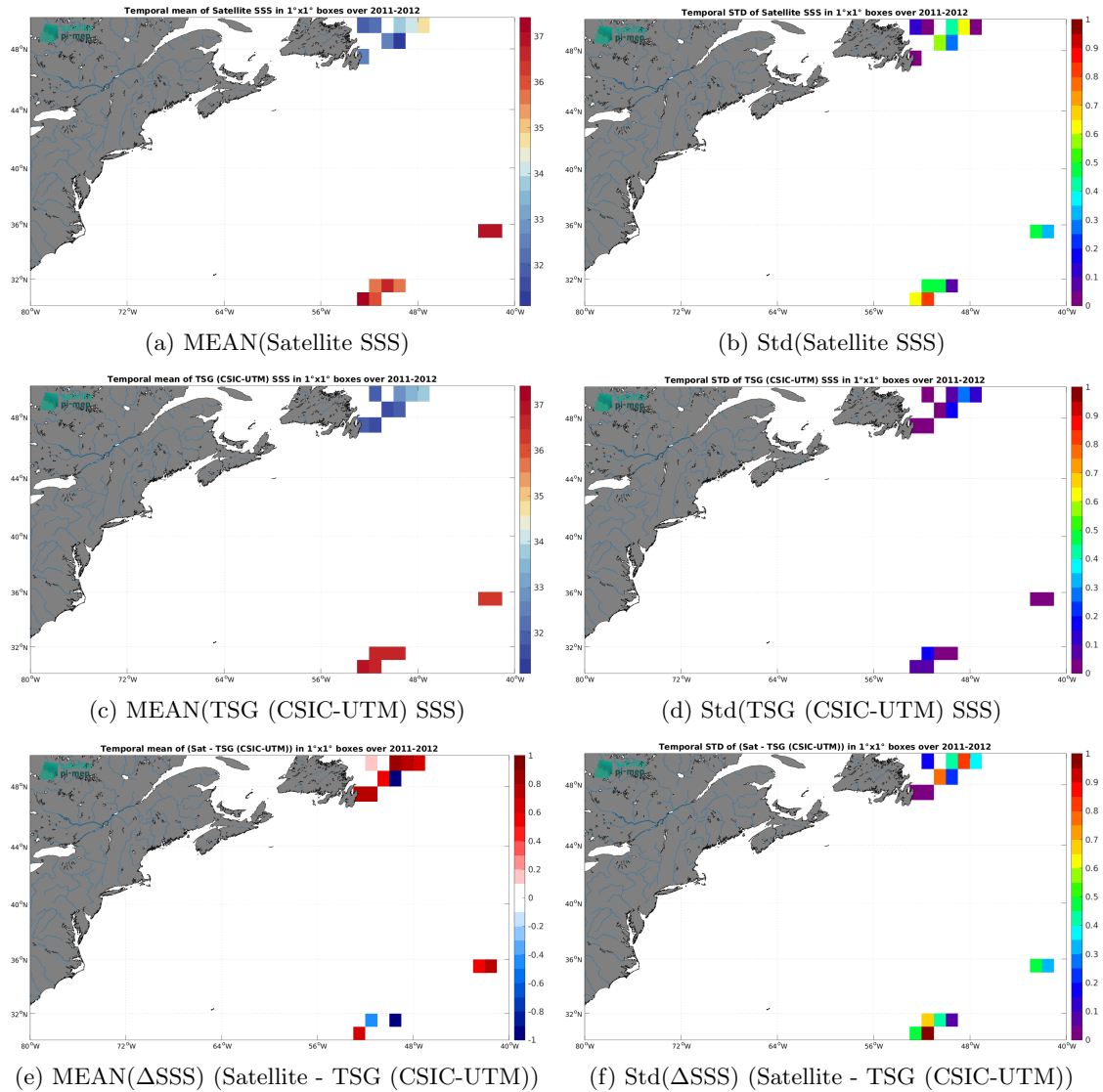
Figure 7: Temporal mean (left) and Std (right) of SSS from SMOS SSS L2Q v333 - 0.25 Deg (CATDS-CPDC) (top), TSG (CSIC-UTM) (middle), and of \Delta SSS (Satellite - TSG (CSIC-UTM)). Only match-up pairs are used to generate these maps.
