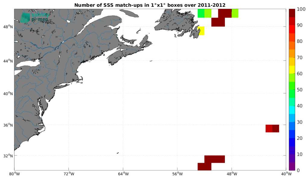
Figure 5: Number of SSS match-ups between TSG (CSIC-UTM) SSS and the SMOS SSS L2Q v333 - 0.25 Deg (CATDS-CPDC) SSS product for the Gulf Stream Pi-MEP region over 1°x1° boxes and for the full satellite product period.
