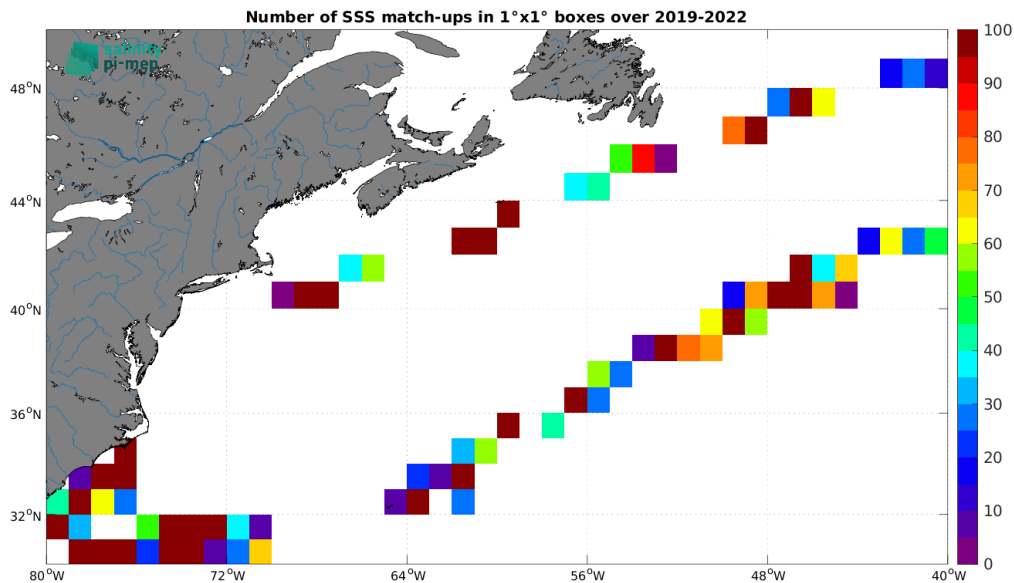
Figure 5: Number of SSS match-ups between Salldrone SSS and the SMOS SSS L2Q v333 - 0.25 Deg (CATDS-CPDC) SSS product for the Gulf Stream Pi-MEP region over 1^\circ \times 1^\circ boxes and for the full satellite product period.
