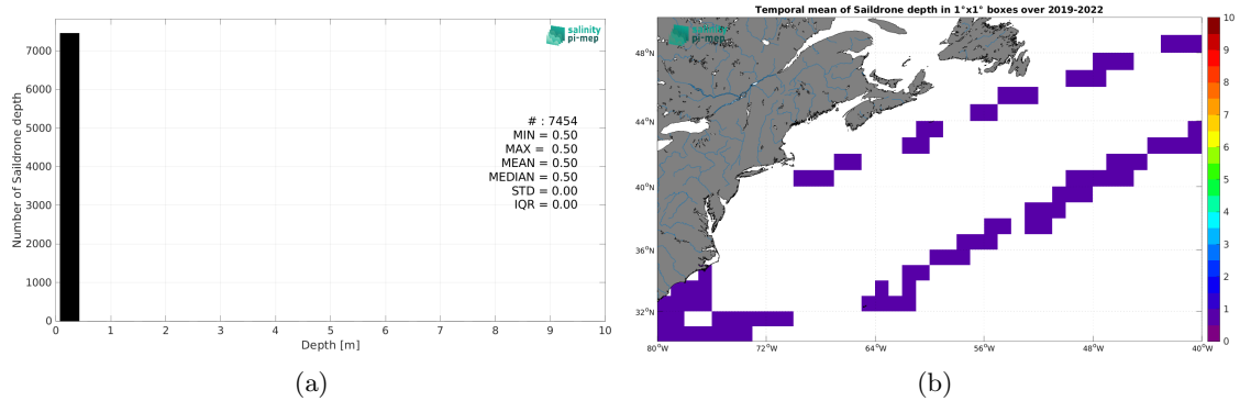
Figure 4: Histograms of the depth of the upper level SSS measurements from Salldrone in the Match-up DataBase for the Gulf Stream Pi-MEP region (a) and temporal mean spatial distribution of pressure of the in situ SSS data over 1^\circ \times 1^\circ boxes and for the full satellite product period (b).
