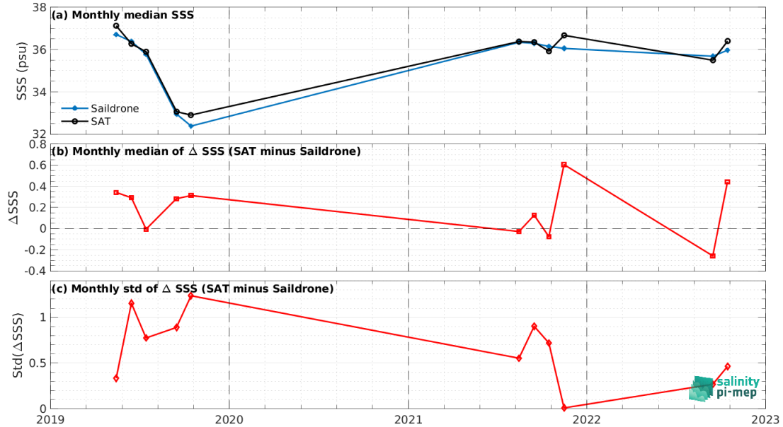
Figure 8: Time series of the monthly median SSS (top), median of \Delta SSS (Satellite - Saildrone) and Std of \Delta SSS (Satellite - Saildrone) over the Gulf Stream Pi-MEP region considering all match-ups collected by the Pi-MEP.
