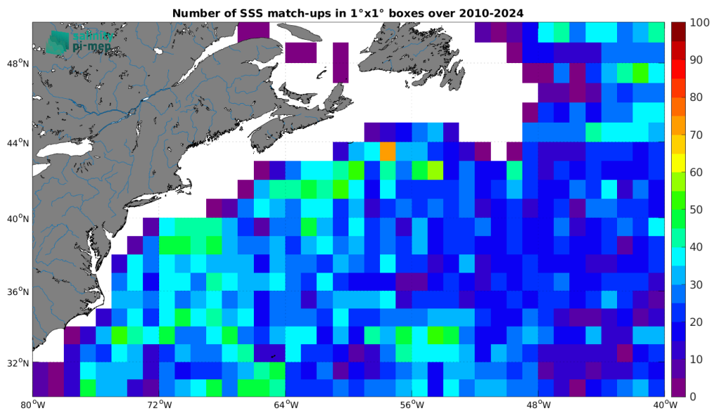
Figure 5: Number of SSS match-ups between Argo SSS and the SMOS SSS L2Q v333 - 0.25 Deg (CATDS-CPDC) SSS product for the Gulf Stream Pi-MEP region over 1^\circ \times 1^\circ boxes and for the full satellite product period.
