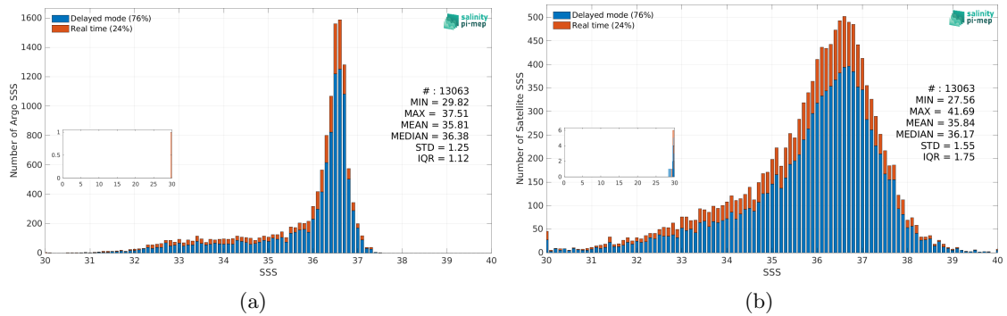
Figure 3: Histograms of SSS from Argo (a) and SMOS SSS L2Q v333 - 0.25 Deg (CATDS-CPDC) (b) considering all match-up pairs per bins of 0.1 over the Gulf Stream Pi-MEP region and for the full satellite product period.
