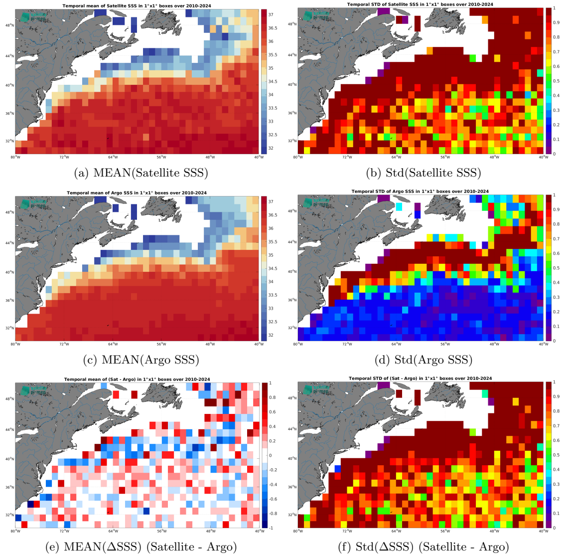
Figure 7: Temporal mean (left) and Std (right) of SSS from SMOS SSS L2Q v333 - 0.25 Deg (CATDS-CPDC) (top), Argo (middle), and of \Delta SSS (Satellite - Argo). Only match-up pairs are used to generate these maps.
