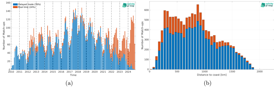
Figure 2: Number of match-ups between Argo and SMOS SSS L2Q v333 - 0.25 Deg (CATDS-CPDC) SSS as a function of time (a) and as function of the distance to coast (b) over the Gulf Stream Pi-MEP region and for the full satellite product period.
