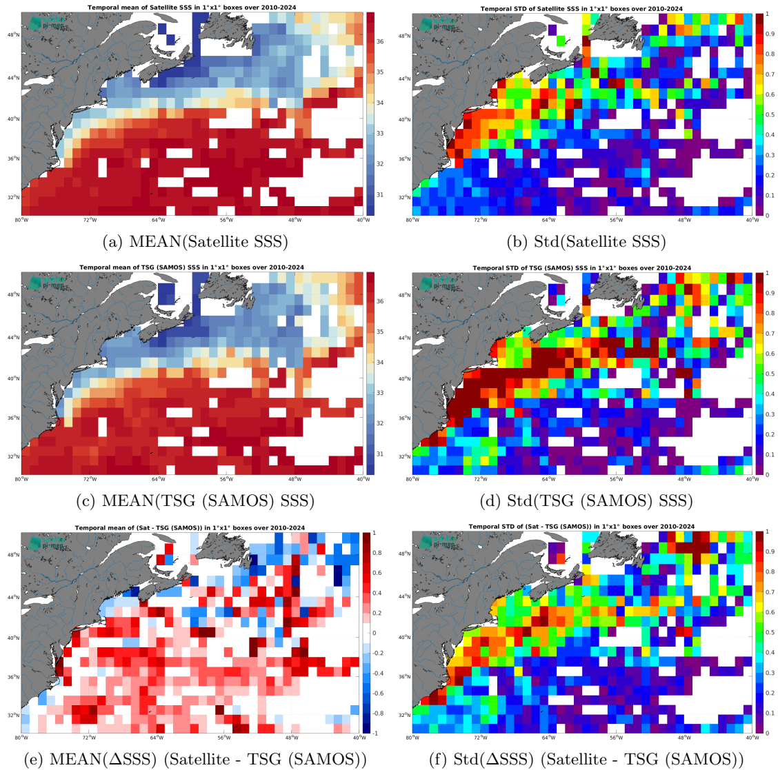
Figure 7: Temporal mean (left) and Std (right) of SSS from SMOS SSS L3 v332 - 9 Days (CATDS-CPDC) (top), TSG (SAMOS) (middle), and of \Delta SSS (Satellite - TSG (SAMOS)). Only match-up pairs are used to generate these maps.
