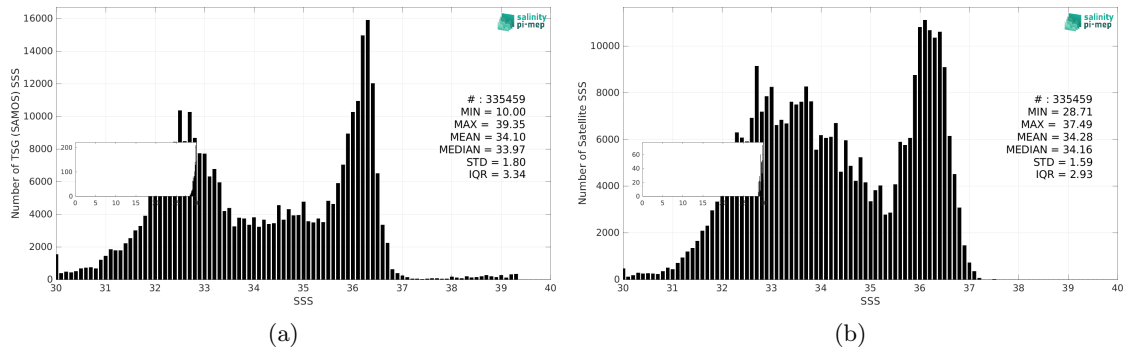
Figure 3: Histograms of SSS from TSG (SAMOS) (a) and SMOS SSS L3 v332 - 9 Days (CATDS-CPDC) (b) considering all match-up pairs per bins of 0.1 over the Gulf Stream Pi-MEP region and for the full satellite product period.
