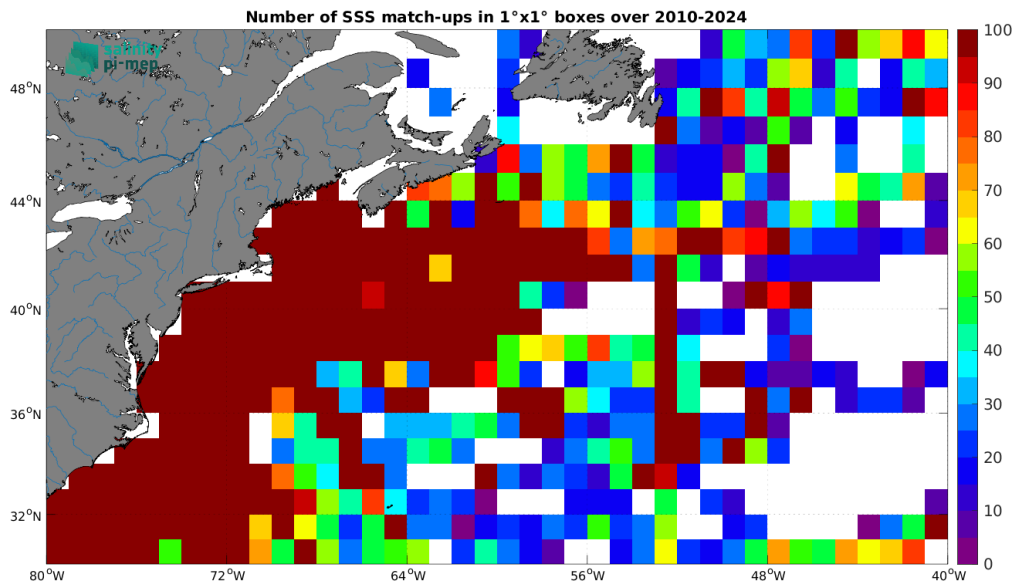
Figure 5: Number of SSS match-ups between TSG (SAMOS) SSS and the SMOS SSS L3 v332 - 9 Days (CATDS-CPDC) SSS product for the Gulf Stream Pi-MEP region over 1^\circ \times 1^\circ boxes and for the full satellite product period.
