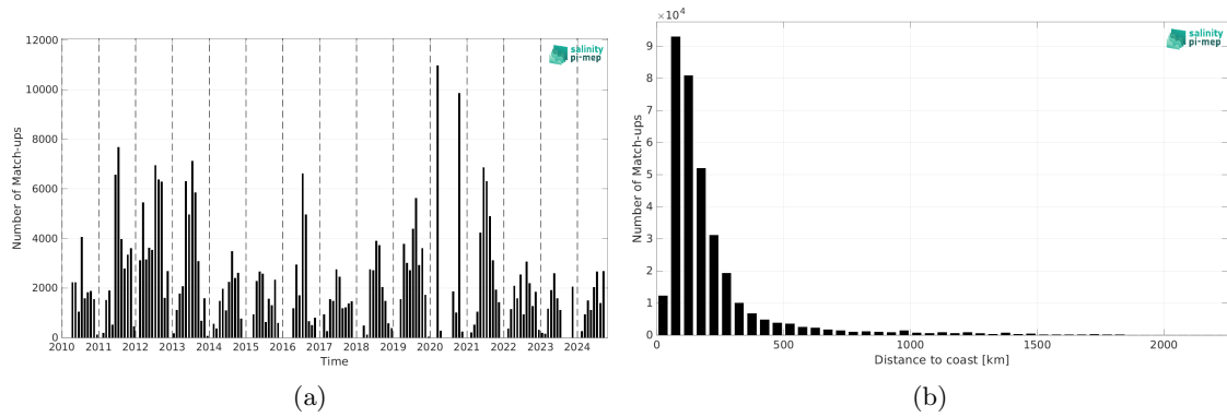
Figure 2: Number of match-ups between TSG (SAMOS) and SMOS SSS L3 v332 - 9 Days (CATDS-CPDC) SSS as a function of time (a) and as function of the distance to coast (b) over the Gulf Stream Pi-MEP region and for the full satellite product period.
