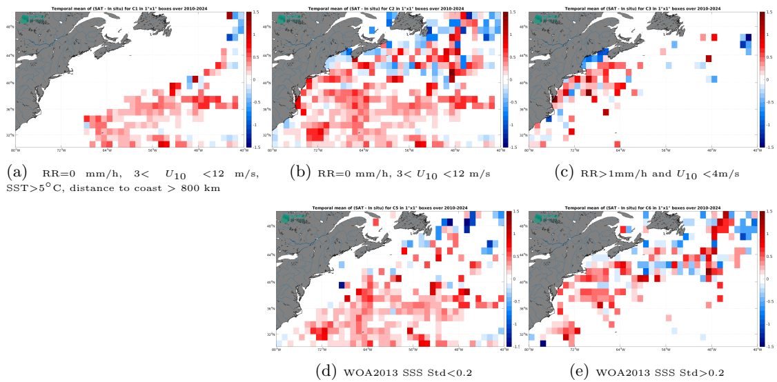
Figure 14: Temporal mean gridded over spatial boxes of size 1^\circ \times 1^\circ of \Delta SSS (SMOS SSS L3 v332 - 9 Days (CATDS-CPDC) - TSG (SAMOS)) for 5 different subdatasets corresponding to:RR=0 mm/h, 3 < U_{10} < 12 m/s, SST>5°C, distance to coast > 800 km (a), RR=0 mm/h, 3 < U_{10} < 12 m/s (b), RR>1mm/h and U_{10} < 4 m/s (c), WOA2013 SSS Std<0.2 (d), WOA2013 SSS Std>0.2 (e).
