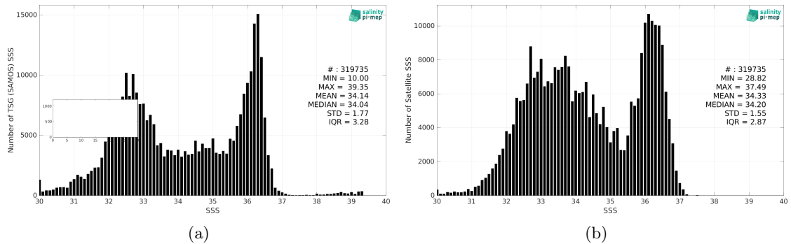
Figure 2: Histograms of SSS from TSG (SAMOS) (a) and SMOS SSS L3 v332 - 9 Days (CATDS-CPDC) (b) considering all match-up pairs per bins of 0.1 over the Gulf Stream Pi-MEP region and for the full satellite product period.
