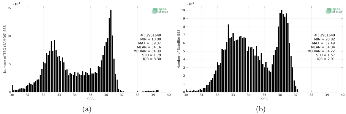
Figure 2: Histograms of SSS from TSG (SAMOS) (a) and SMOS SSS L3 v332 - 9 Days (CATDS-CPDC) (b) considering all match-up pairs per bins of 0.1 over the Gulf Stream Pi-MEP region and for the full satellite product period.
