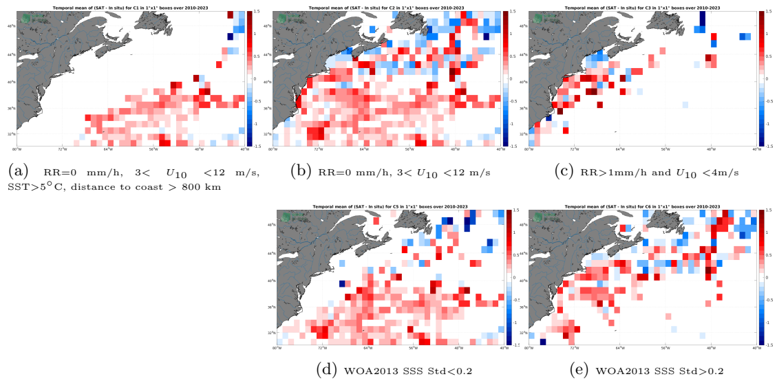
Figure 12: Temporal mean gridded over spatial boxes of size 1^\circ \times 1^\circ of \Delta SSS (SMOS SSS L3 v332 - 9 Days (CATDS-CPDC) - TSG (SAMOS)) for 5 different subdatasets corresponding to:RR=0 mm/h, 3 < U_{10} < 12 m/s, SST >5^\circ C, distance to coast > 800 km (a), RR=0 mm/h, 3 < U_{10} < 12 m/s (b), RR >1 mm/h and U_{10} < 4 m/s (c), WOA2013 SSS Std <0.2 (d), WOA2013 SSS Std >0.2 (e).
