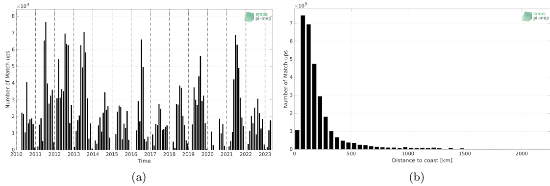
Figure 1: Number of match-ups between TSG (SAMOS) and SMOS SSS L3 v332 - 9 Days (CATDS-CPDC) SSS as a function of time (a) and as function of the distance to coast (b) over the Gulf Stream Pi-MEP region and for the full satellite product period.
