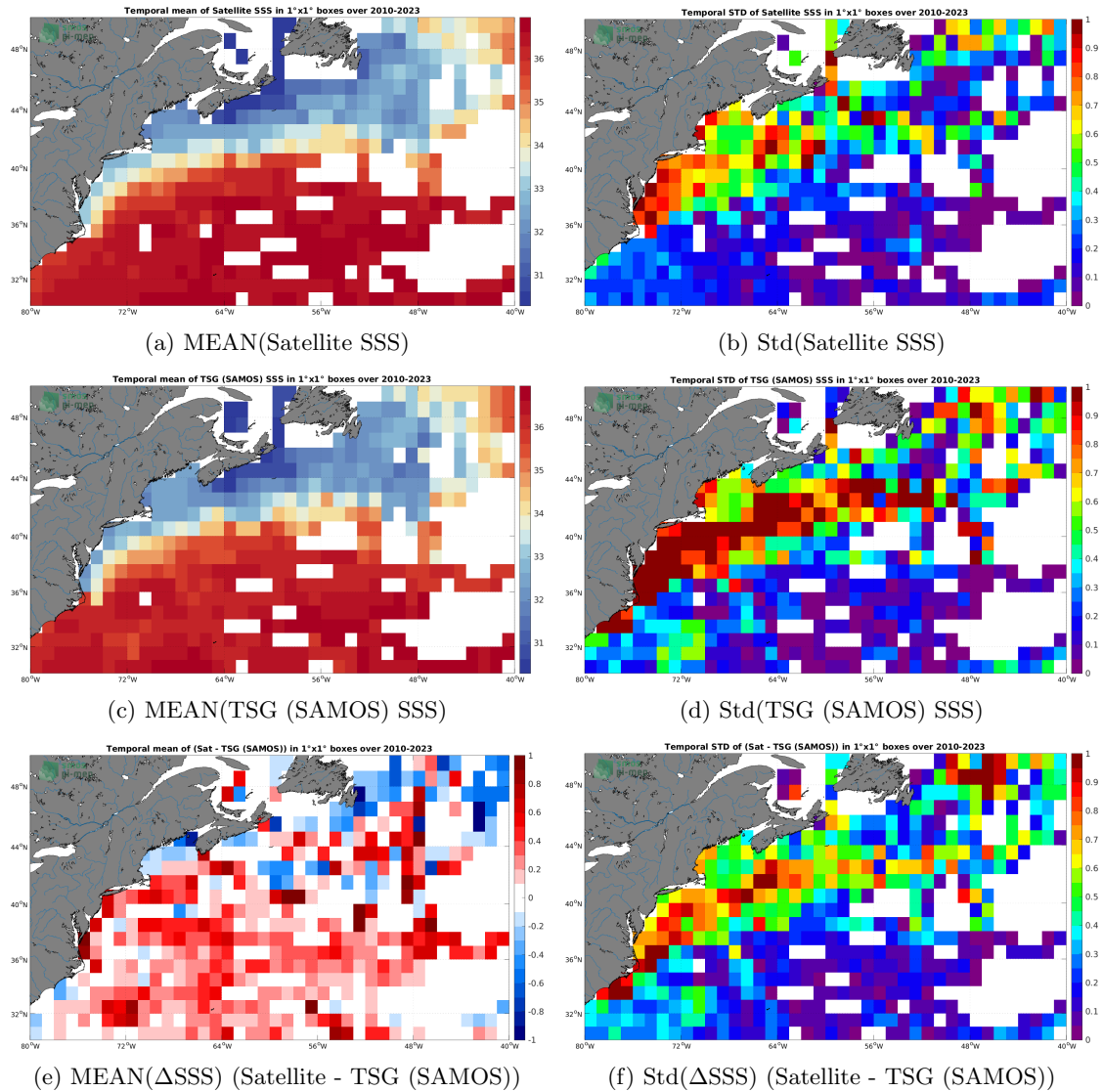
Figure 6: Temporal mean (left) and Std (right) of SSS from SMOS SSS L3 v332 - 9 Days (CATDS-CPDC) (top), TSG (SAMOS) (middle), and of \Delta SSS (Satellite - TSG (SAMOS)). Only match-up pairs are used to generate these maps.
