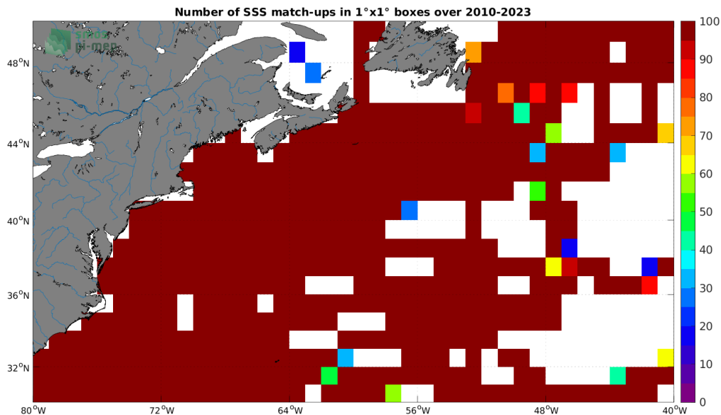
Figure 4: Number of SSS match-ups between TSG (SAMOS) SSS and the SMOS SSS L3 v332 - 9 Days (CATDS-CPDC) SSS product for the Gulf Stream Pi-MEP region over 1^\circ \times 1^\circ boxes and for the full satellite product period.
