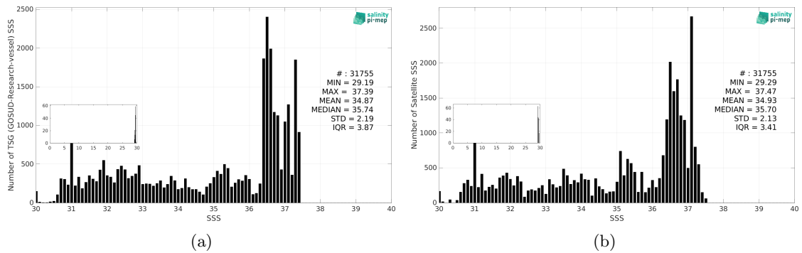
Figure 3: Histograms of SSS from TSG (GOSUD-Research-vessel) (a) and SMOS SSS L3 v332 - 9 Days (CATDS-CPDC) (b) considering all match-up pairs per bins of 0.1 over the Gulf Stream Pi-MEP region and for the full satellite product period.
