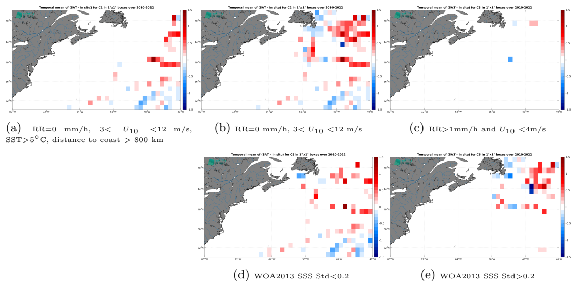
Figure 14: Temporal mean gridded over spatial boxes of size 1^\circ \times 1^\circ of \Delta SSS (SMOS SSS L3 v332 - 9 Days (CATDS-CPDC) - TSG (GOSUD-Research-vessel)) for 5 different subdatasets corresponding to:RR=0 mm/h, 3 < U_{10} < 12 m/s, SST >5^\circ\text{C} , distance to coast > 800 km (a), RR=0 mm/h, 3 < U_{10} < 12 m/s (b), RR >1 mm/h and U_{10} < 4 m/s (c), WOA2013 SSS Std <0.2 (d), WOA2013 SSS Std >0.2 (e).
