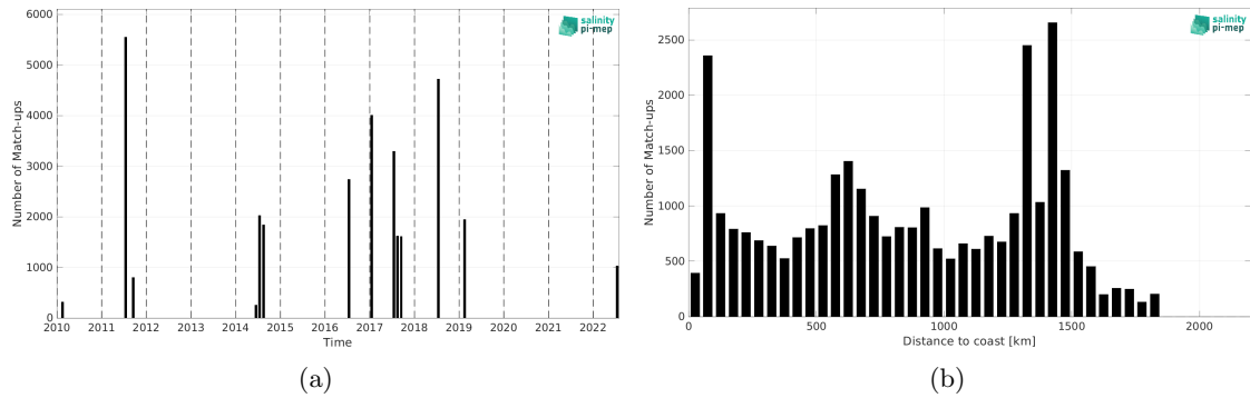
Figure 2: Number of match-ups between TSG (GOSUD-Research-vessel) and SMOS SSS L3 v332 - 9 Days (CATDS-CPDC) SSS as a function of time (a) and as function of the distance to coast (b) over the Gulf Stream Pi-MEP region and for the full satellite product period.
