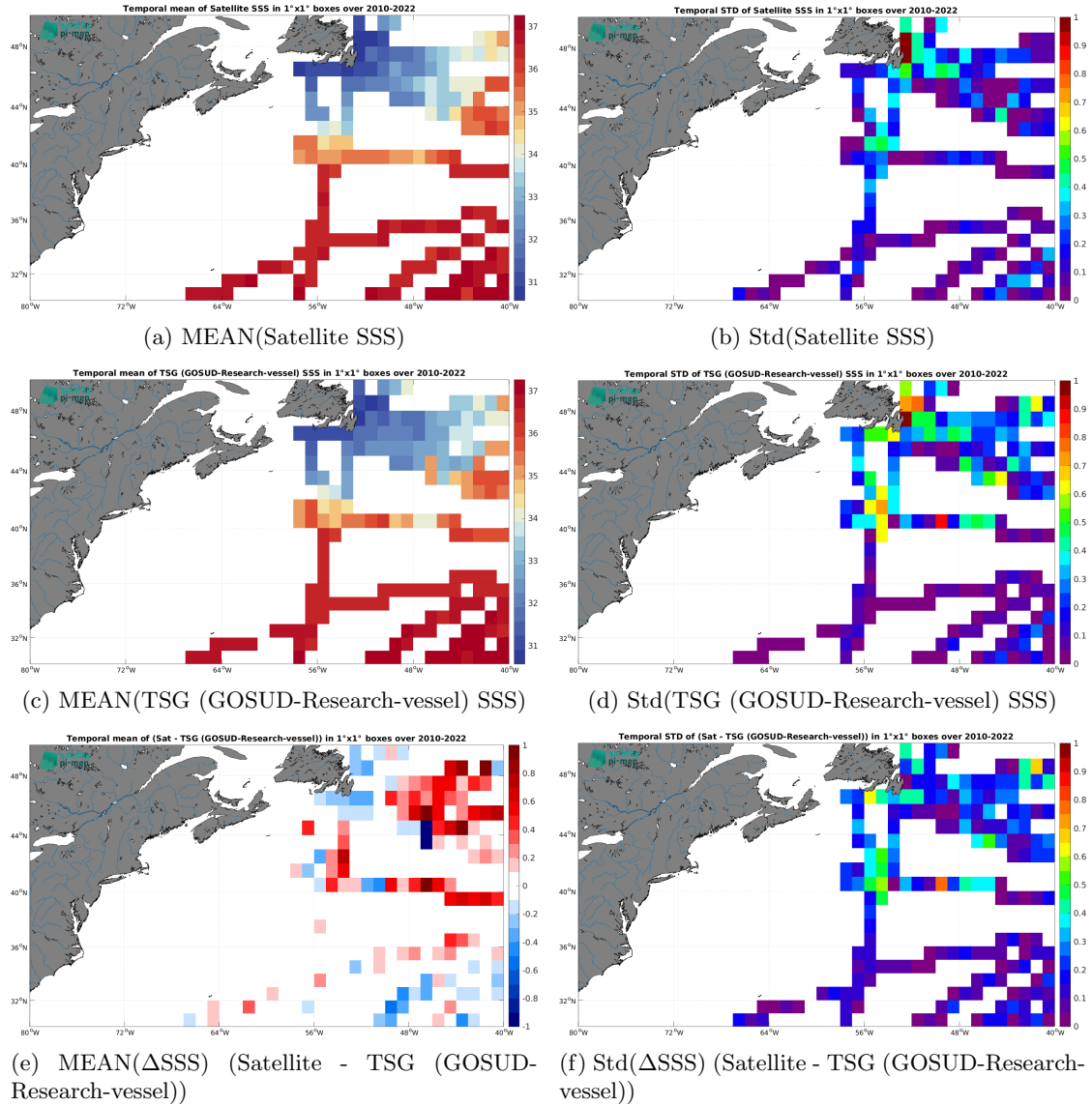
Figure 7: Temporal mean (left) and Std (right) of SSS from SMOS SSS L3 v332 - 9 Days (CATDS-CPDC) (top), TSG (GOSUD-Research-vessel) (middle), and of \Delta SSS (Satellite - TSG (GOSUD-Research-vessel)). Only match-up pairs are used to generate these maps.
