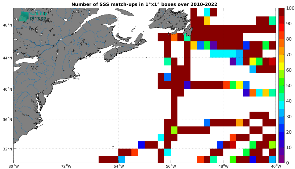
Figure 5: Number of SSS match-ups between TSG (GOSUD-Research-vessel) SSS and the SMOS SSS L3 v332 - 9 Days (CATDS-CPDC) SSS product for the Gulf Stream Pi-MEP region over 1^\circ \times 1^\circ boxes and for the full satellite product period.
