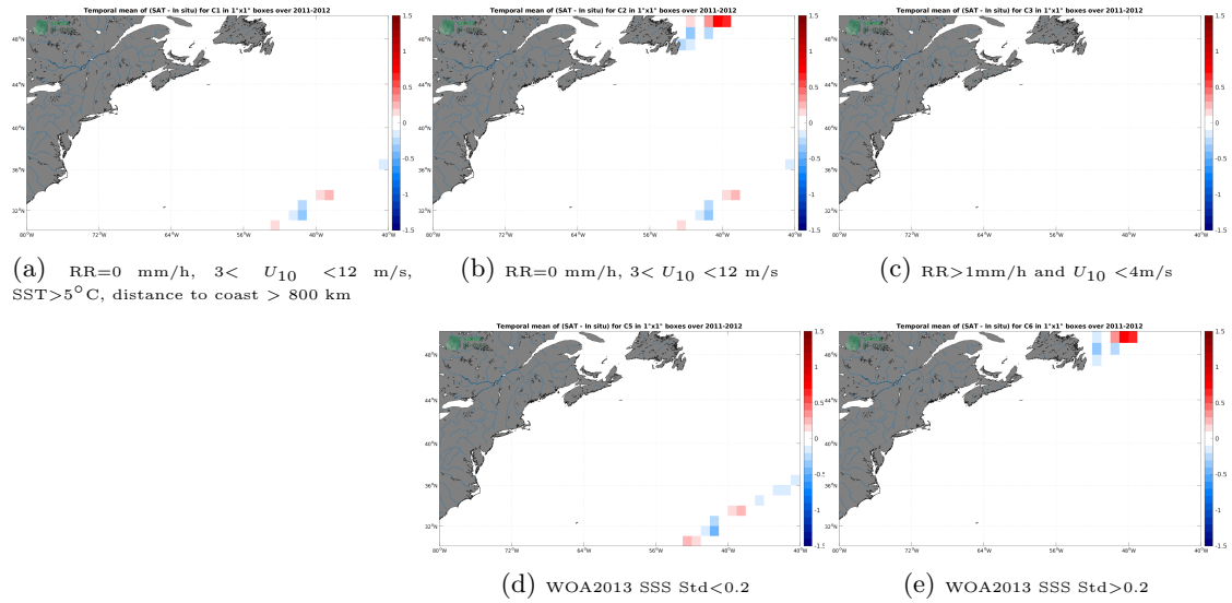
Figure 12: Temporal mean gridded over spatial boxes of size 1^\circ \times 1^\circ of \Delta SSS (SMOS SSS L3 v332 - 9 Days (CATDS-CPDC) - TSG (CSIC-UTM)) for 5 different subdatasets corresponding to:RR=0 mm/h, 3 < U_{10} < 12 m/s, SST >5^\circ C, distance to coast > 800 km (a), RR=0 mm/h, 3 < U_{10} < 12 m/s (b), RR >1 mm/h and U_{10} < 4 m/s (c), WOA2013 SSS Std <0.2 (d), WOA2013 SSS Std >0.2 (e).
