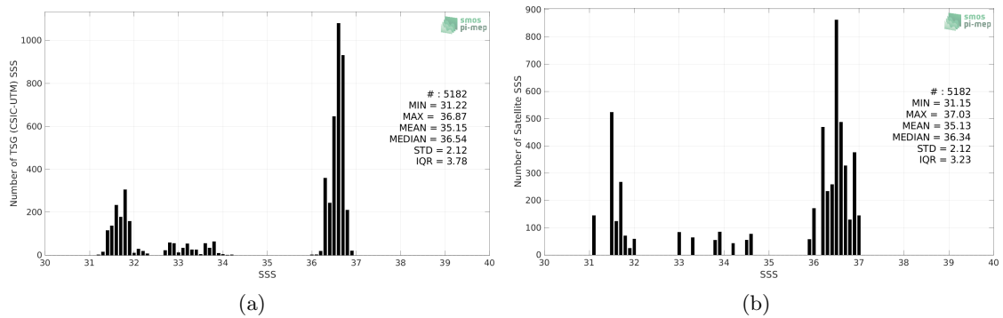
Figure 2: Histograms of SSS from TSG (CSIC-UTM) (a) and SMOS SSS L3 v332 - 9 Days (CATDS-CPDC) (b) considering all match-up pairs per bins of 0.1 over the Gulf Stream Pi-MEP region and for the full satellite product period.
