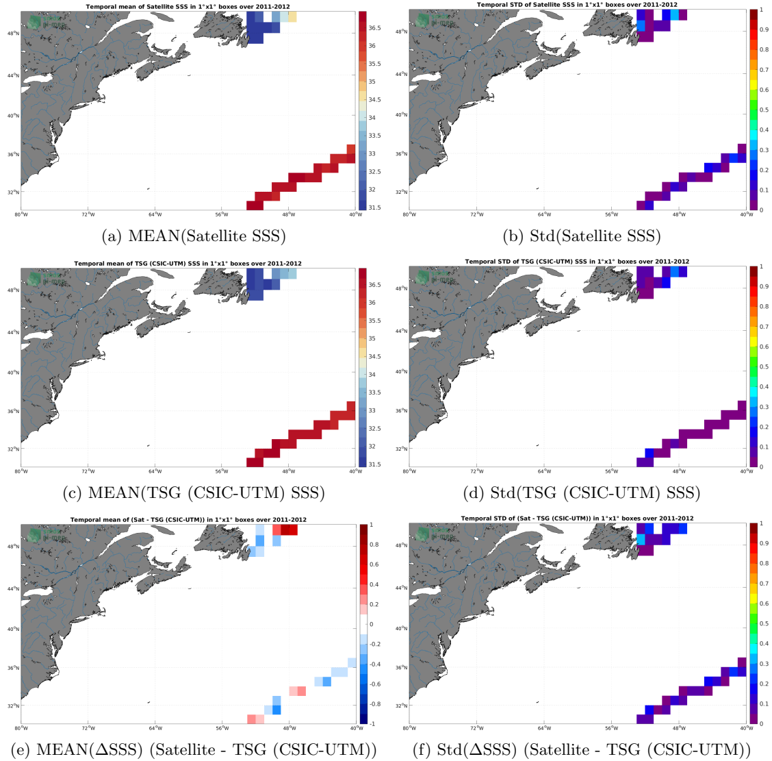
Figure 6: Temporal mean (left) and Std (right) of SSS from SMOS SSS L3 v332 - 9 Days (CATDS-CPDC) (top), TSG (CSIC-UTM) (middle), and of \Delta SSS (Satellite - TSG (CSIC-UTM)). Only match-up pairs are used to generate these maps.
