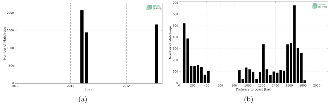
Figure 1: Number of match-ups between TSG (CSIC-UTM) and SMOS SSS L3 v332 - 9 Days (CATDS-CPDC) SSS as a function of time (a) and as function of the distance to coast (b) over the Gulf Stream Pi-MEP region and for the full satellite product period.
