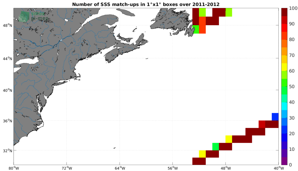
Figure 4: Number of SSS match-ups between TSG (CSIC-UTM) SSS and the SMOS SSS L3 v332 - 9 Days (CATDS-CPDC) SSS product for the Gulf Stream Pi-MEP region over 1^\circ \times 1^\circ boxes and for the full satellite product period.
