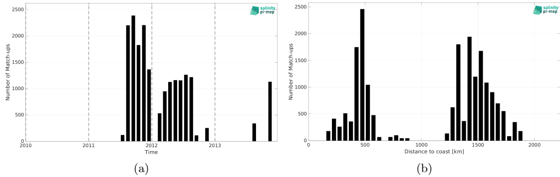
Figure 1: Number of match-ups between Surface drifters and SMOS SSS L3 v332 - 9 Days (CATDS-CPDC) SSS as a function of time (a) and as function of the distance to coast (b) over the Gulf Stream Pi-MEP region and for the full satellite product period.
