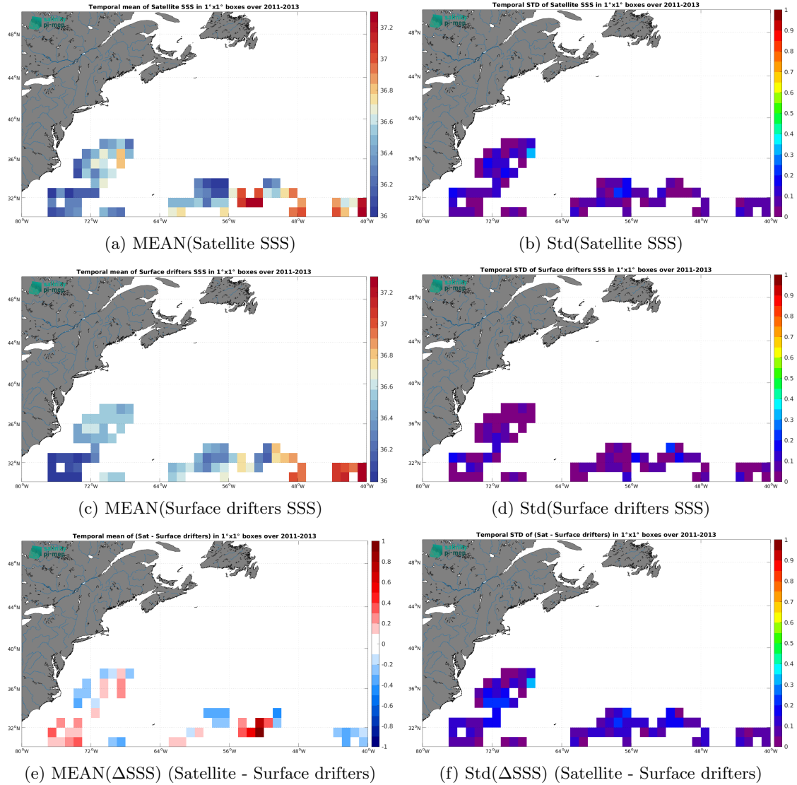
Figure 5: Temporal mean (left) and Std (right) of SSS from SMOS SSS L3 v332 - 9 Days (CATDS-CPDC) (top), Surface drifters (middle), and of \Delta SSS (Satellite - Surface drifters). Only match-up pairs are used to generate these maps.
