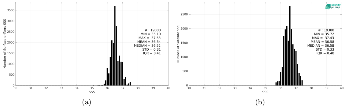
Figure 2: Histograms of SSS from Surface drifters (a) and SMOS SSS L3 v332 - 9 Days (CATDS-CPDC) (b) considering all match-up pairs per bins of 0.1 over the Gulf Stream Pi-MEP region and for the full satellite product period.
