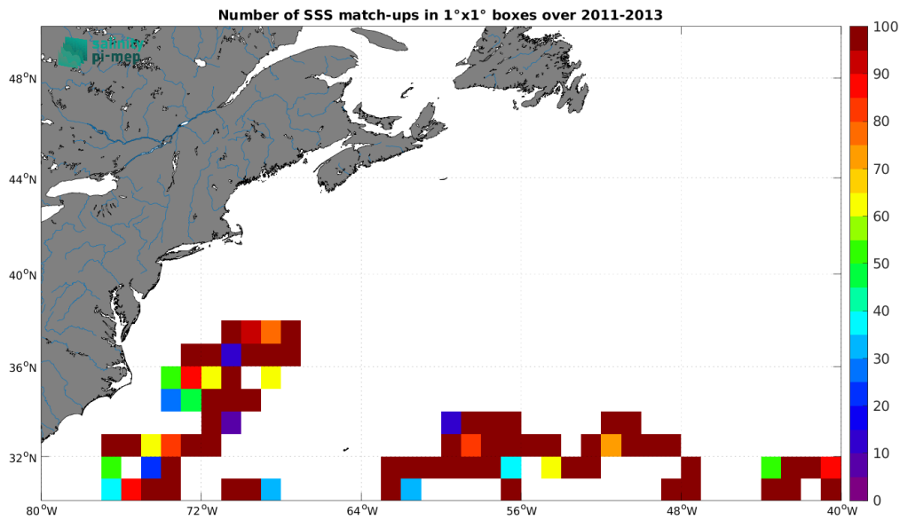
Figure 3: Number of SSS match-ups between Surface drifters SSS and the SMOS SSS L3 v332 - 9 Days (CATDS-CPDC) SSS product for the Gulf Stream Pi-MEP region over 1^\circ \times 1^\circ boxes and for the full satellite product period.
