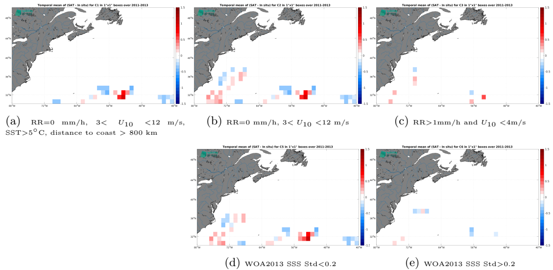
Figure 11: Temporal mean gridded over spatial boxes of size 1^{\circ}\times 1^{\circ} of \Delta\text{SSS} (SMOS SSS L3 v332 - 9 Days (CATDS-CPDC) - Surface drifters) for 5 different subdatasets corresponding to:RR=0 mm/h, 3 < U_{10} < 12 m/s, SST >5^{\circ}\text{C} , distance to coast > 800 km (a), RR=0 mm/h, 3 < U_{10} < 12 m/s (b), RR >1 mm/h and U_{10} < 4 m/s (c), WOA2013 SSS Std <0.2 (d), WOA2013 SSS Std >0.2 (e).
