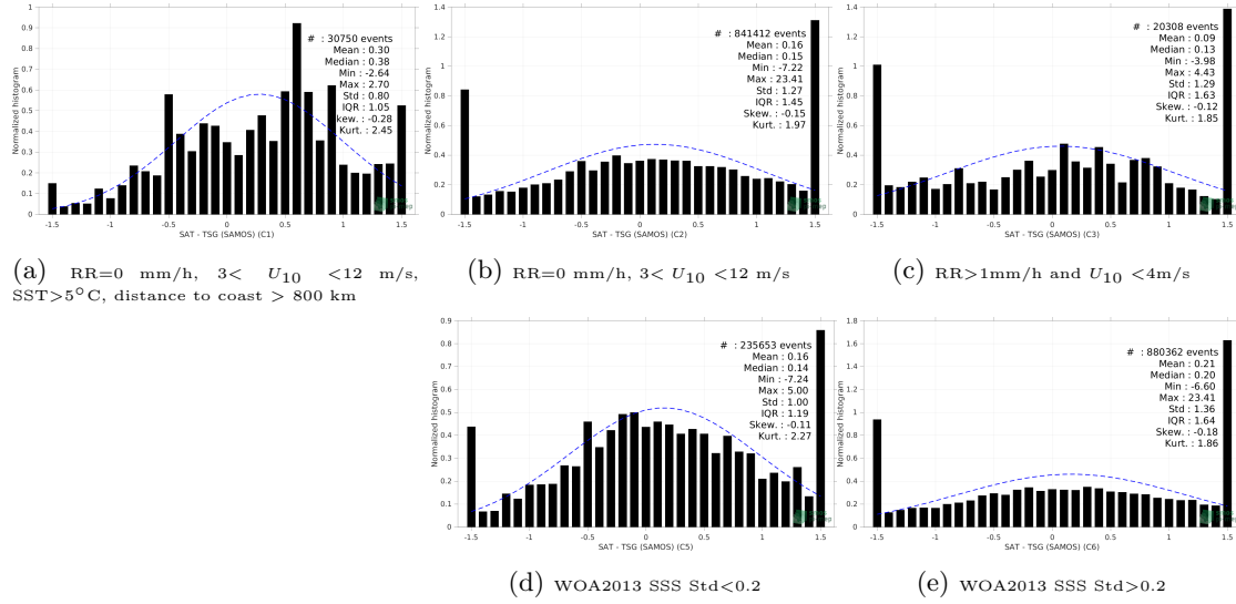
Figure 13: Normalized histogram of \Delta SSS (SMOS SSS L2Q v331 - 0.25 Deg (CATDS-CPDC) - TSG (SAMOS)) for 5 different subdatasets corresponding to: RR=0 mm/h, 3 < U_{10} < 12 m/s, SST > 5°C, distance to coast > 800 km (a), RR=0 mm/h, 3 < U_{10} < 12 m/s (b), RR > 1mm/h and U_{10} < 4 m/s (c), WOA2013 SSS Std < 0.2 (d), WOA2013 SSS Std > 0.2 (e).
