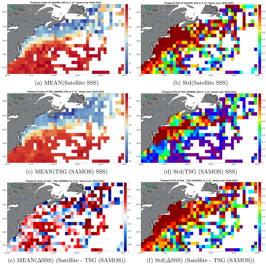
Figure 6: Temporal mean (left) and Std (right) of SSS from SMOS SSS L2Q v331 - 0.25 Deg (CATDS-CPDC) (top), TSG (SAMOS) (middle), and of \Delta SSS (Satellite - TSG (SAMOS)). Only match-up pairs are used to generate these maps.
