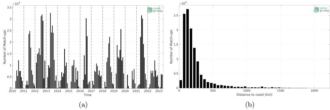
Figure 1: Number of match-ups between TSG (SAMOS) and SMOS SSS L2Q v331 - 0.25 Deg (CATDS-CPDC) SSS as a function of time (a) and as function of the distance to coast (b) over the Gulf Stream Pi-MEP region and for the full satellite product period.
