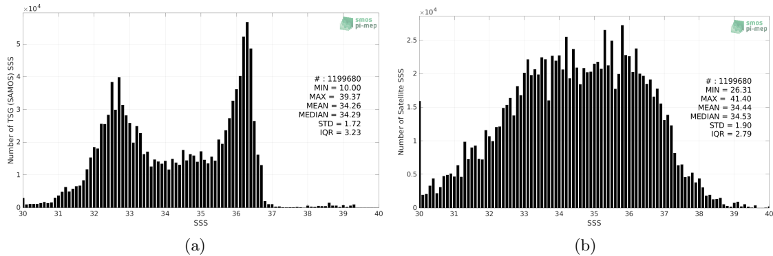
Figure 2: Histograms of SSS from TSG (SAMOS) (a) and SMOS SSS L2Q v331 - 0.25 Deg (CATDS-CPDC) (b) considering all match-up pairs per bins of 0.1 over the Gulf Stream Pi-MEP region and for the full satellite product period.
