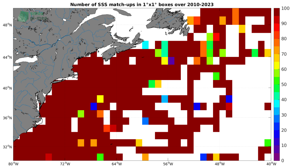
Figure 4: Number of SSS match-ups between TSG (SAMOS) SSS and the SMOS SSS L2Q v331 - 0.25 Deg (CATDS-CPDC) SSS product for the Gulf Stream Pi-MEP region over 1^\circ \times 1^\circ boxes and for the full satellite product period.
