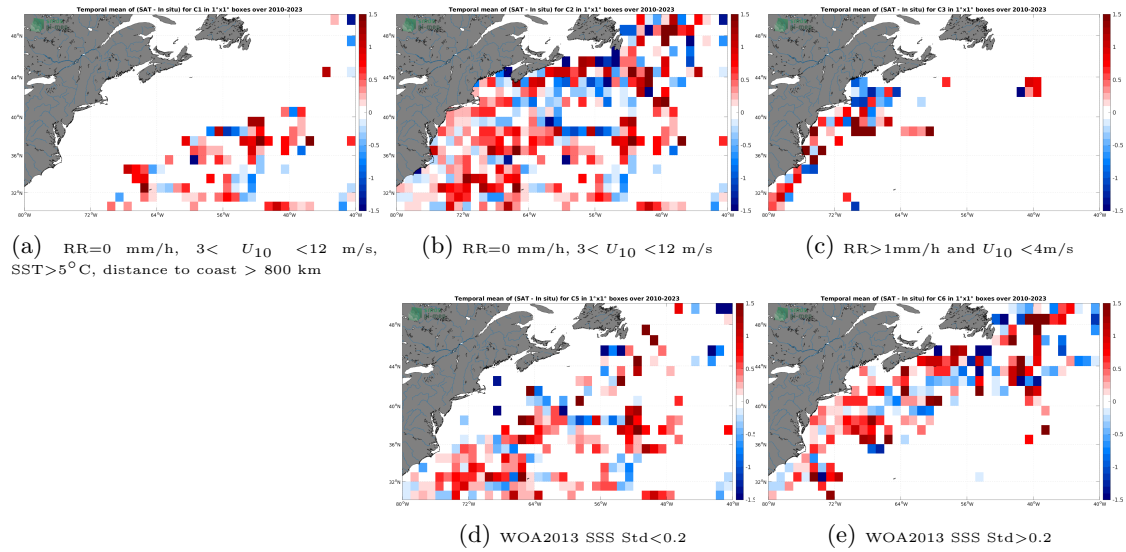
Figure 12: Temporal mean gridded over spatial boxes of size 1^\circ \times 1^\circ of \Delta SSS (SMOS SSS L2Q v331 - 0.25 Deg (CATDS-CPDC) - TSG (SAMOS)) for 5 different subdatasets corresponding to:RR=0 mm/h, 3 < U_{10} < 12 m/s, SST >5^\circ C, distance to coast > 800 km (a), RR=0 mm/h, 3 < U_{10} < 12 m/s (b), RR >1 mm/h and U_{10} < 4 m/s (c), WOA2013 SSS Std <0.2 (d), WOA2013 SSS Std >0.2 (e).
