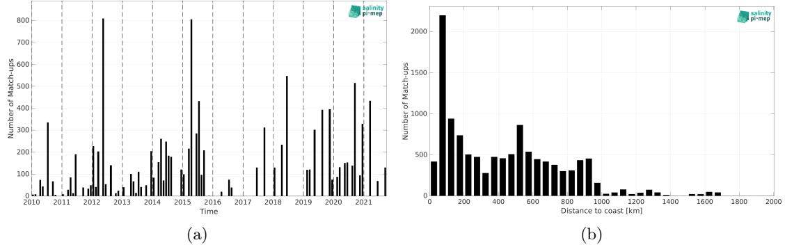
Figure 1: Number of match-ups between TSG (LEGOS-DM) and SMOS SSS L2Q v331 - 0.25 Deg (CATDS-CPDC) SSS as a function of time (a) and as function of the distance to coast (b) over the Gulf Stream Pi-MEP region and for the full satellite product period.
