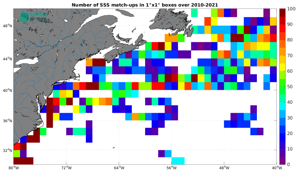
Figure 4: Number of SSS match-ups between TSG (LEGOS-DM) SSS and the SMOS SSS L2Q v331 - 0.25 Deg (CATDS-CPDC) SSS product for the Gulf Stream Pi-MEP region over 1^\circ \times 1^\circ boxes and for the full satellite product period.
