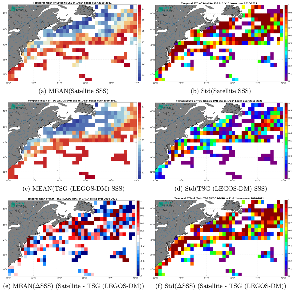
Figure 6: Temporal mean (left) and Std (right) of SSS from SMOS SSS L2Q v331 - 0.25 Deg (CATDS-CPDC) (top), TSG (LEGOS-DM) (middle), and of \Delta SSS (Satellite - TSG (LEGOS-DM)). Only match-up pairs are used to generate these maps.
