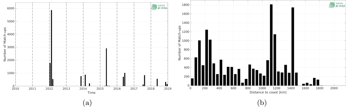
Figure 1: Number of match-ups between TSG (GOSUD-Sailing-ship) and SMOS SSS L2Q v331 - 0.25 Deg (CATDS-CPDC) SSS as a function of time (a) and as function of the distance to coast (b) over the Gulf Stream Pi-MEP region and for the full satellite product period.
