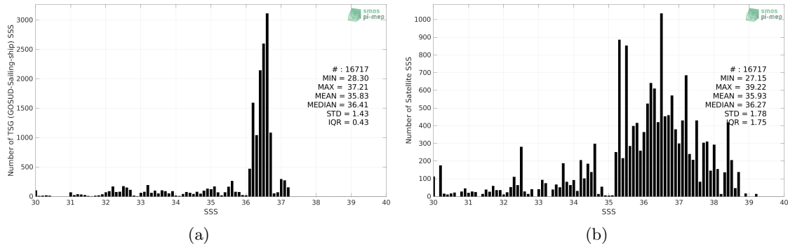
Figure 2: Histograms of SSS from TSG (GOSUD-Sailing-ship) (a) and SMOS SSS L2Q v331 - 0.25 Deg (CATDS-CPDC) (b) considering all match-up pairs per bins of 0.1 over the Gulf Stream Pi-MEP region and for the full satellite product period.
