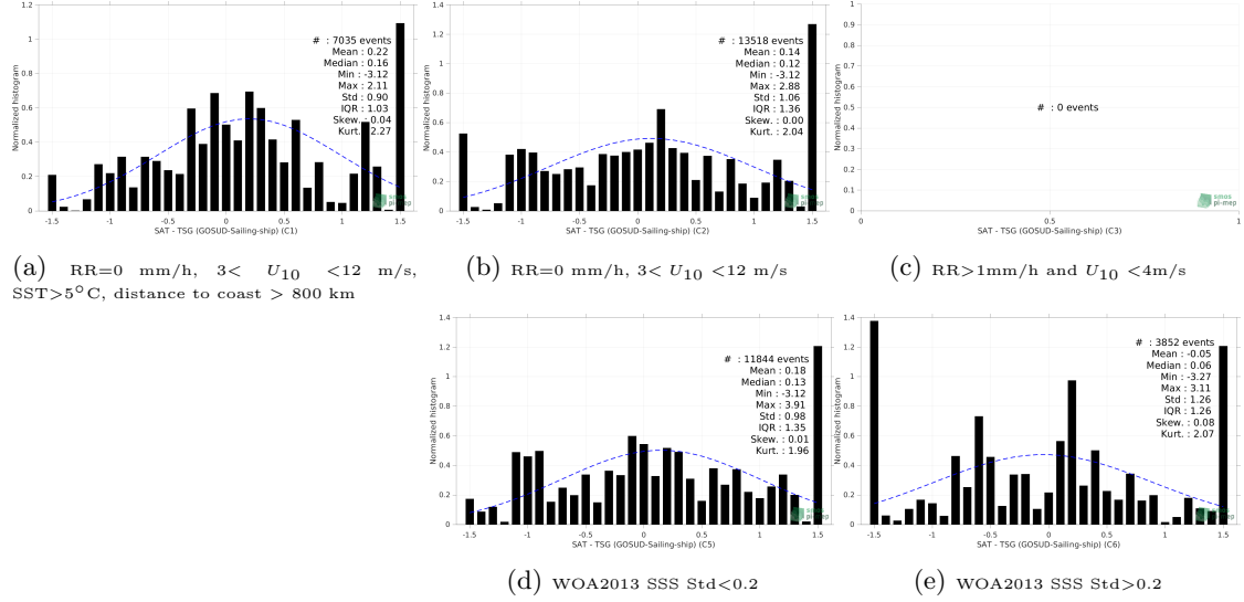
Figure 13: Normalized histogram of \Delta SSS (SMOS SSS L2Q v331 - 0.25 Deg (CATDS-CPDC) - TSG (GOSUD-Sailing-ship)) for 5 different subdatasets corresponding to: RR=0 mm/h, 3 < U_{10} < 12 m/s, SST > 5°C, distance to coast > 800 km (a), RR=0 mm/h, 3 < U_{10} < 12 m/s (b), RR > 1mm/h and U_{10} < 4 m/s (c), WOA2013 SSS Std < 0.2 (d), WOA2013 SSS Std > 0.2 (e).
