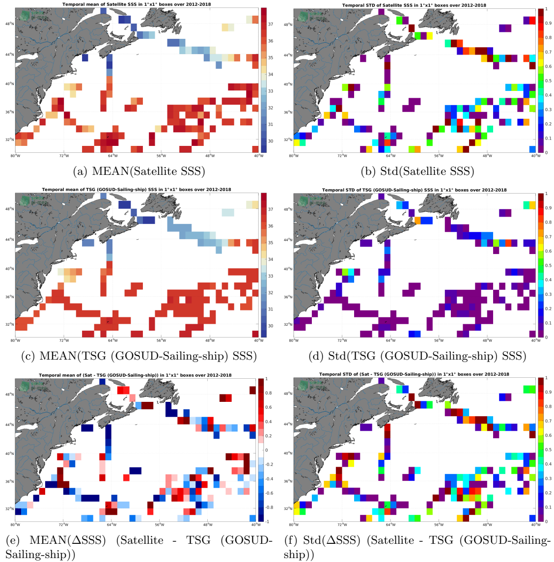
Figure 6: Temporal mean (left) and Std (right) of SSS from SMOS SSS L2Q v331 - 0.25 Deg (CATDS-CPDC) (top), TSG (GOSUD-Sailing-ship) (middle), and of \Delta SSS (Satellite - TSG (GOSUD-Sailing-ship)). Only match-up pairs are used to generate these maps.
