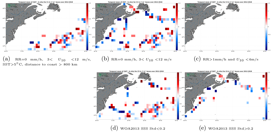
Figure 12: Temporal mean gridded over spatial boxes of size 1^{\circ}\times 1^{\circ} of \Delta SSS (SMOS SSS L2Q v331 - 0.25 Deg (CATDS-CPDC) - TSG (GOSUD-Sailing-ship)) for 5 different subdatasets corresponding to: RR=0 mm/h, 3 < U_{10} < 12 m/s, SST > 5^{\circ}\text{C} , distance to coast > 800 km (a), RR=0 mm/h, 3 < U_{10} < 12 m/s (b), RR > 1 mm/h and U_{10} < 4 m/s (c), WOA2013 SSS Std < 0.2 (d), WOA2013 SSS Std > 0.2 (e).
