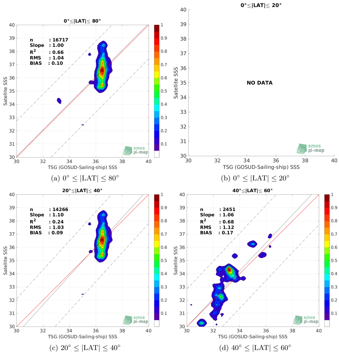
Figure 9: Contour maps of the concentration of SMOS SSS L2Q v331 - 0.25 Deg (CATDS-CPDC) SSS (y-axis) versus TSG (GOSUD-Sailing-ship) SSS (x-axis) at match-up pairs for different latitude bands. For each plot, the red line shows x=y . The black thin and dashed lines indicate a linear fit through the data cloud and the \pm 95\% confidence levels, respectively. The number of match-up pairs n , the slope and R^2 coefficient of the linear fit, the root mean square (RMS) and the mean bias between satellite and in situ data are indicated for each latitude band in each plot.
