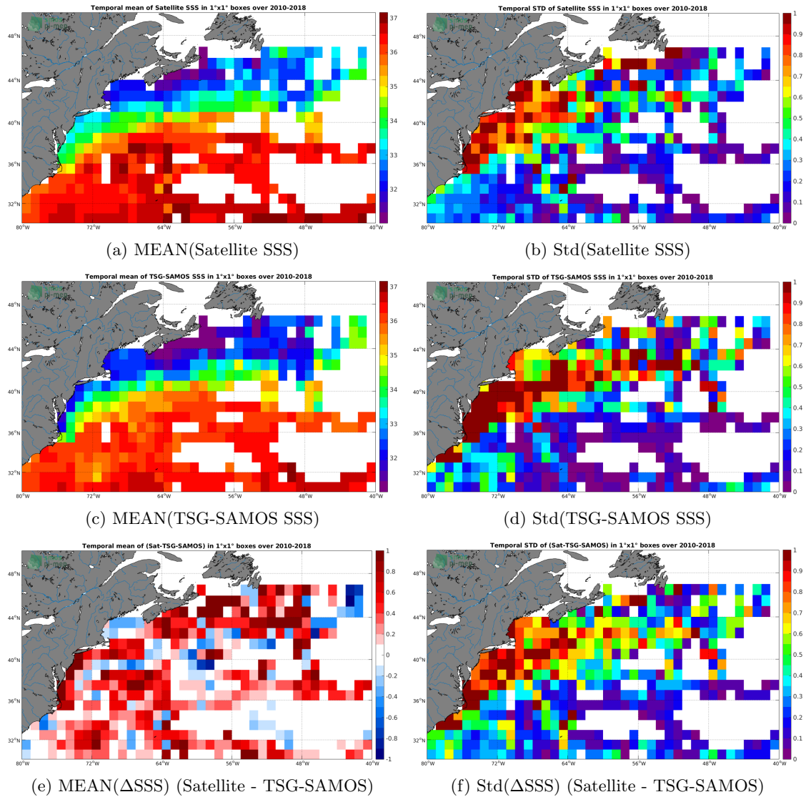
Figure 6: Temporal mean (left) and Std (right) of SSS from SMOS-L3-CATDS-CPDC-V3-10DAYS-25KM (top), TSG-SAMOS (middle), and of \Delta SSS (Satellite - TSG-SAMOS). Only match-up pairs are used to generate these maps.
