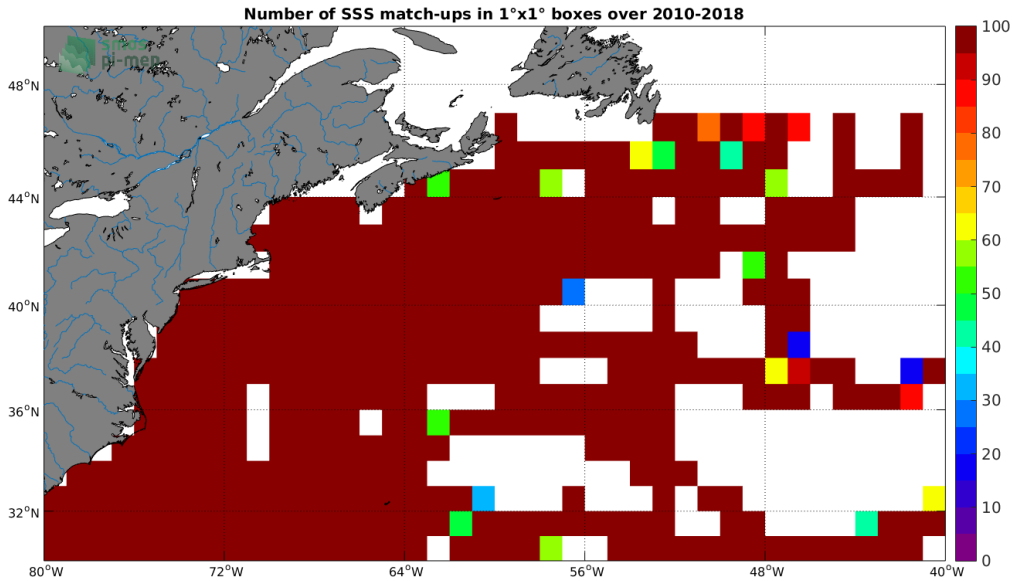
Figure 4: Number of SSS match-ups between TSG-SAMOS SSS and the SMOS-L3-CATDS-CPDC-V3-10DAYS-25KM SSS product for the Gulf Stream Pi-MEP region over 1^\circ \times 1^\circ boxes and for the full satellite product period.
