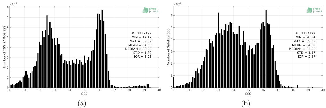
Figure 2: Histograms of SSS from TSG-SAMOS (a) and SMOS-L3-CATDS-CPDC-V3-10DAYS-25KM (b) considering all match-up pairs per bins of 0.1 over the Gulf Stream Pi-MEP region and for the full satellite product period.
