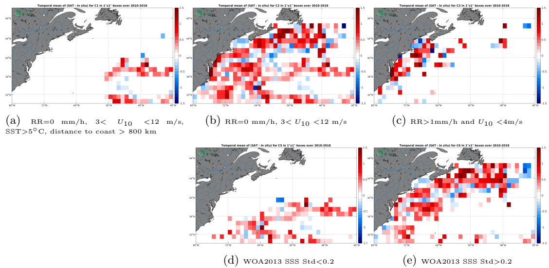
Figure 12: Temporal mean gridded over spatial boxes of size 1^\circ \times 1^\circ of \Delta SSS (SMOS-L3-CATDS-CPDC-V3-10DAYS-25KM - TSG-SAMOS) for 5 different subdatasets corresponding to:RR=0 mm/h, 3 < U_{10} < 12 m/s, SST >5^\circ C, distance to coast > 800 km (a), RR=0 mm/h, 3 < U_{10} < 12 m/s (b), RR >1 mm/h and U_{10} < 4 m/s (c), WOA2013 SSS Std <0.2 (d), WOA2013 SSS Std >0.2 (e).
