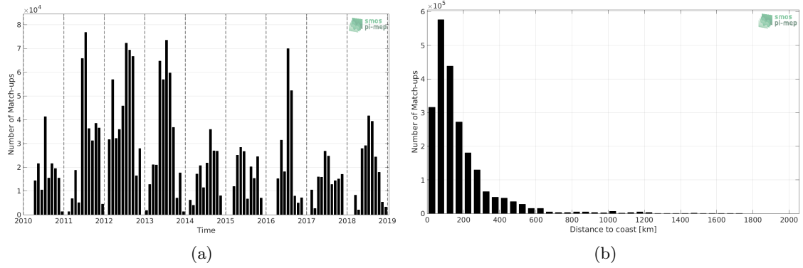
Figure 1: Number of match-ups between TSG-SAMOS and SMOS-L3-CATDS-CPDC-V3-10DAYS-25KM SSS as a function of time (a) and as function of the distance to coast (b) over the Gulf Stream Pi-MEP region and for the full satellite product period.
