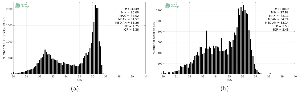
Figure 2: Histograms of SSS from TSG-LEGOS-DM (a) and SMOS-L3-CATDS-CPDC-V3-10DAYS-25KM (b) considering all match-up pairs per bins of 0.1 over the Gulf Stream Pi-MEP region and for the full satellite product period.
