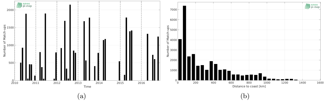
Figure 1: Number of match-ups between TSG-LEGOS-DM and SMOS-L3-CATDS-CPDC-V3-10DAYS-25KM SSS as a function of time (a) and as function of the distance to coast (b) over the Gulf Stream Pi-MEP region and for the full satellite product period.
