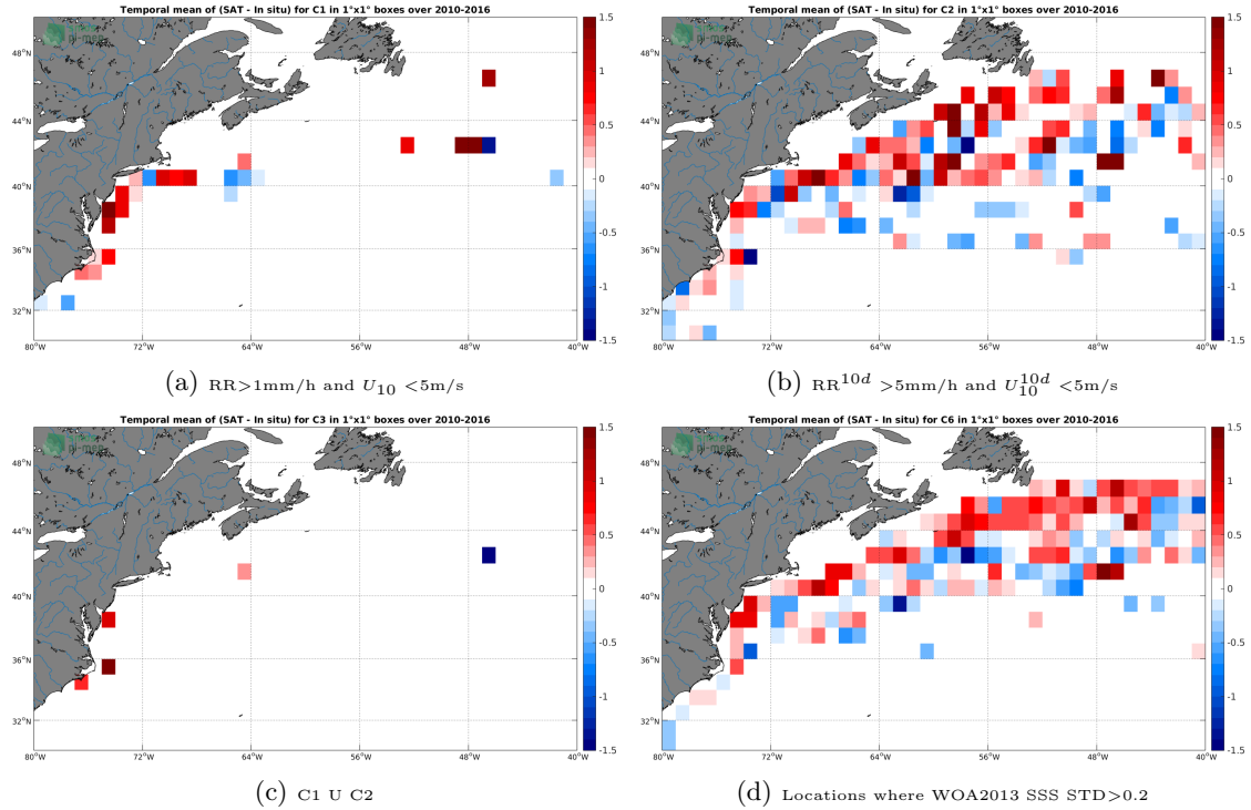
Figure 12: Temporal mean gridded over spatial boxes of size 1^\circ \times 1^\circ of \Delta SSS (SMOS-L3-CATDS-CPDC-V3-10DAYS-25KM - TSG-LEGOS-DM) for 4 different subdatasets corresponding to: RR > 1mm/h and U_{10} < 5 m/s (a), RR^{10d} > 5 mm/h and U_{10}^{10d} < 5 m/s (b), C1 U C2 (c), Locations where WOA2013 SSS STD > 0.2 (d).
