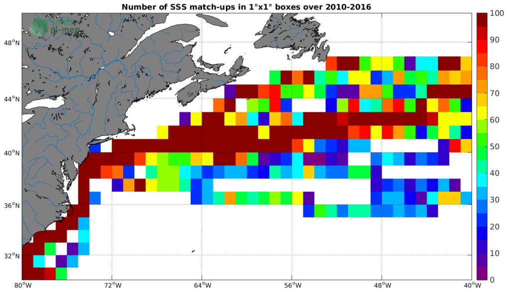
Figure 4: Number of SSS match-ups between TSG-LEGOS-DM SSS and the SMOS-L3-CATDS-CPDC-V3-10DAYS-25KM SSS product for the Gulf Stream Pi-MEP region over 1^\circ \times 1^\circ boxes and for the full satellite product period.
